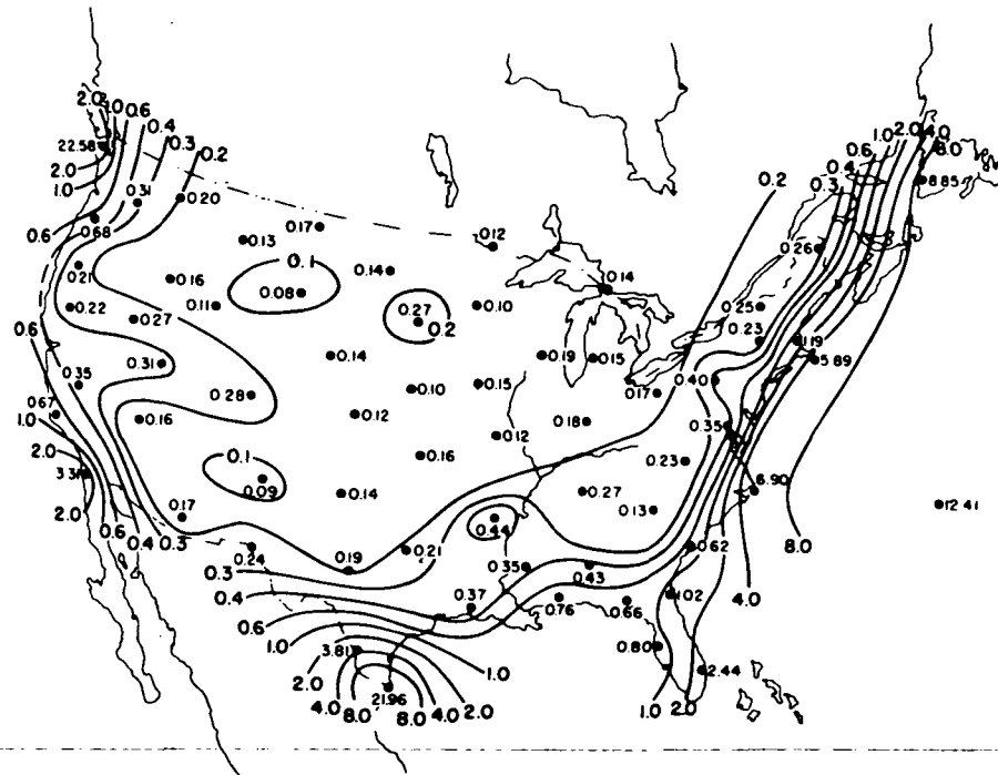
Source: Junge and Werby (1958) Average \text{Cl}^- concentration (milligrams per liter) in rain over the United States from July 1955 to June 1956. FIGURE VII-6 CHLORIDE IN PRECIPITATION OVER THE UNITED STATES
