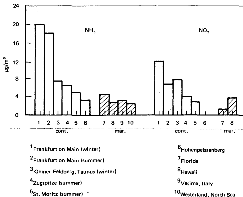
FIGURE VI-9 CONCENTRATION OF \text{NH}_3 AND \text{NO}_2 IN AIR AT DIFFERENT CONTINENTAL AND MARITIME LOCATIONS
