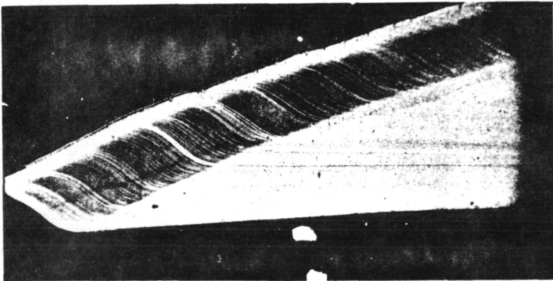
(2) Unio raveneliensis . Recent, Nicaragua. Radial thin section. Plane polarized light. X38.
