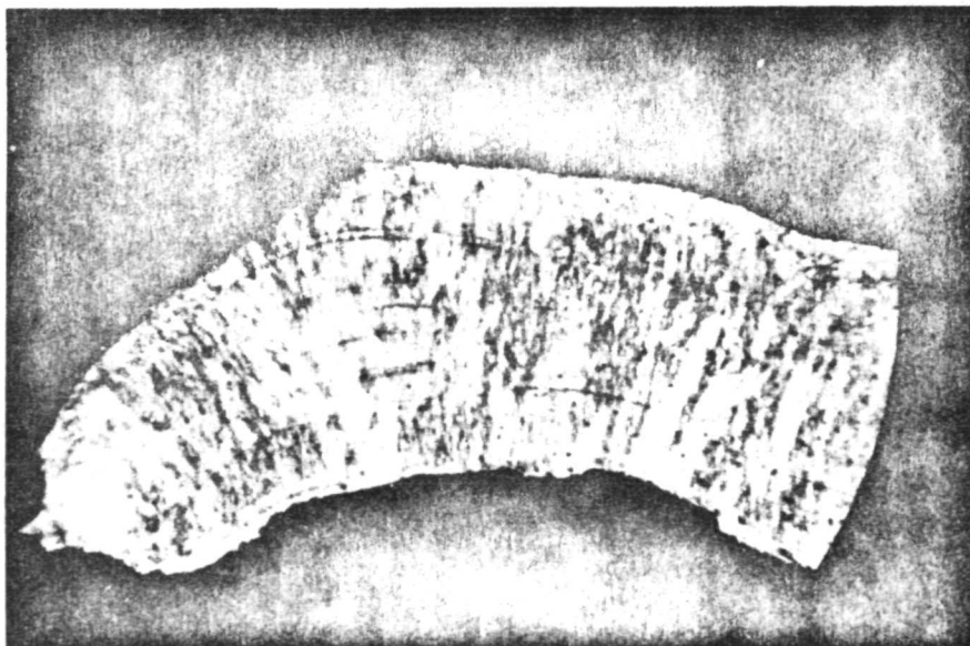
(2) Spondylus crassiguama Lamarck . Cross section of calcareous spine. Thin section normal to long axis of spine, near distal end of spine. Recent, Gulf of California. Crossed Nichols X25.
