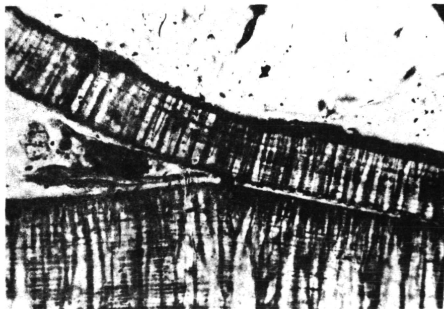
(2) Minor growth band on surface of shell in upper right corner of (1). Plane polarized light X160.
