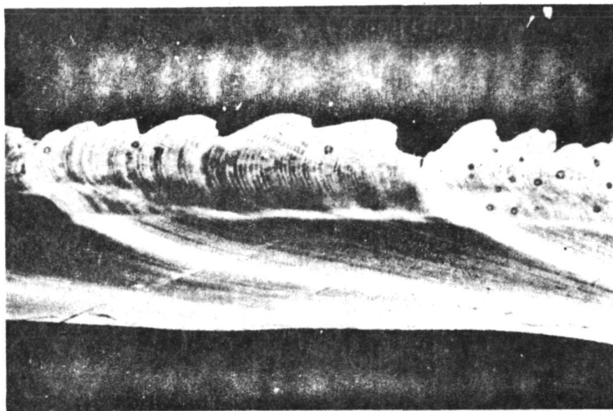
(1) Two slow-growth groove deposits appear as brightly illuminated growth layers X29.
