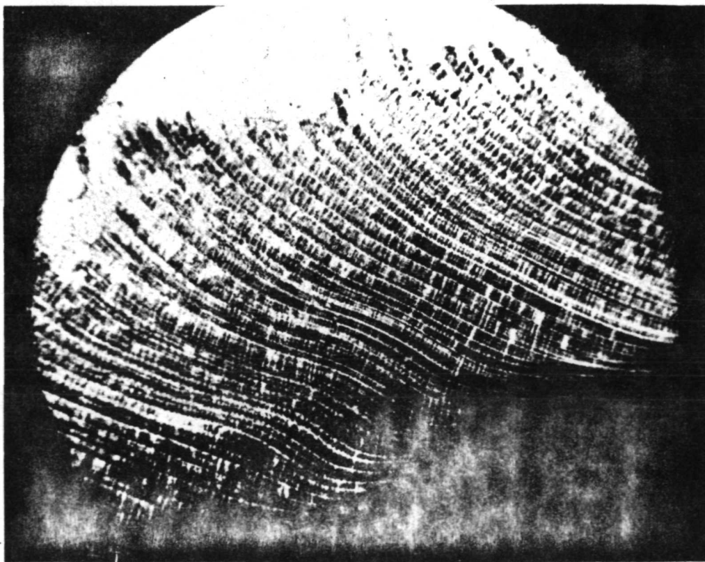
Plate 8:2. Mercenaria mercenaria (Linnaeus). Concentric ridges and troughs in thin section of pigmented shell. Recent, Bradenton, Florida. Plane polarized light X64.
