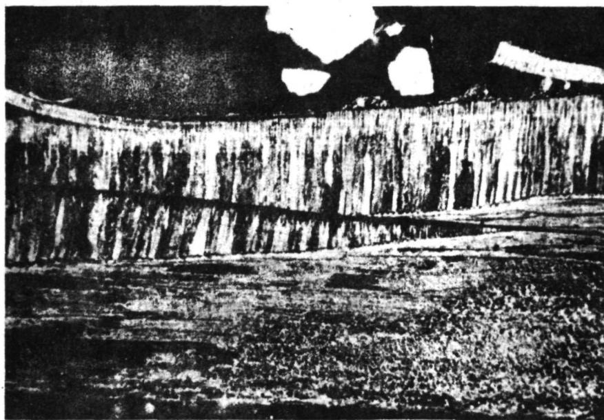
(1) Imbrication of prismatic and nacreous layers. Crossed Nichols X24.
