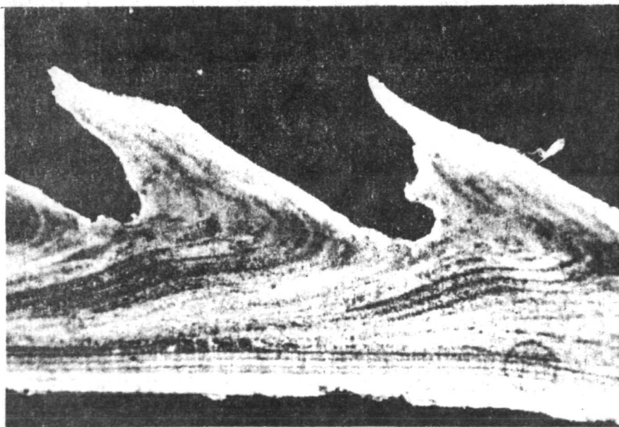
(2) Zirfaea gabbi Lowe . Protrusive ridges in radial thin section. Recent, San Francisco Beach, California. Crossed Nichols X59.
