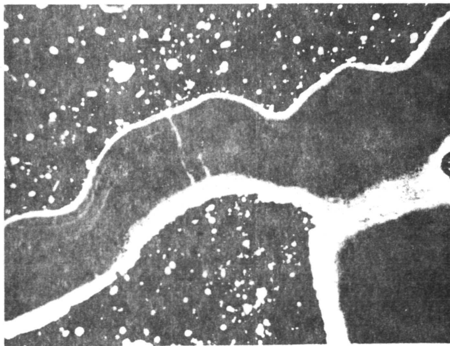
(2) Horizontal thin section of ridge on ventral margin. Crossed Nichols X87.
