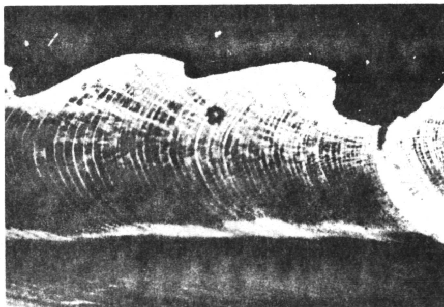
(2) Enlargement, concentric ridges shown at lower magnification in (1)X73.
