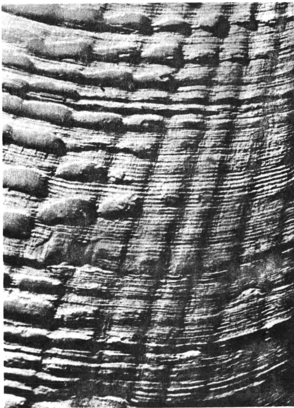
Plate 11. Protothaca fructifraga (Sowerby). Growth laminae forming concentric ridges and troughs on etched surface. Recent, Cholla Bay, Sonora, Mexico X13.
