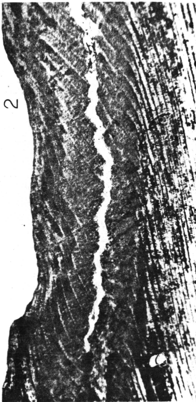
(2) Growth laminae and two concentric ridges X117.
