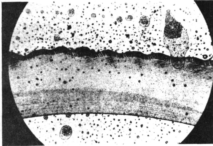
(1) Eucrassatella digueti Lamarck . Radial thin section of ventral portion of shell. Recent, Gulf of California. Crossed Nichols - X38.
