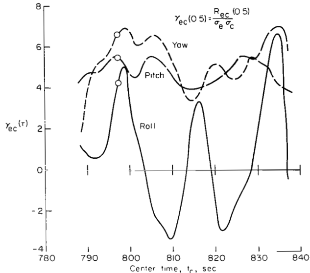
Figure 18.— Variation of the normalized cross-covariance function for each axis during the TPI maneuver.
