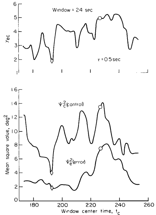
Figure 10.— Comparison of variation of \gamma_{ec} with mean squared values of signals.
