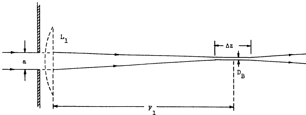
Focal Tolerance in Transmission Optics (see Figure 18)
