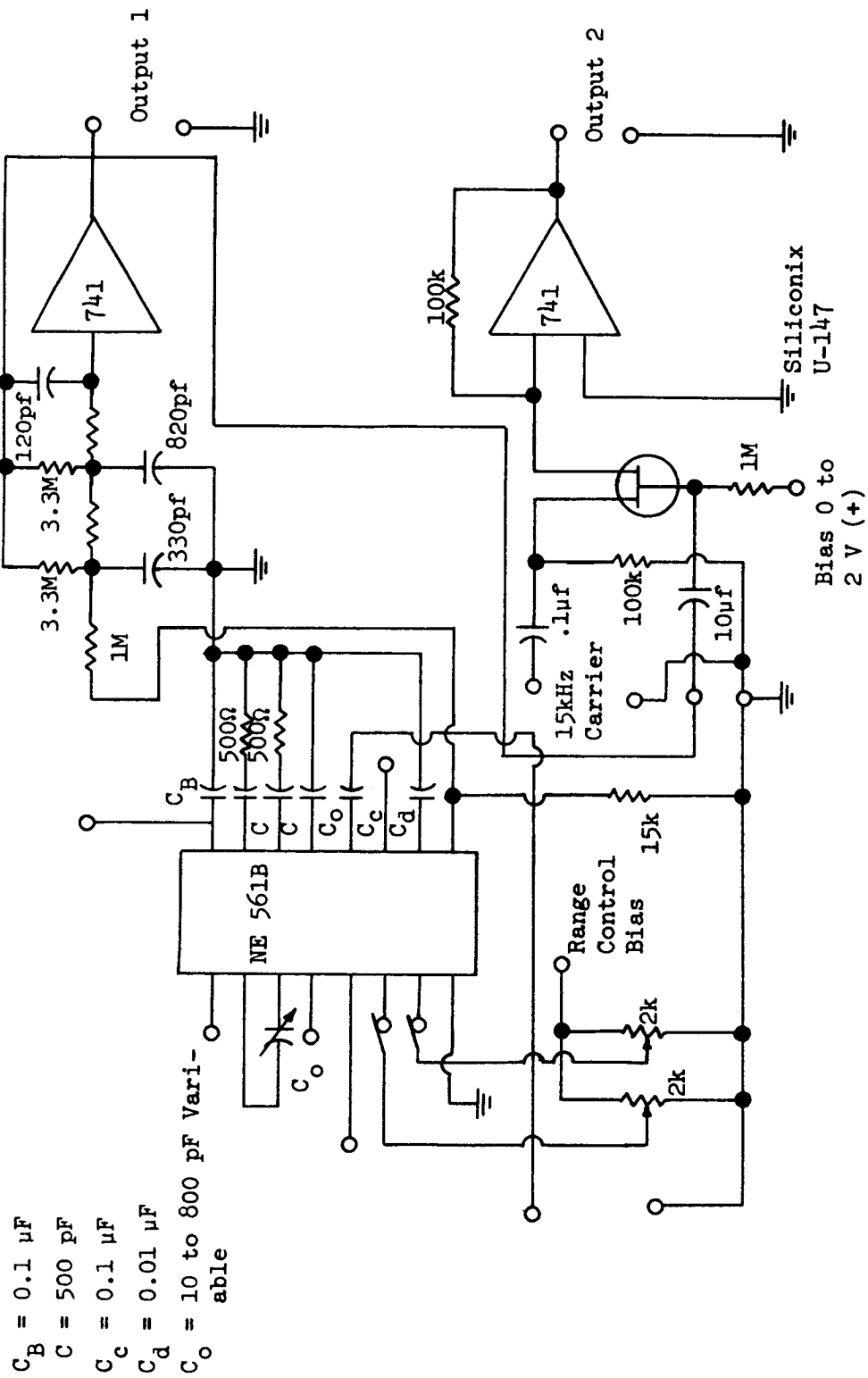
Figure 48 Circuit Diagram of the Phase-Locked Loop Detector
