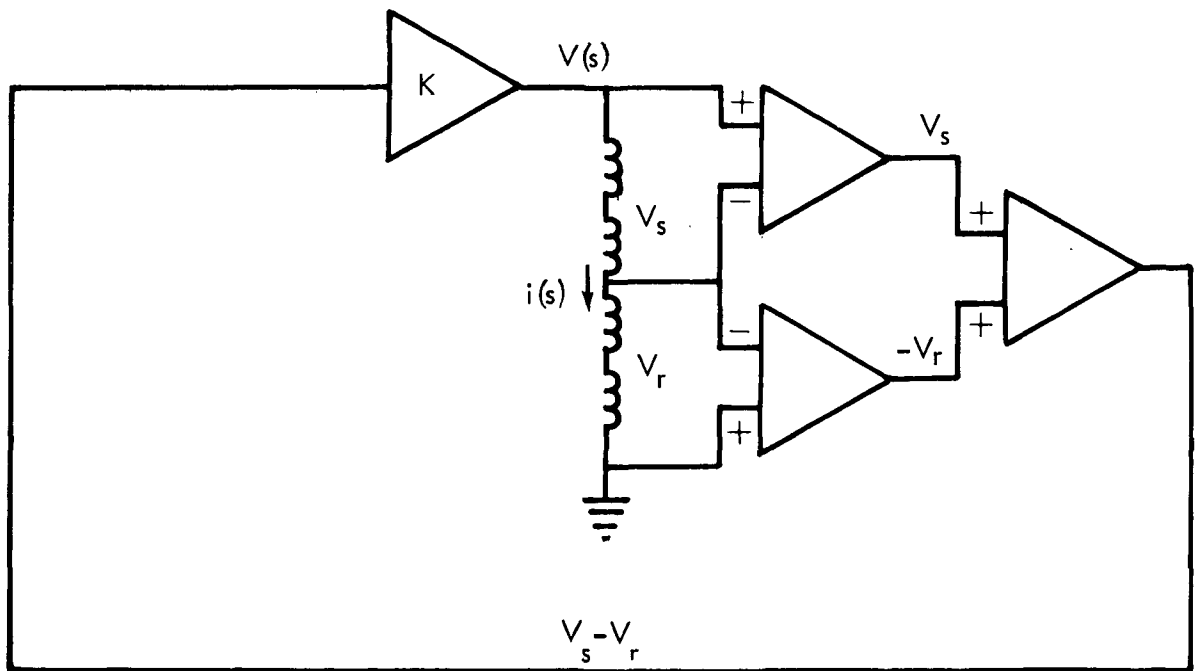
Figure 9.3-2. Elimination of Velocity Pickup Coil
