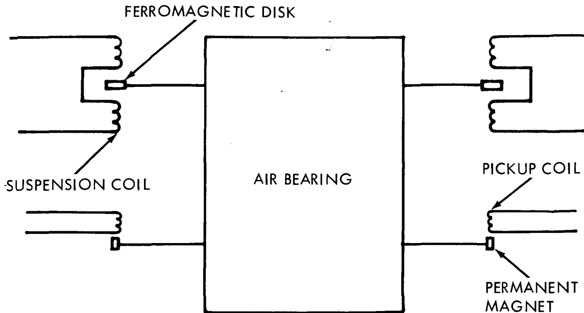
Figure 4.1-2. Suspension Geometry
