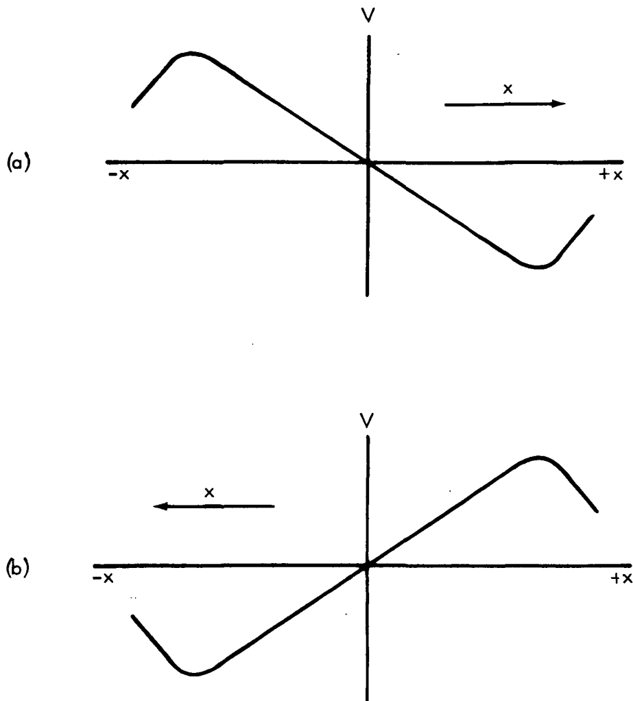
Figure 4.2-1. Output Voltage of Velocity Sensing Coils
