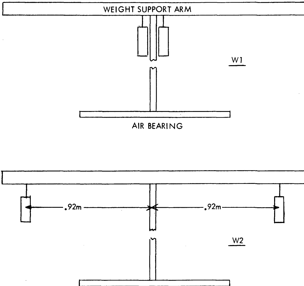
Figure 7.3-1 Weight Configurations
