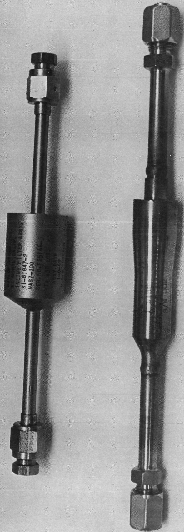
Figure 11: VACCO FILTER (LEFT) AND JPL FILTER (RIGHT)
