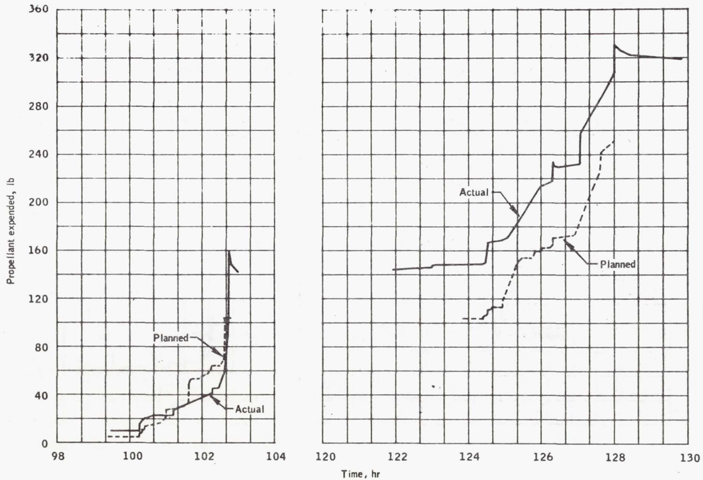
Figure 9.- Comparison of predicted and actual propellant consumption.
