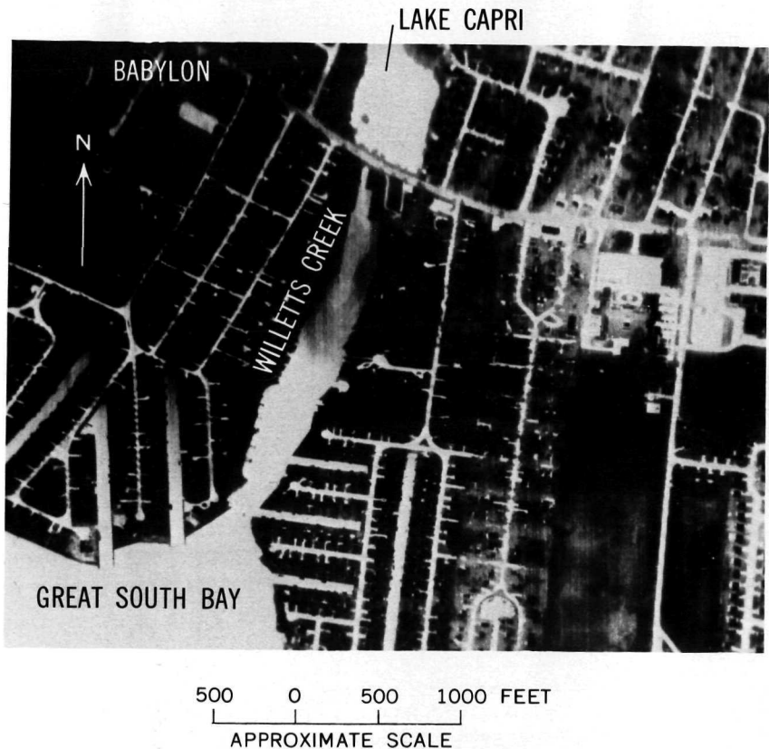
FIGURE 10.—Imagery obtained June 17, 1969, of the lower reaches of Willetts Creek, showing ground-water seepage into the creek. (Imagery from RADC.)
