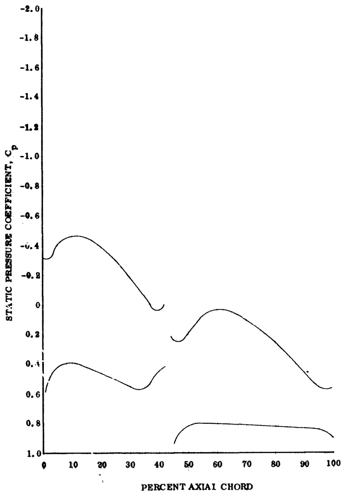
Figure 47. Rotor C Static Pressure Coefficient, 75% Span From Tip
