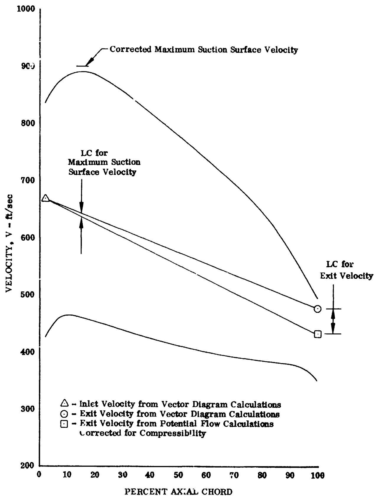
Figure 24. Stator A Vane Surface Velocities, 95% Span From Tip
