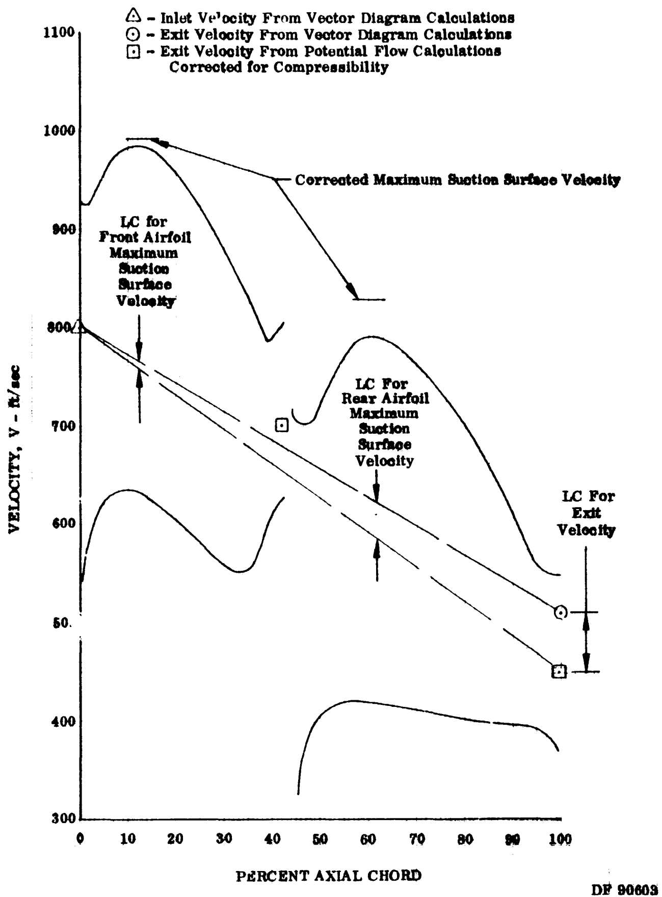
Figure 48. Rotor C Blade Surface Velocities, 75% Span From Tip
