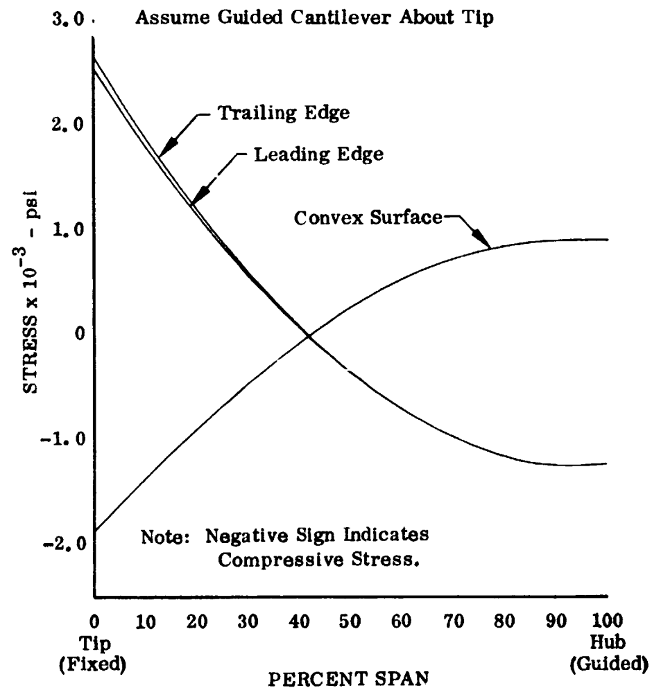
Figure 73. Calculated Stator A Stress Distribution
