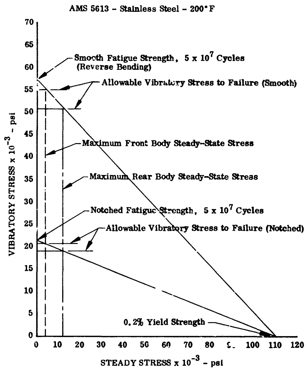
Figure 78. Soderberg Goodman Diagram
