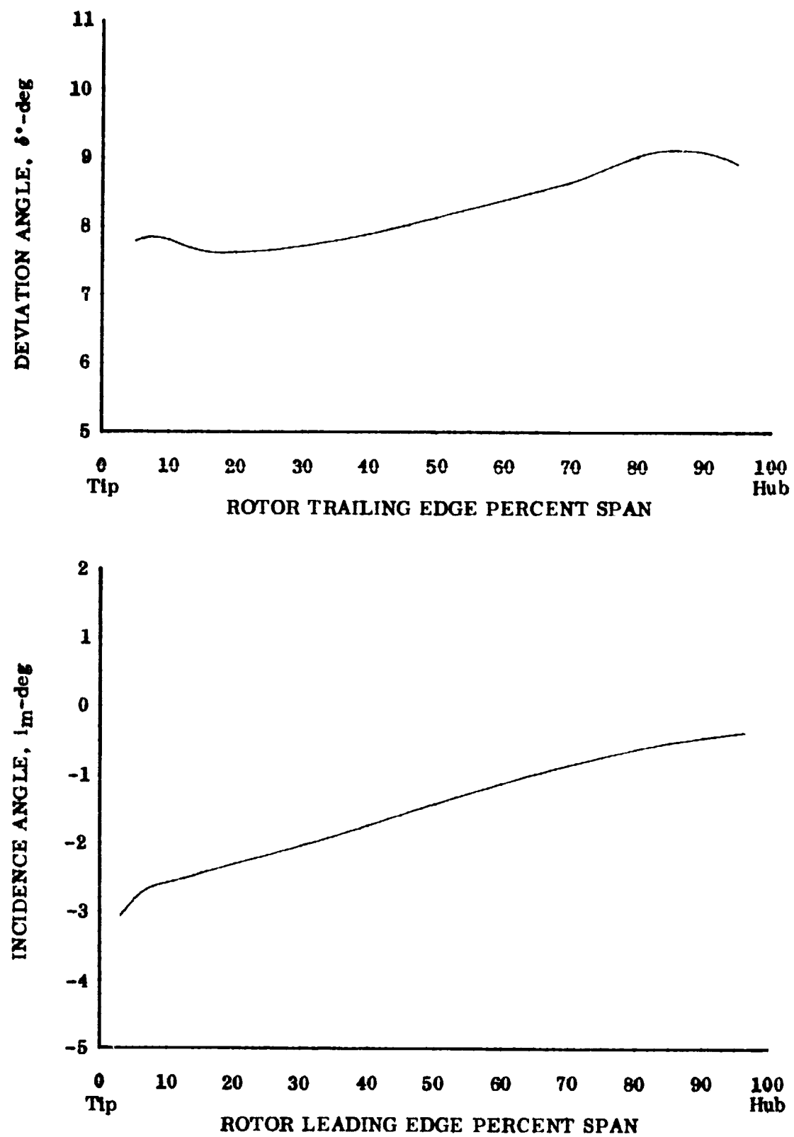
Figure 11. Rotor Incidence and Deviation Angle
