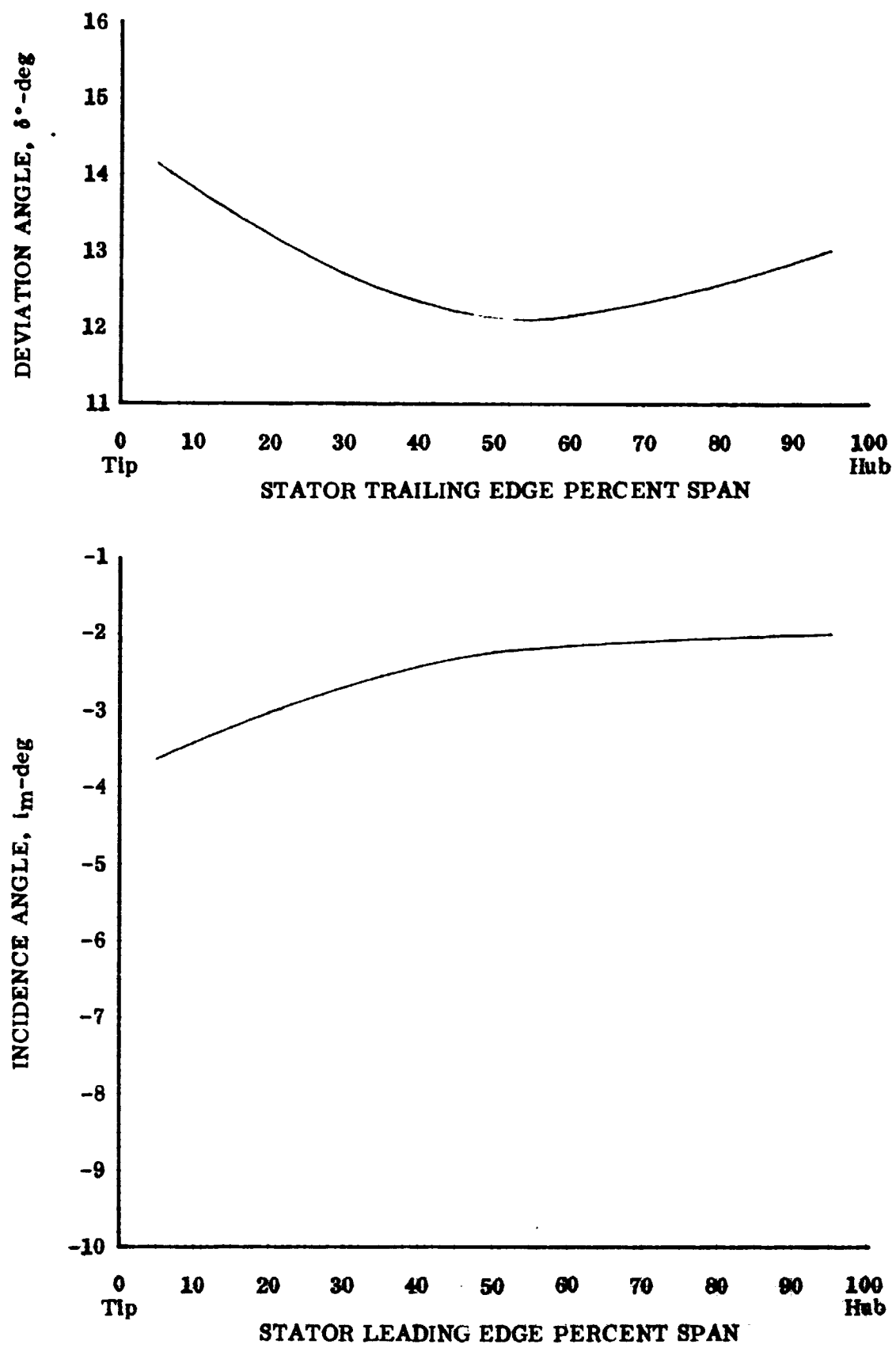
Figure 13. Stator Incidence and Deviation Angle
