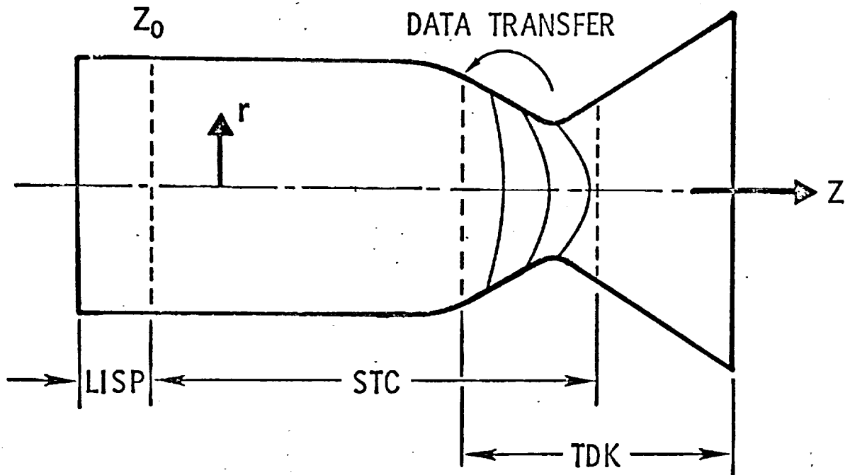
Figure 15. Distributed Energy Release Revised STC/TDK Interface
