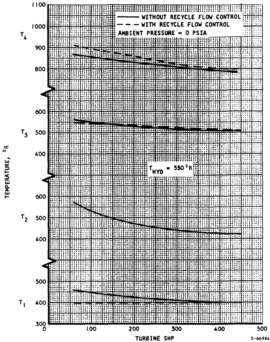
Figure 5-5. Comparison of Hydrogen Loop Performance with and without Recycle Flow Control at 75°R Hydrogen Inlet Temperature
