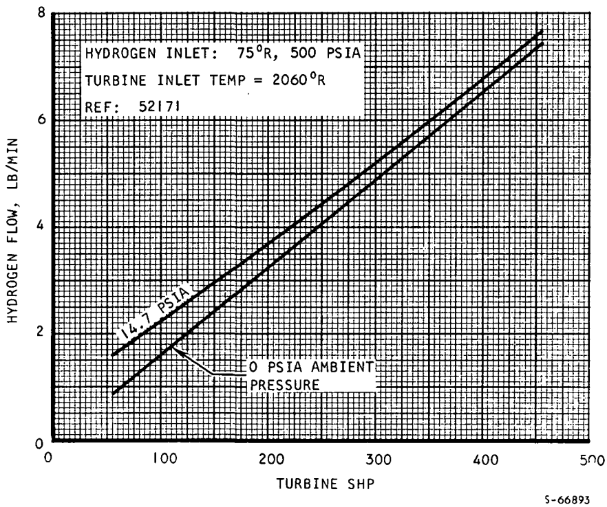
Figure 2-2. Typical Hydrogen Flow Characteristics
