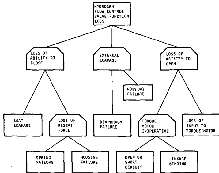
HYDROGEN FLOW CONTROL VALVE
