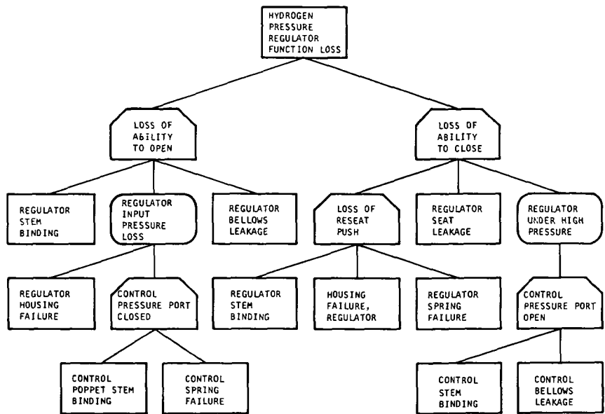
HYDROGEN PRESSURE REGULATOR
