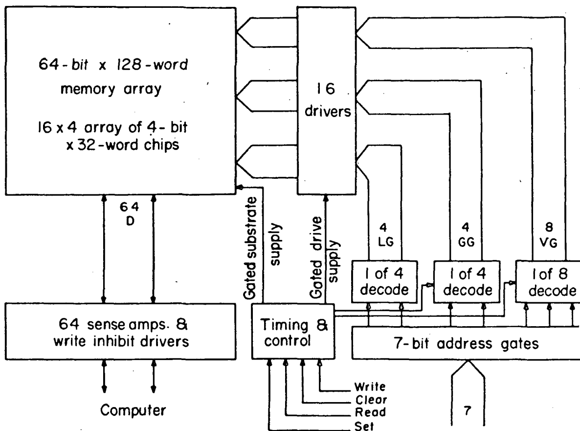
FIG. 11 Block diagram of control memory.
