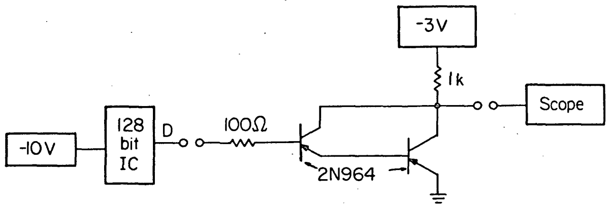
FIG. 8a Schematic of sense amplifier.
