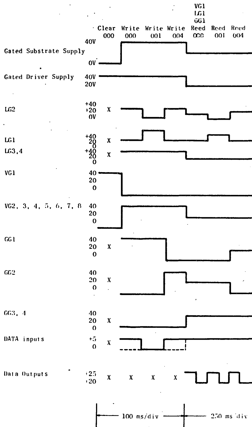
FIG. 16 Timing signals.
