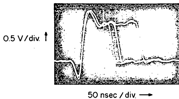
FIG. 22 "D" - line output after comparator.
