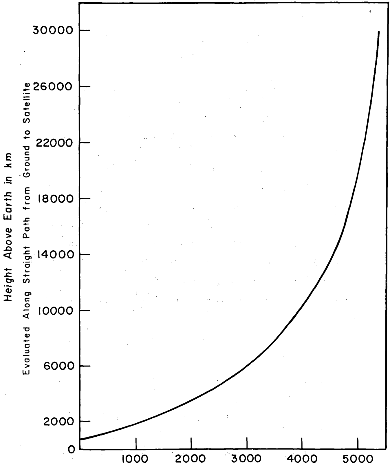
Z , (Temperature Modified Geopotential Height) in km. Evaluated Along Straight Path from Ground to Satellite
