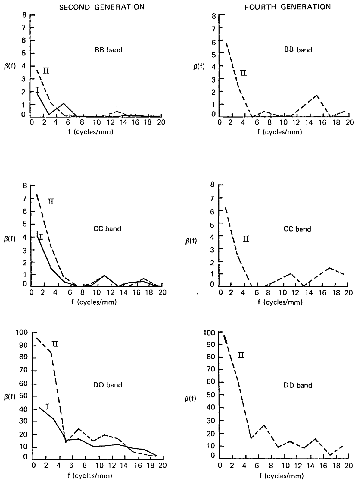
Fig. 16. Signal-to-noise ratios for second and fourth generations.
