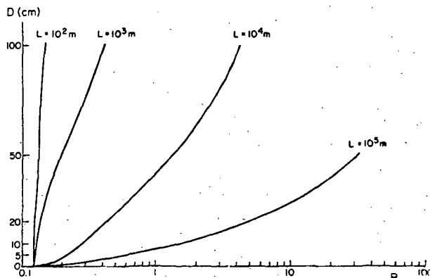
Fig. 2. R vs D for a weak turbulence C_n = 10^{-8} \text{ m}^{-1/3} at \lambda = 1 \mu .
