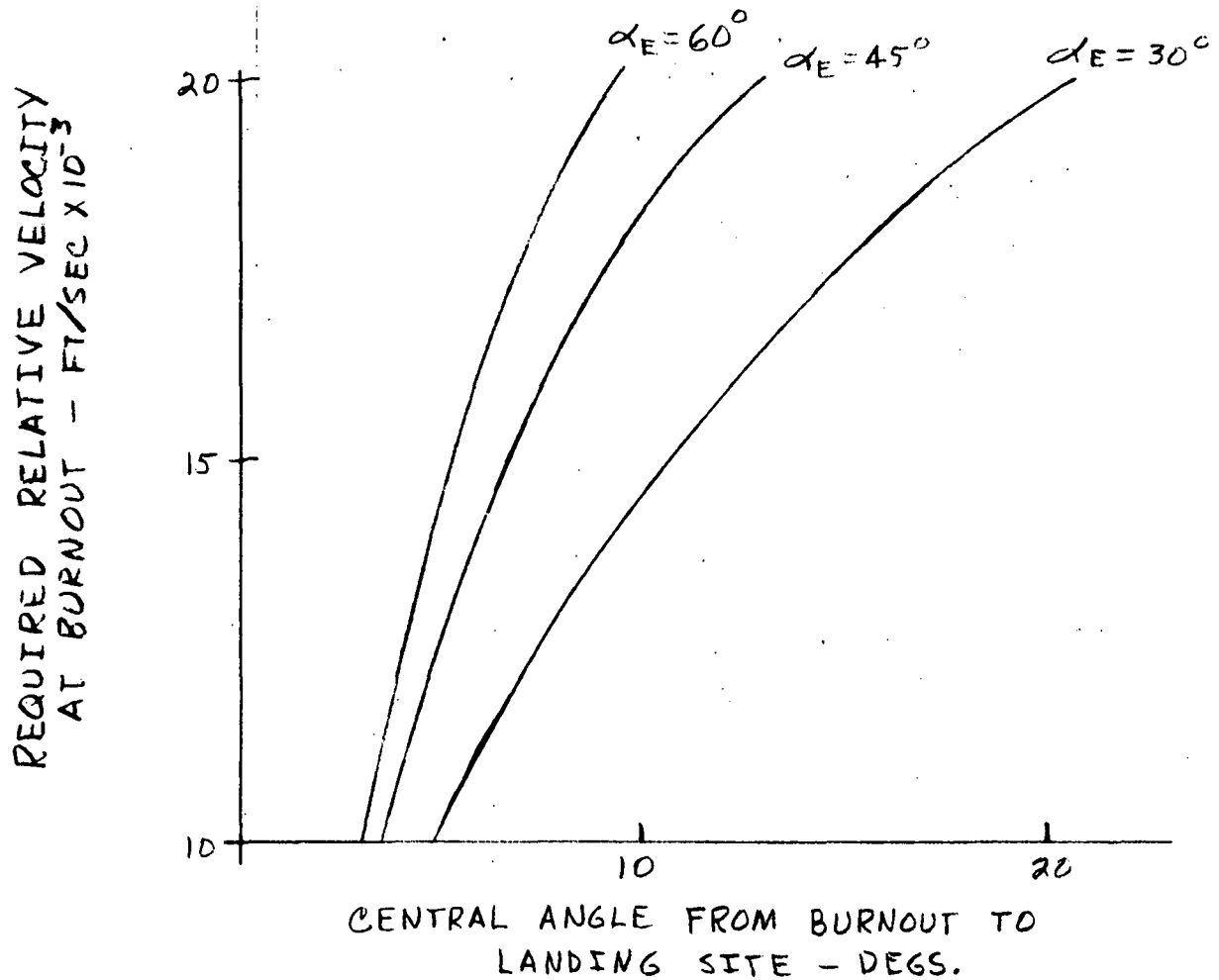
FIGURE 22 RELATION BETWEEN COAST ANGLE AND BURNOUT VELOCITY
