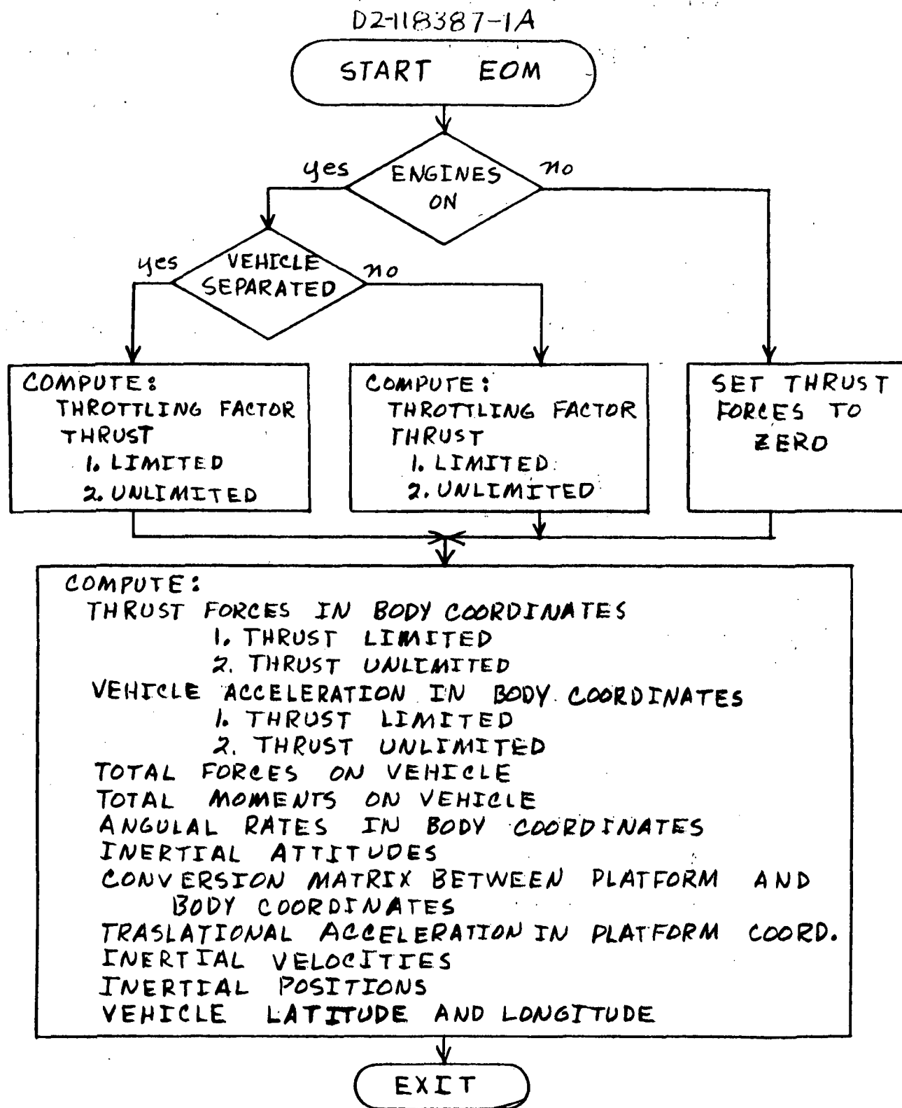
FIGURE 10 FUNCTIONAL FLOW CHART OF EOM SUBROUTINE
