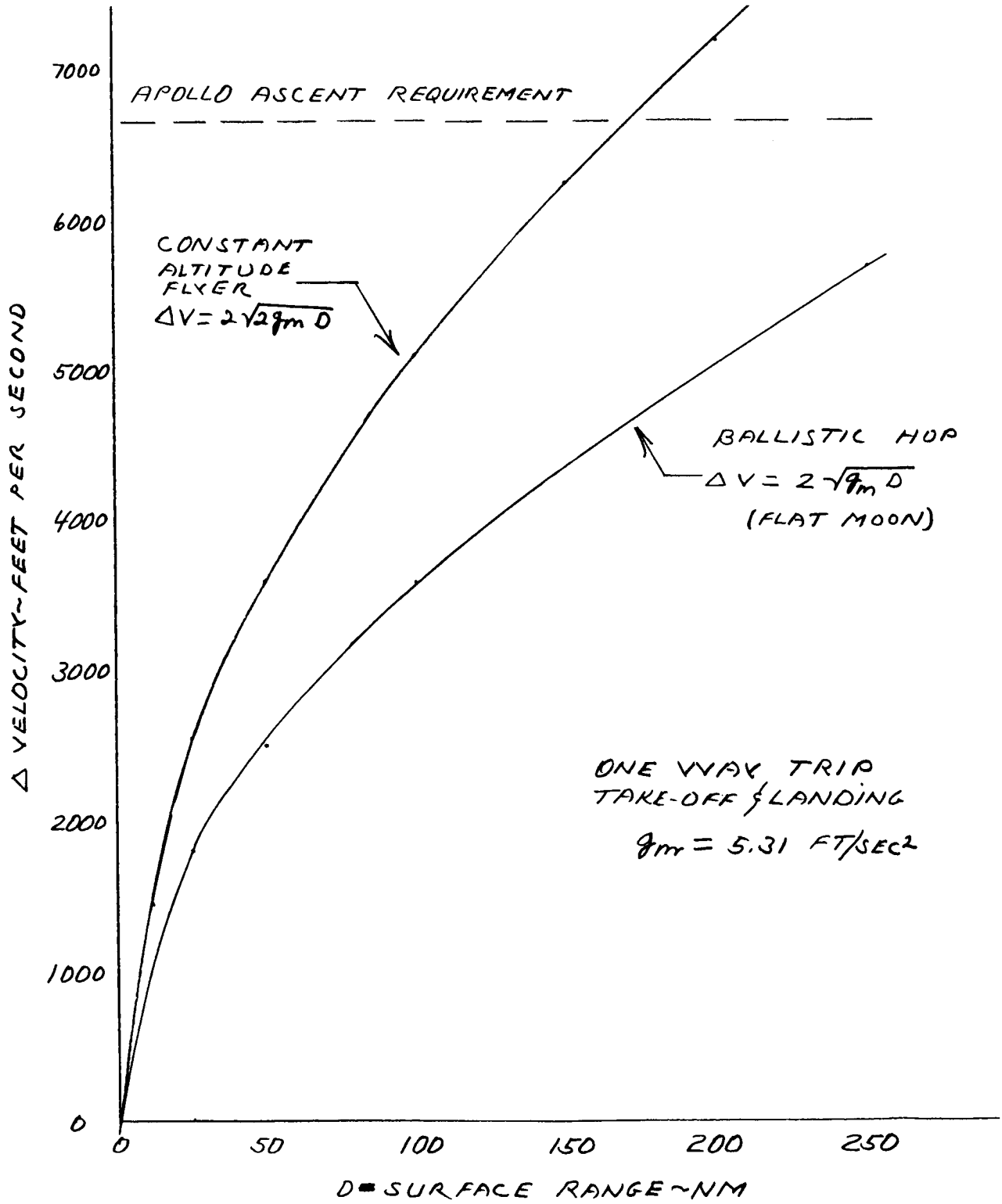
Fig. 7-9 Ballistic Hop Surface-to-Surface Velocity Requirements
