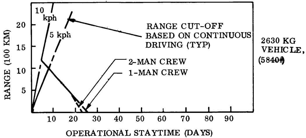
VEHICLE -01
