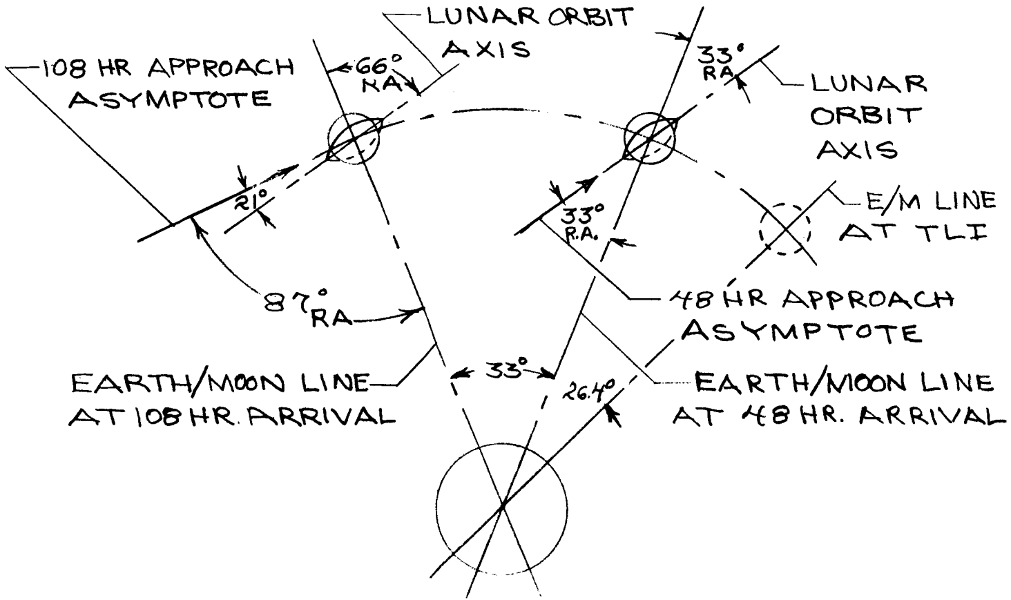
Fig. 2-14 Approach Asymptote/Lunar Orbit Alignment Vs. TL Flight Time (Simultaneous TLI From Earth Orbit)
