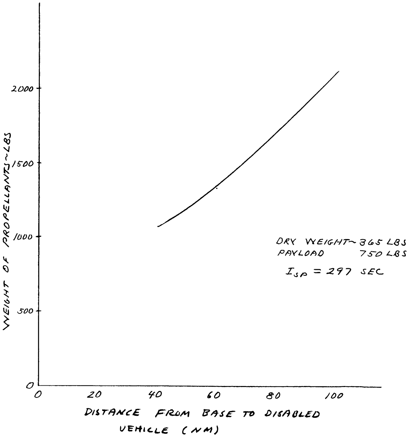
Fig. 7-8 Propellant Requirements vs. LESS/Flyer Round Trip Radius
