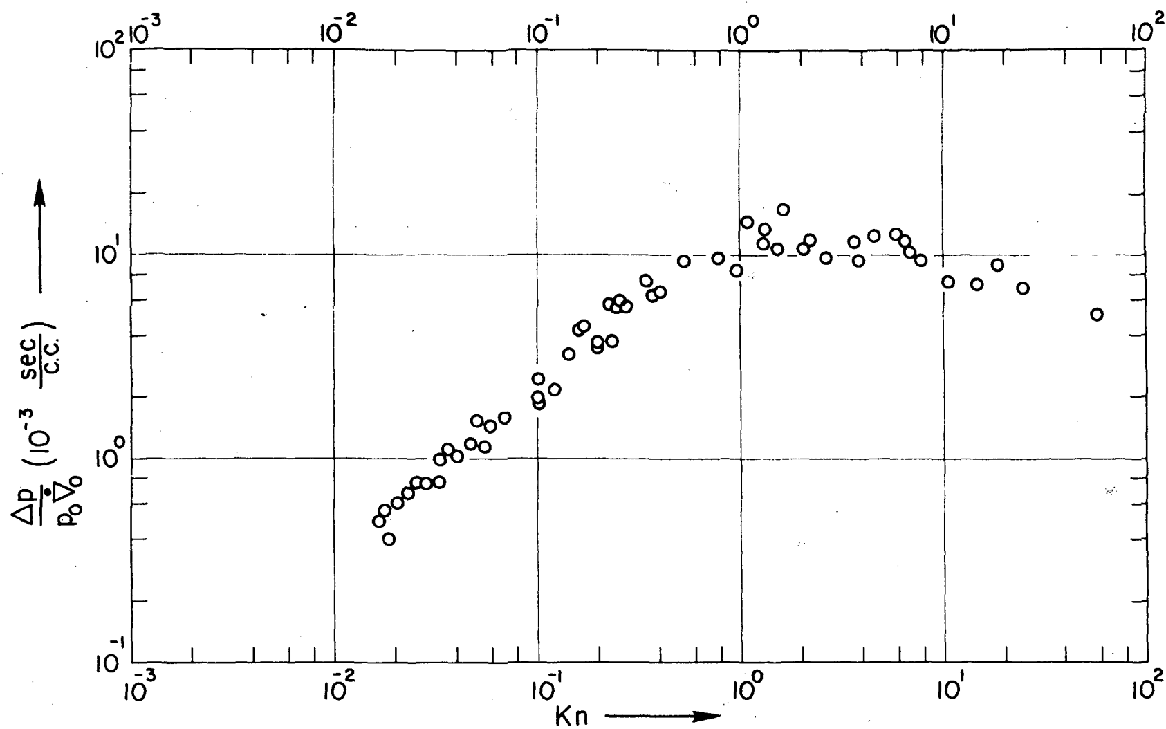
FIG. 12 MODIFIED PRESSURE GRADIENT \frac{\Delta p}{p_0 \dot{V}_0} VS Kn FOR SAND STONE SPECIMEN
