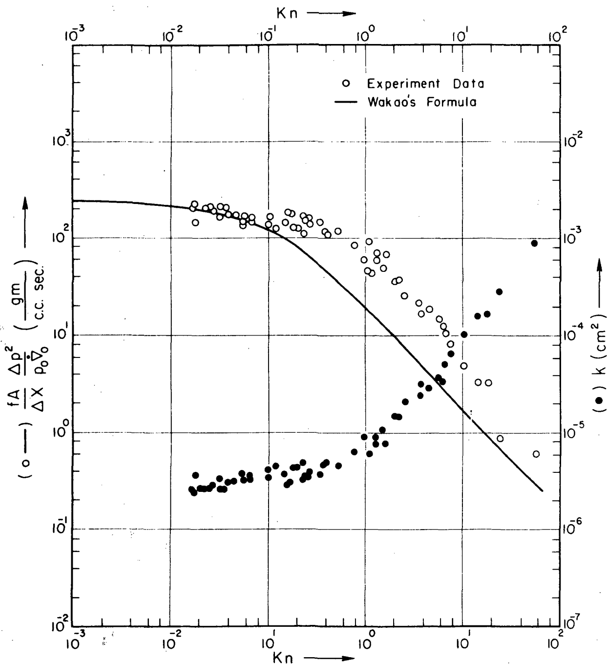
FIG. 9 \frac{fA}{\Delta X} \frac{\Delta p^2}{p_0 \dot{V}_0} \left( \frac{\text{gm}}{\text{c.c. sec.}} \right) AND PERMEABILITY, k , VS Kn FOR SAND STONE SPECIMEN
