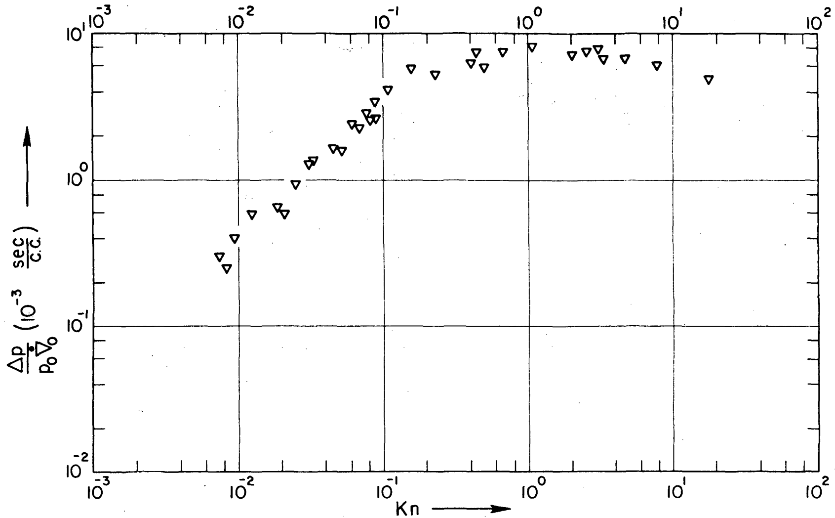
FIG. 11 MODIFIED PRESSURE GRADIENT \frac{\Delta p}{p_0 \nabla_0} VS Kn FOR 3mm SINTERED GLASS BEAD SPECIMEN
