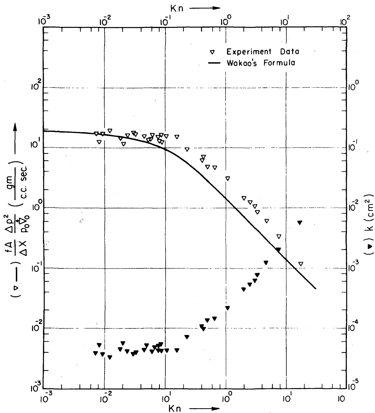
FIG. 8 \frac{fA}{\Delta X} \frac{\Delta p^2}{\rho_0 \nabla_0} \left( \frac{\text{gm}}{\text{c.c. sec.}} \right) AND PERMEABILITY, k , VS Kn FOR 4mm SINTERED GLASS BEAD SPECIMEN
