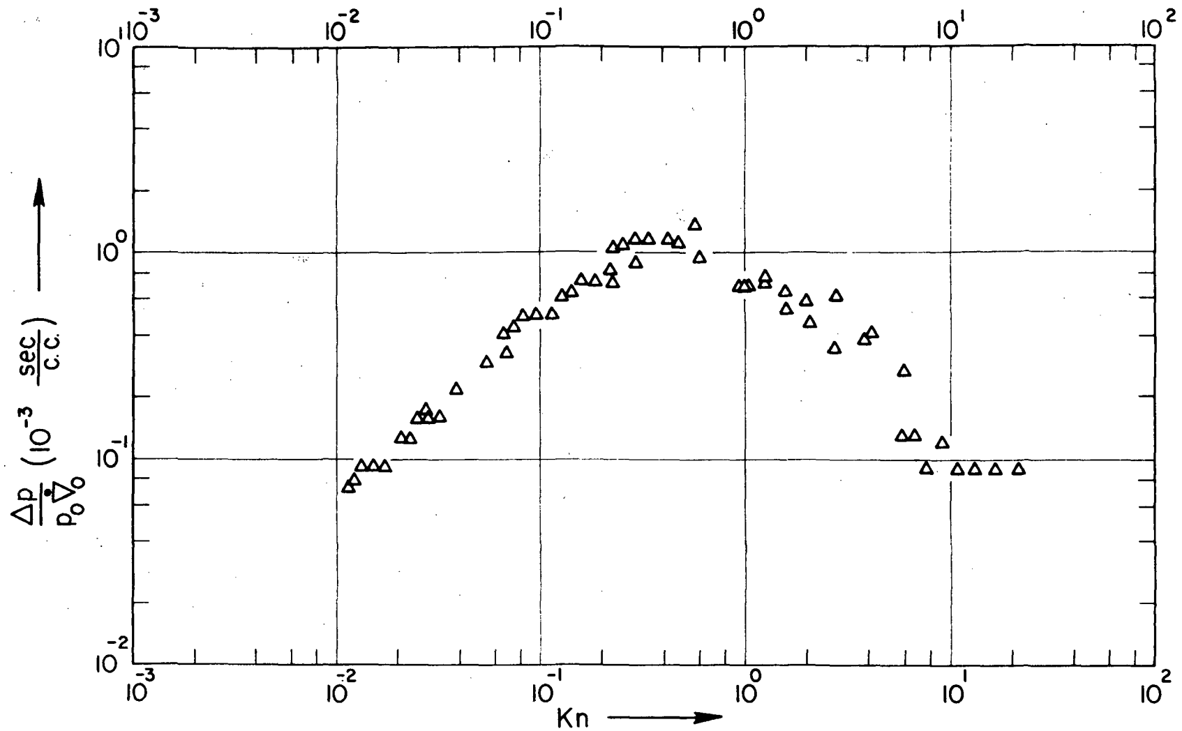
FIG. 10 MODIFIED PRESSURE GRADIENT \frac{\Delta p}{p_0 \nabla_0} VS Kn FOR 3mm SINTERED GLASS BEAD SPECIMEN
