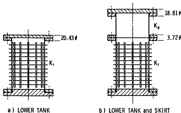
Fig. 3. Intermediate Empty Configuration of Booster Model
