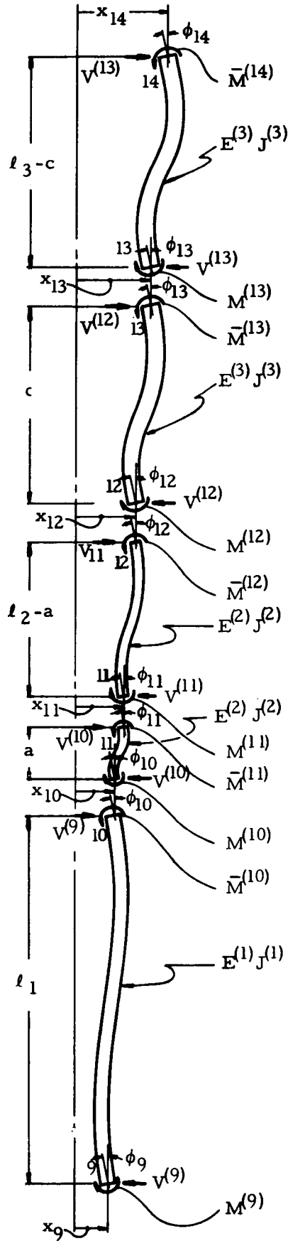
Fig. 2d. Detail of Booster Reinforcing Beam
