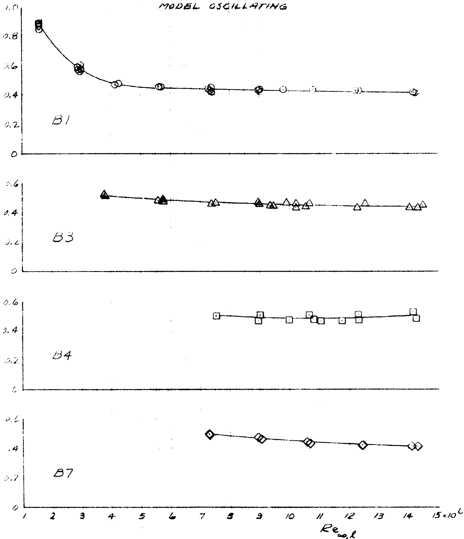
FIG. 18 MEAN BASE PRESSURE , M_\infty \approx 11.3
