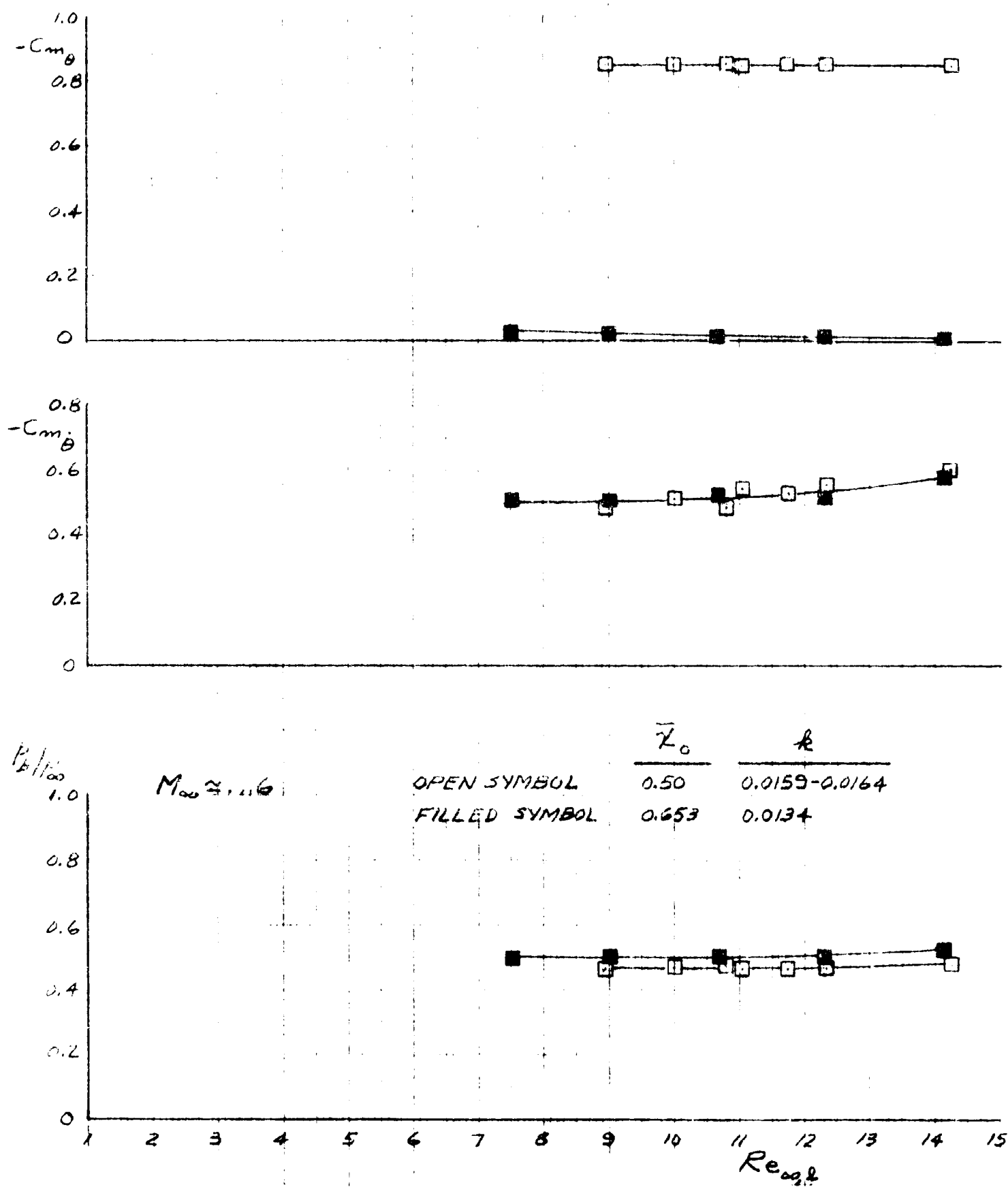
FIG. 21 RESULTS FOR MODEL B4
