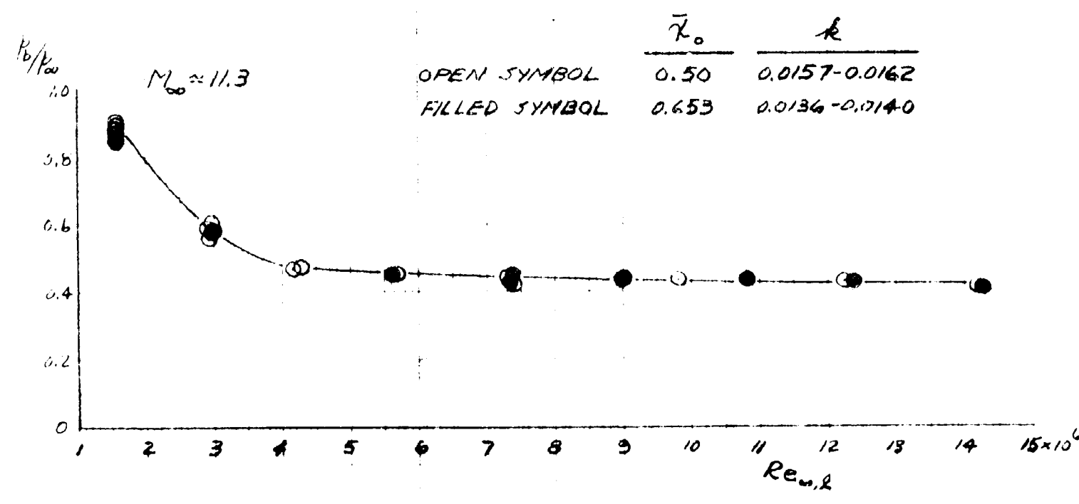
FIG.19 RESULTS FOR MODEL B1
