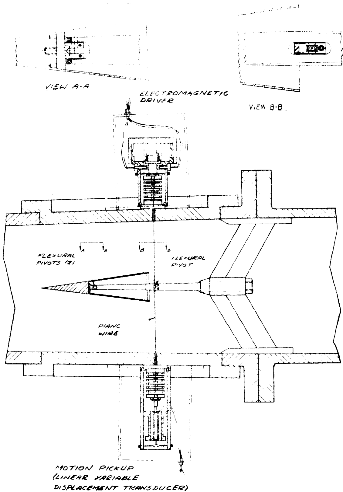
Fig. 6 SCHEMATIC OF OSCILLATORY APPARATUS AND MODEL IN THE HYPERSONIC WIND TUNNEL
