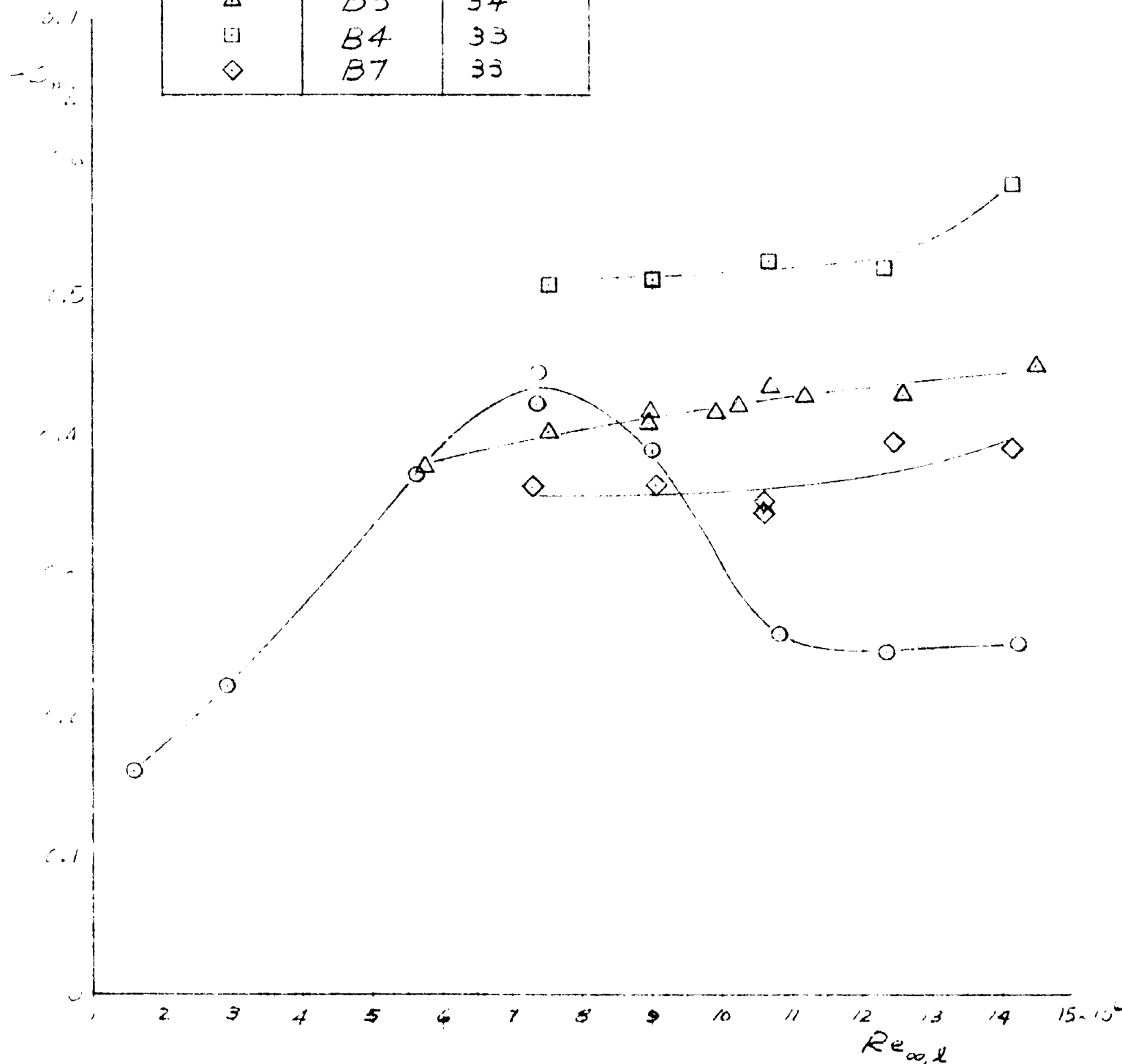
FIG. 15 DAMPING-IN-PITCH DERIVATIVE
