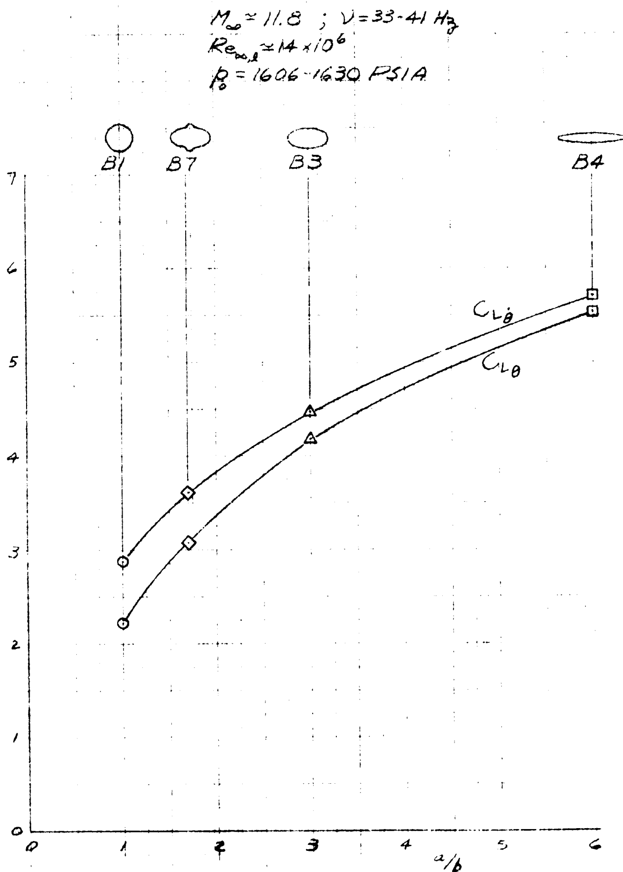
FIG.25 LIFT DERIVATIVES ABOUT APEX
