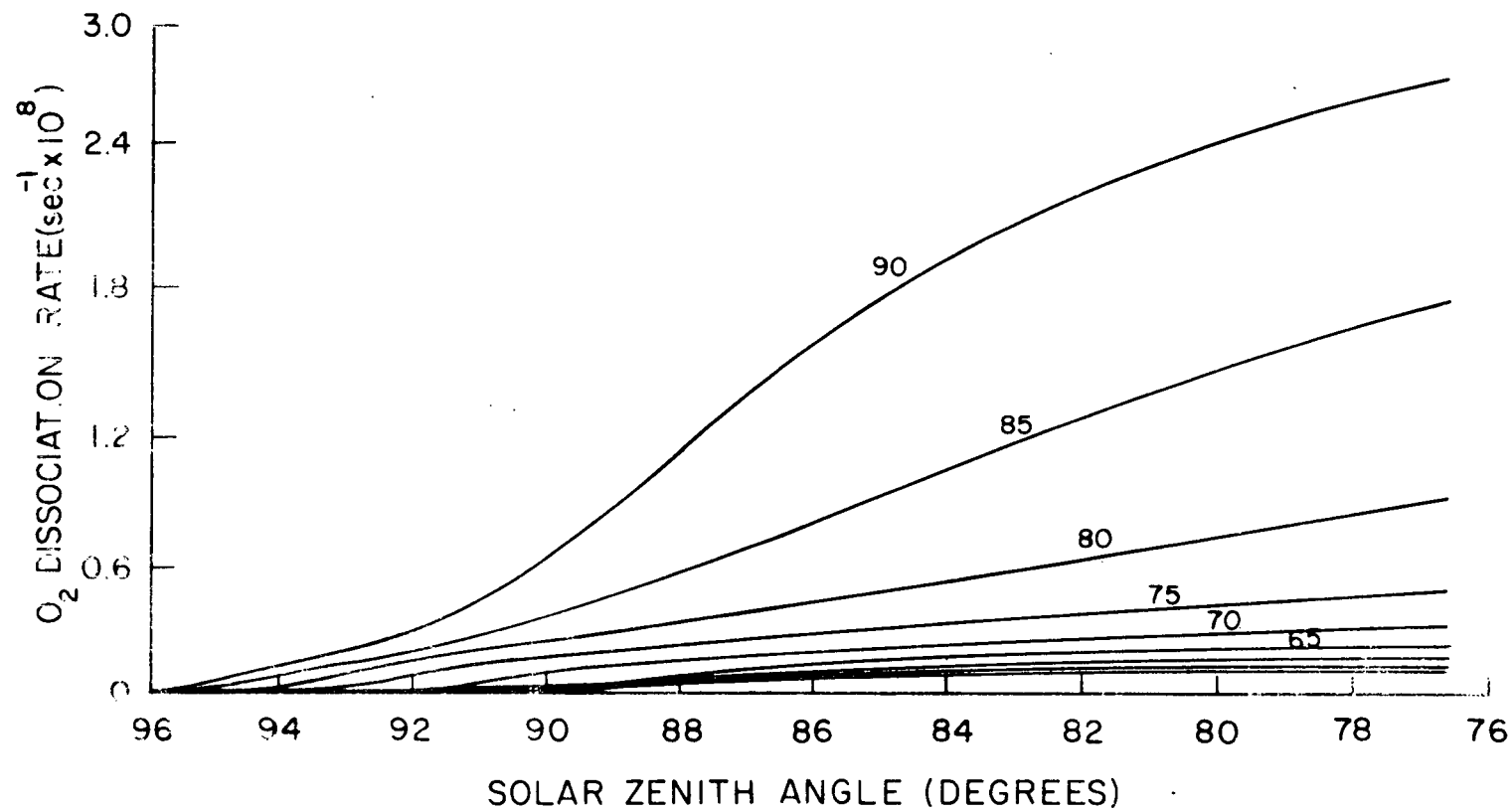
Figure 3.4 Molecular oxygen photodissociation rates over sunrise.
