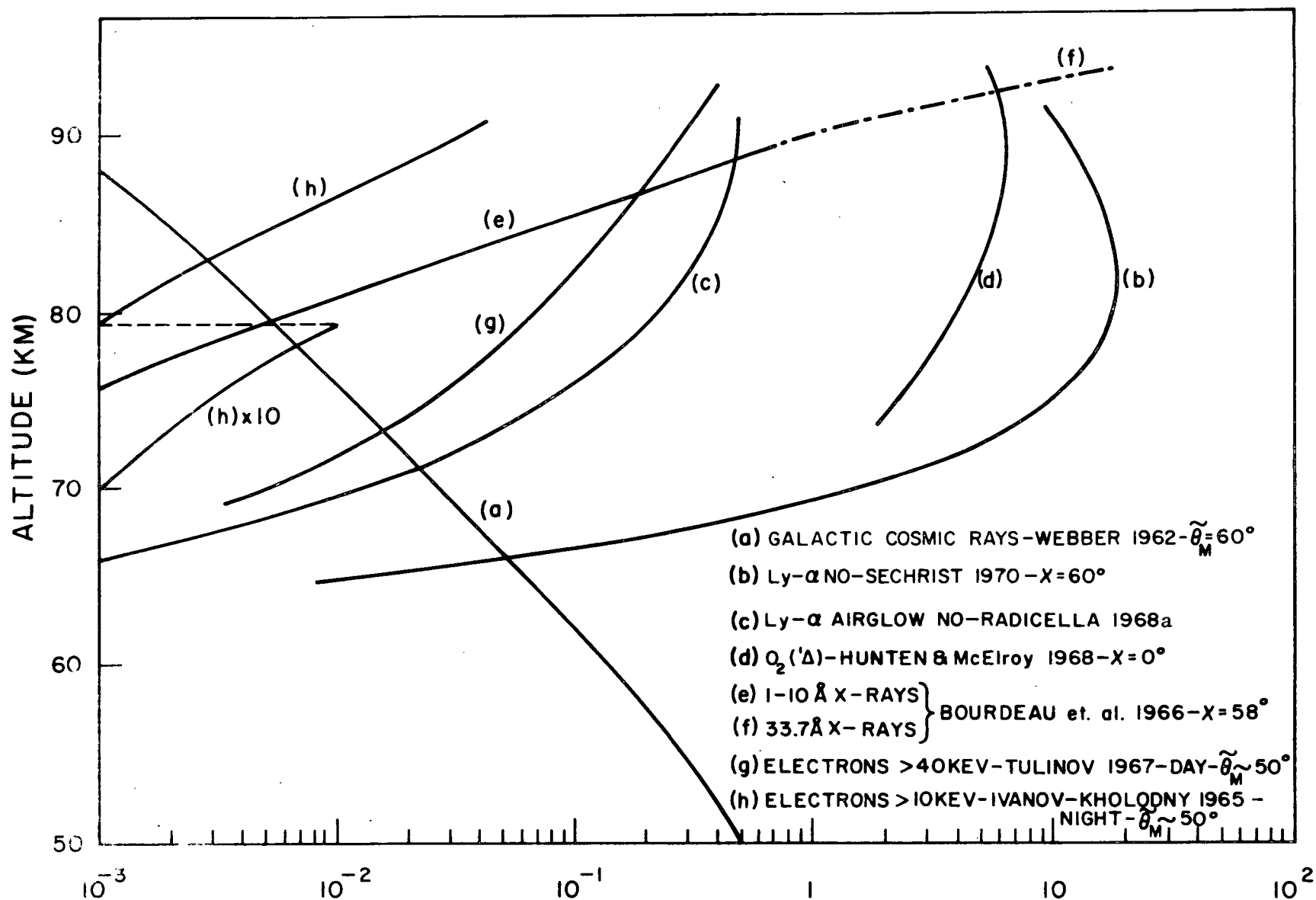
Figure 5.1 Ion-pair production rates in the D region.
