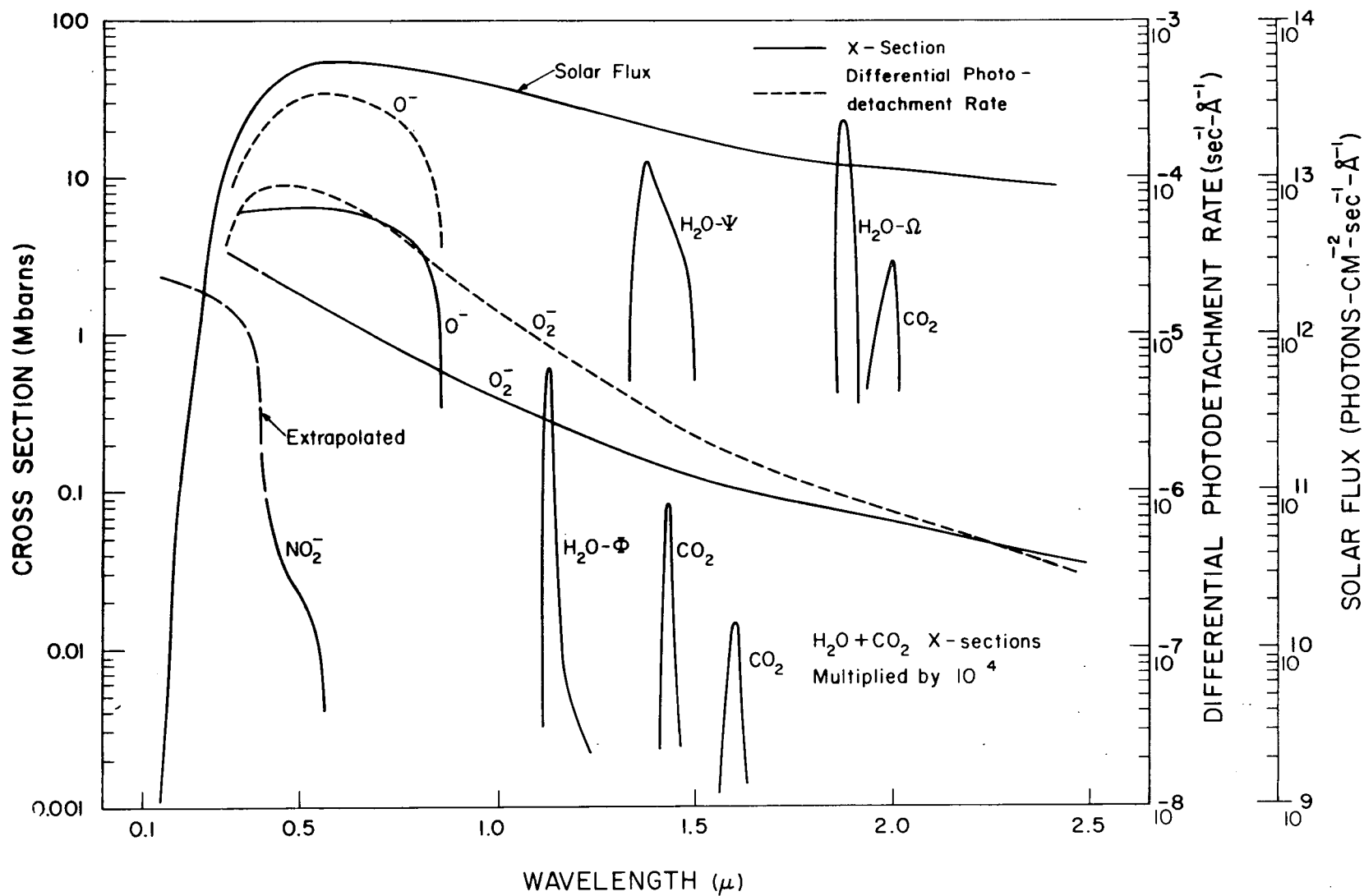
Figure 7.3 Photodetachment cross sections of negative ions and infrared absorption cross sections of \text{H}_2\text{O} and \text{CO}_2 .
