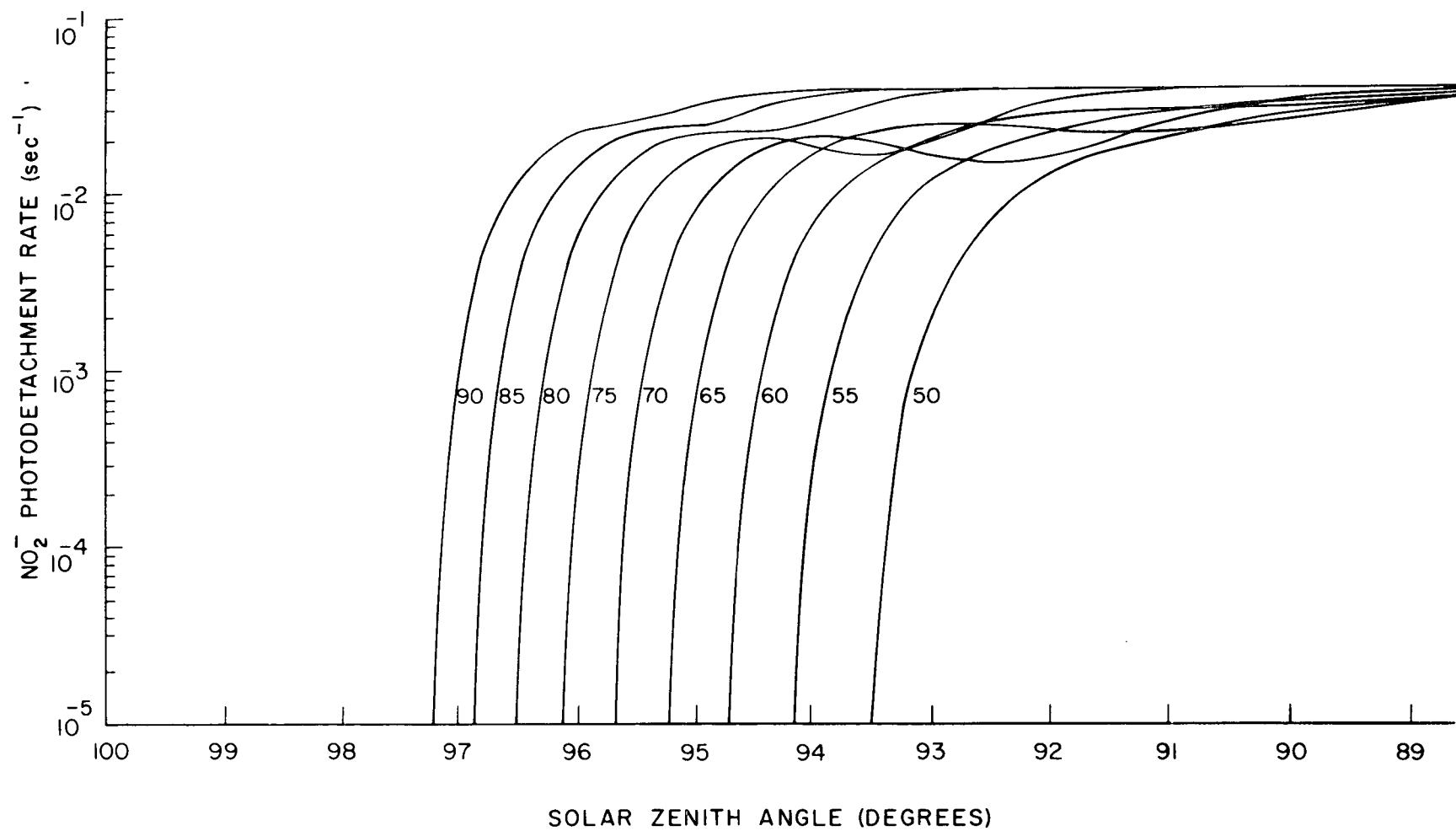
Figure 7.6 \text{NO}_2^- photodetachment rates over sunrise.
