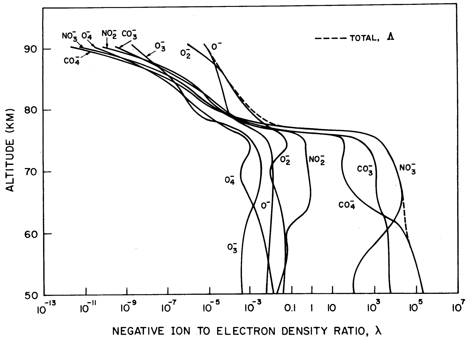
Figure 8.13 Negative ion-to-electron density ratios in the presunrise D region.
