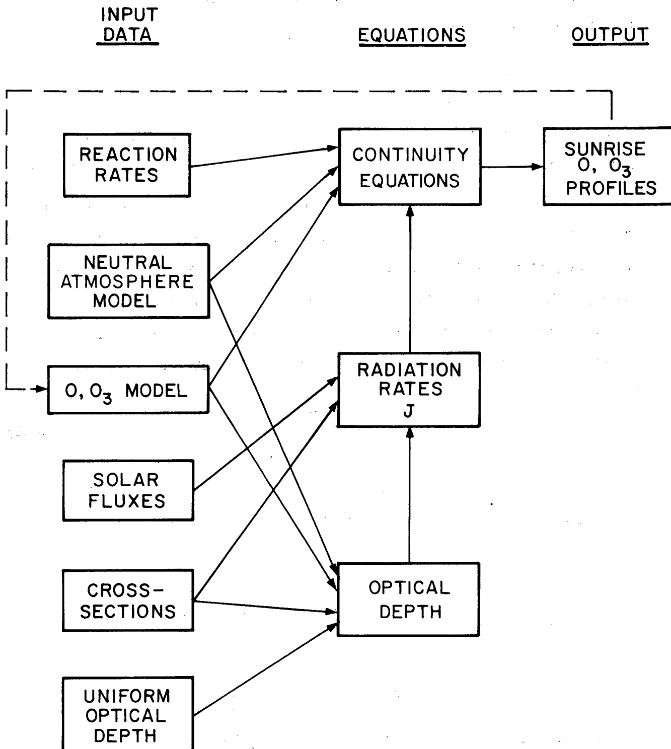
Figure 3.3 Solution scheme for the oxygen atmosphere.
