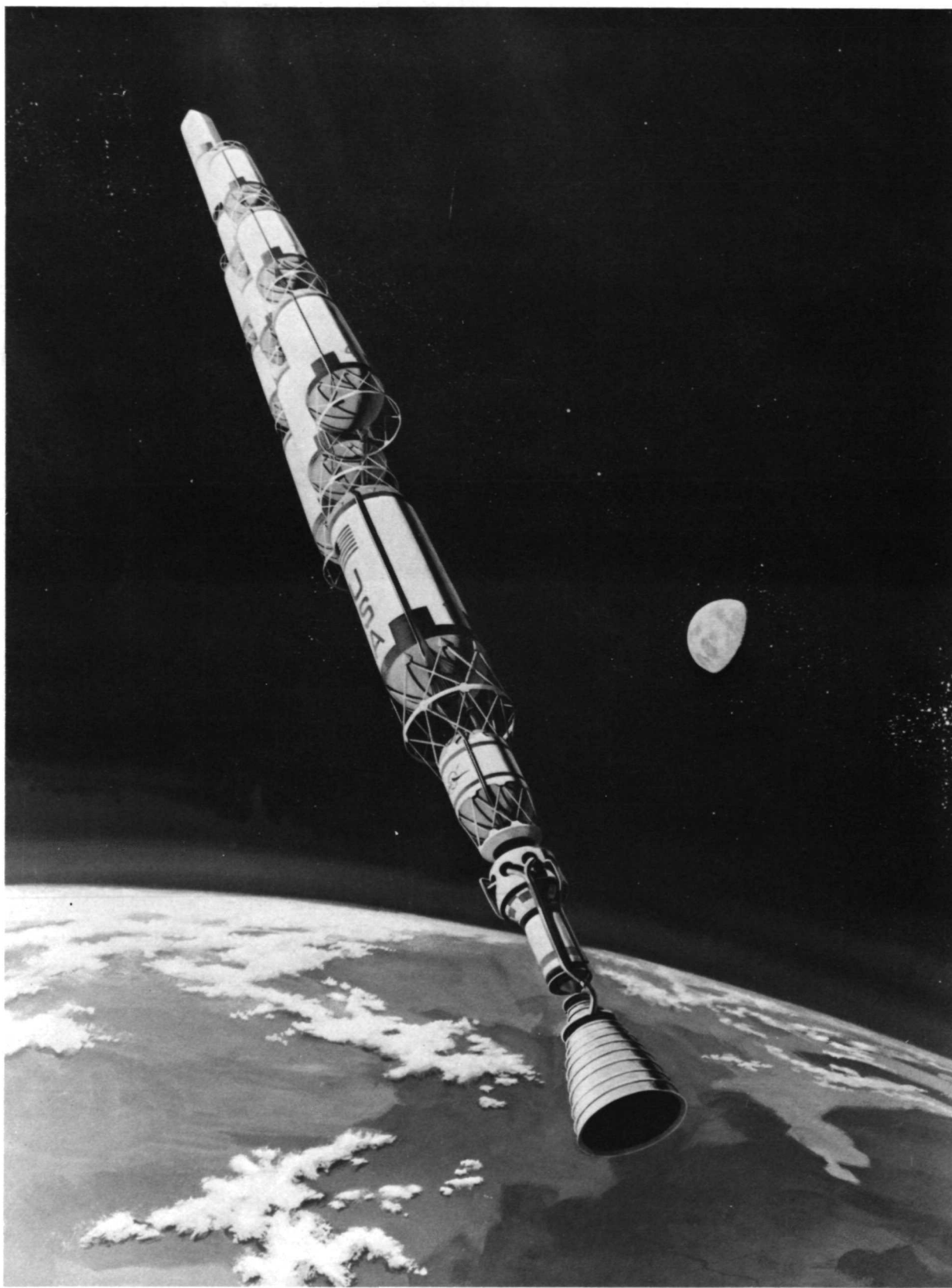
Fig. A-4. Reusable nuclear stage multiple-tank concept
