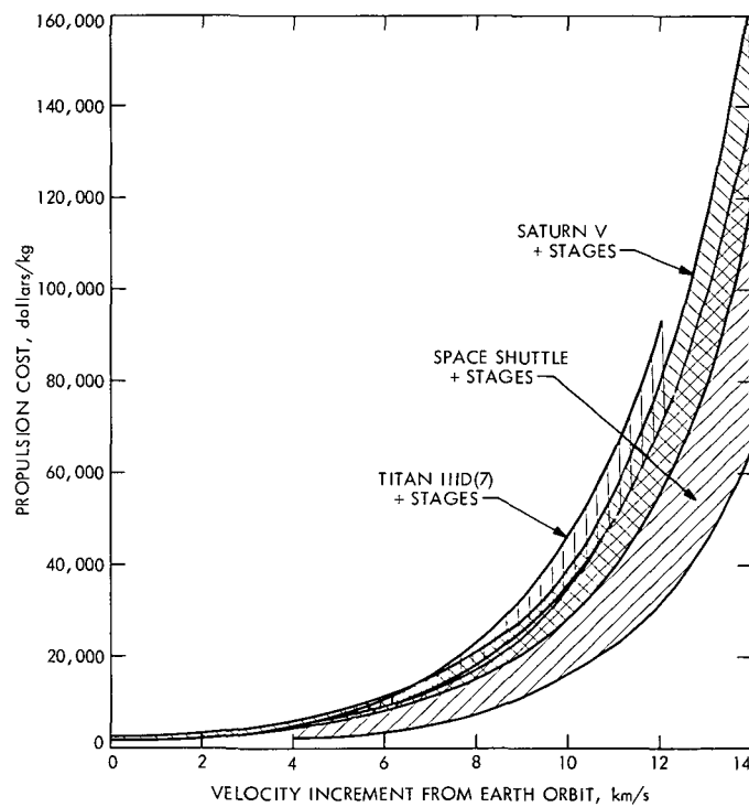
Fig. 4. Propulsion cost comparisons per unit payload beyond Earth orbit (chemical propulsion)
