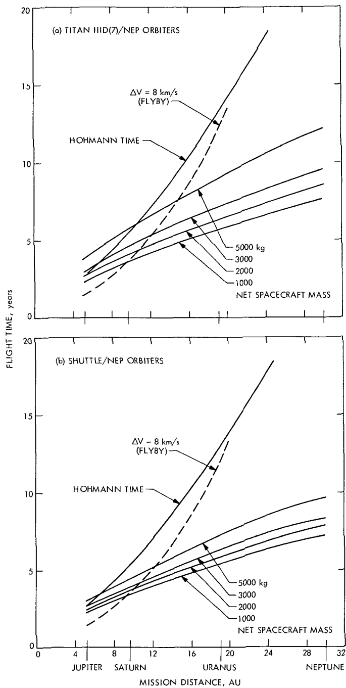
Fig. 5. Planetary mission flight times a. Titan IIID(7)/NEP orbiters b. Shuttle/NEP orbiters
