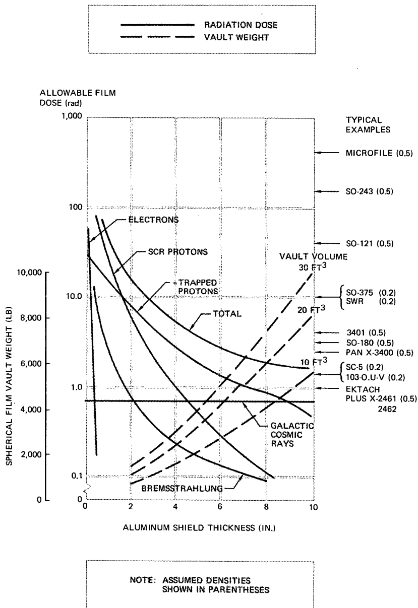
Figure 3-16. Film Vault Shield Requirements—90 Day Dose
