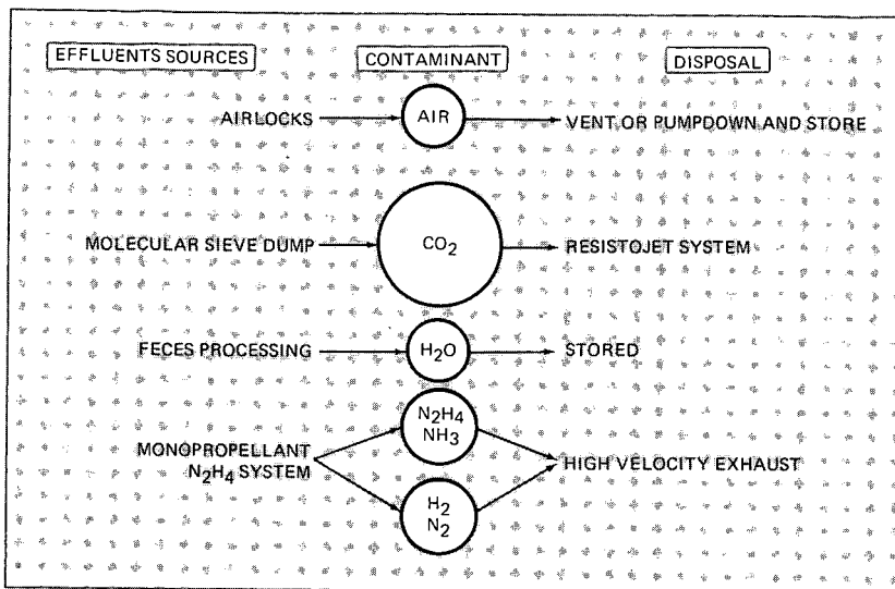
Figure 3-18. Space Station Effluent Sources
