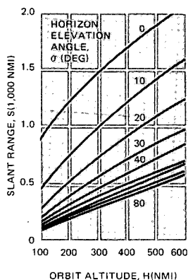
Figure 3-25. Slant Range, S
