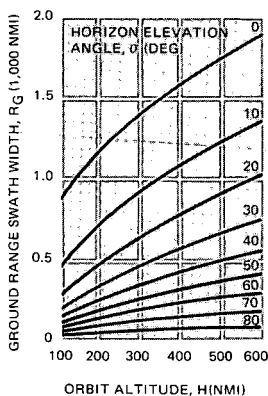
Figure 3-24. Ground Range Swath Width, R_G
