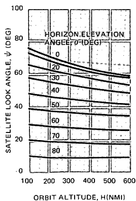
Figure 3-23. Satellite Look Angle, \psi
