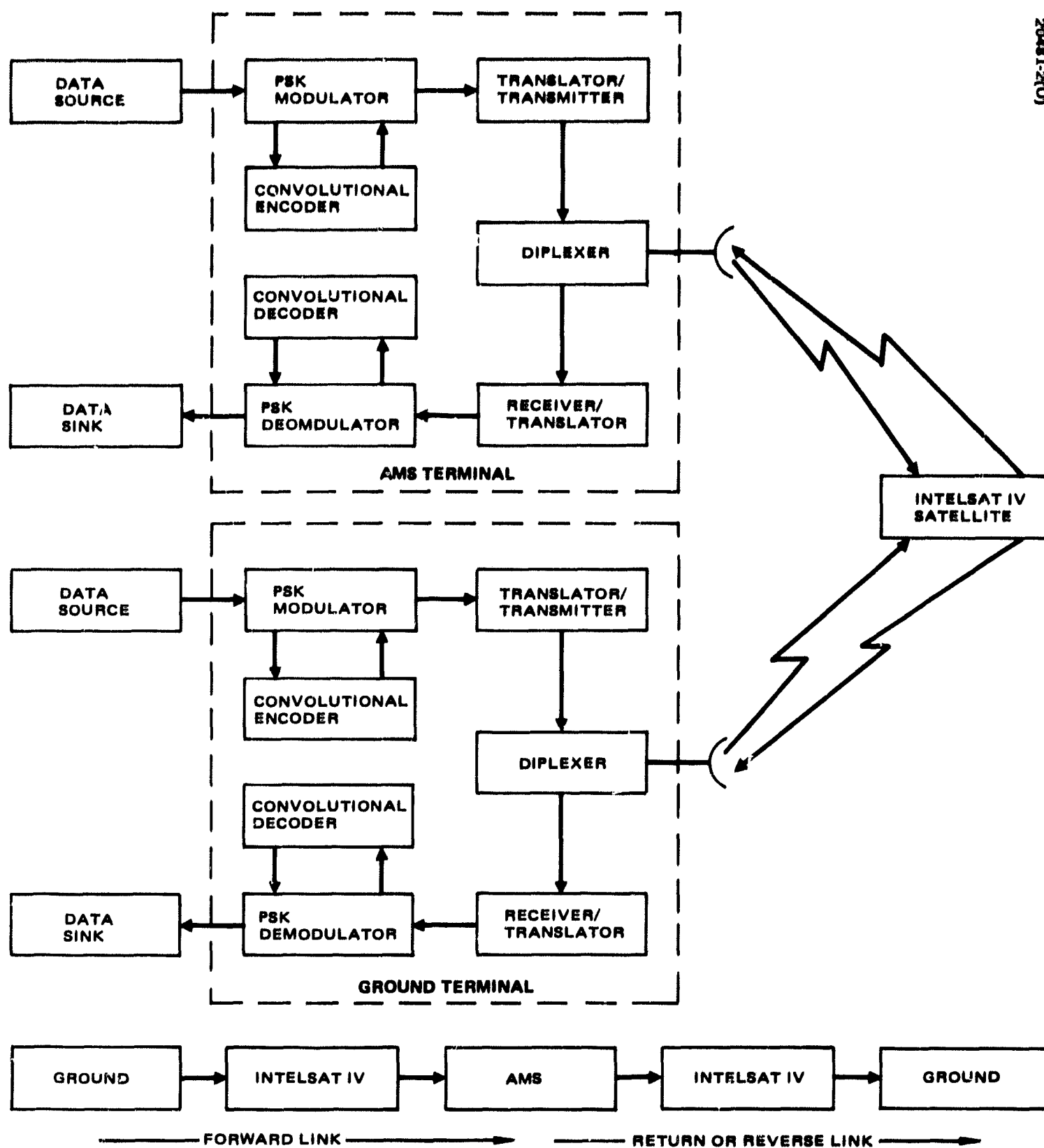
Figure 2. AMS Two-Way Communications Link
