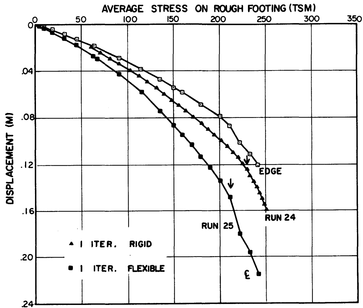
FIGURE 4.9: FLEXIBLE VRS RIGID FOOTING
