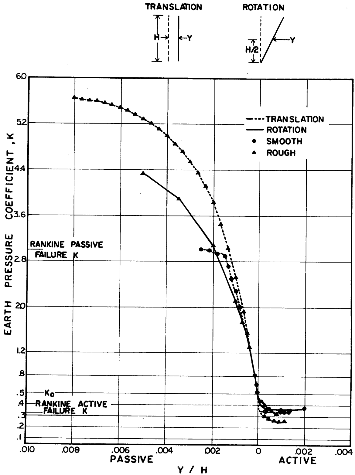
FIGURE 4.4: ROTATION VRS. TRANSLATION OF RETAINING WALL
