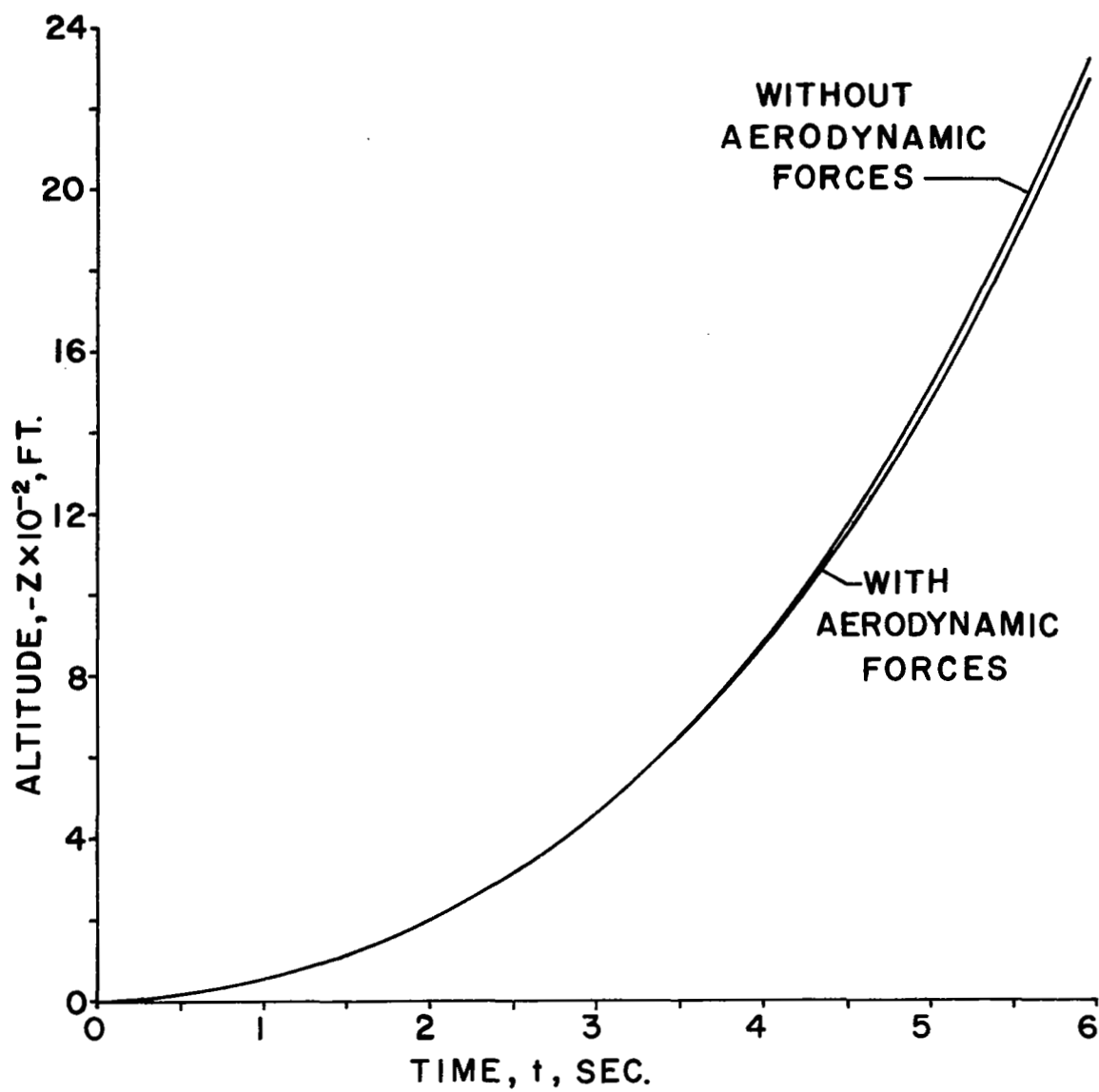
Figure 10 - Altitude vs. Time
