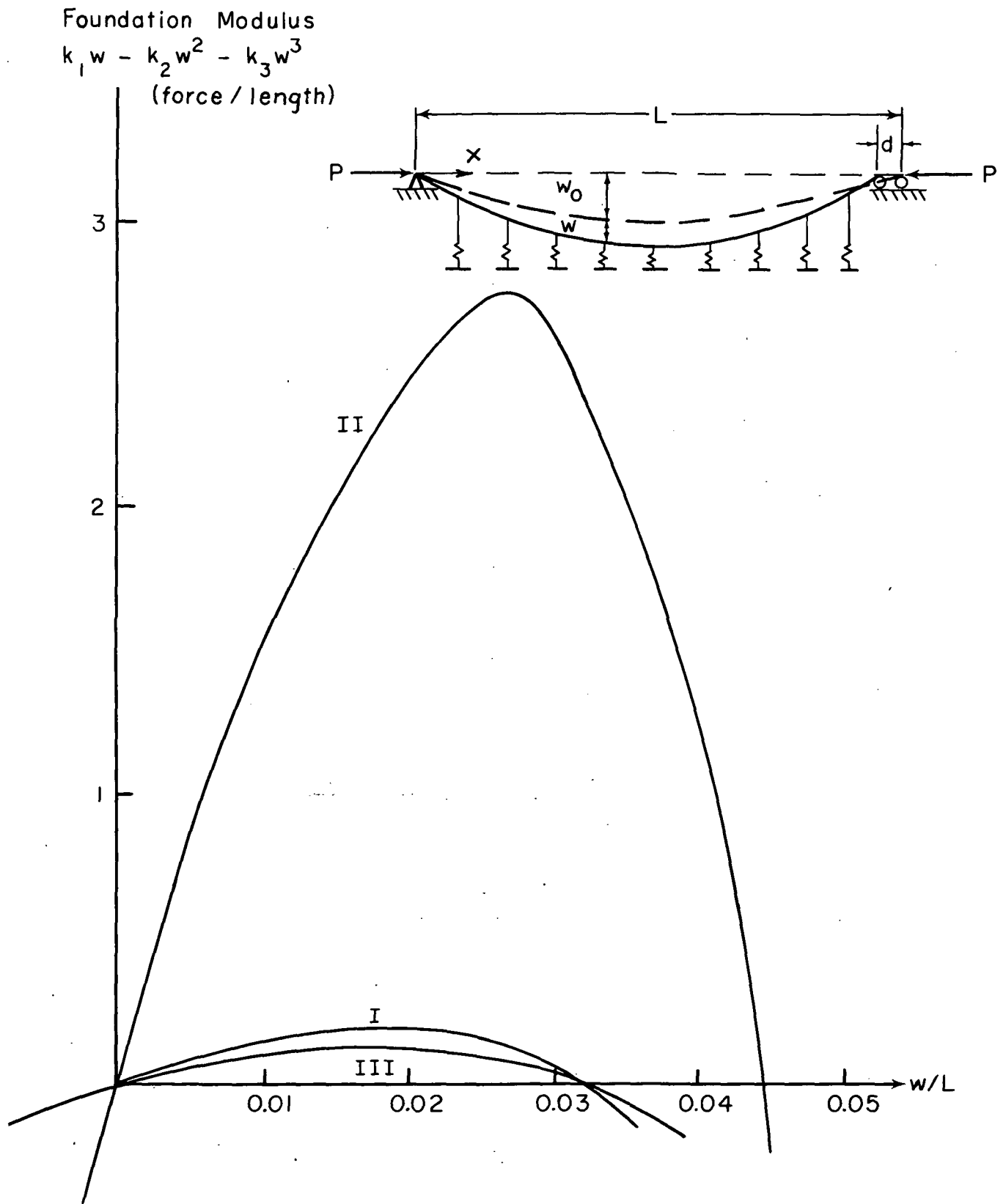
3. Foundation Properties. Beam on Nonlinear Elastic Foundation.
