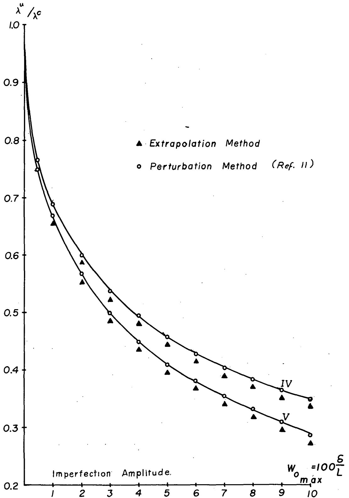
6. Beam on Nonlinear Elastic Foundation. Limit Load as a Function of w_0 . Cases IV-V.
