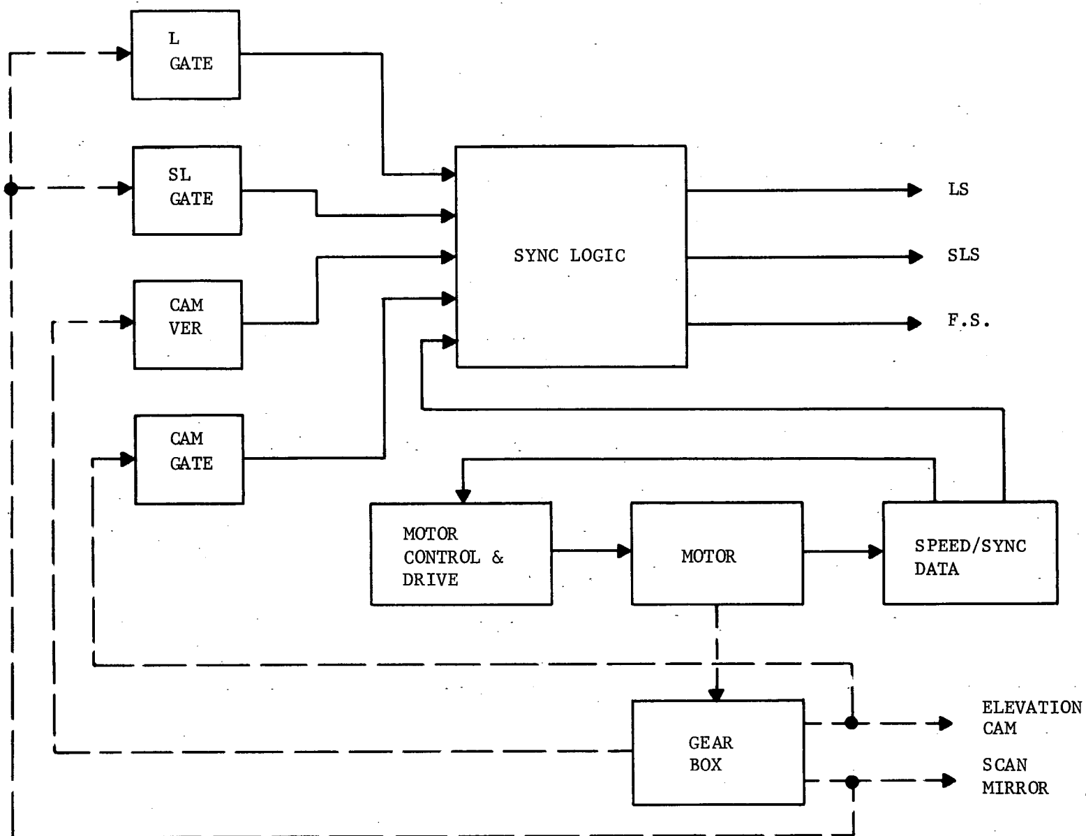
FIGURE 4. SCANNER BLOCK DIAGRAM
