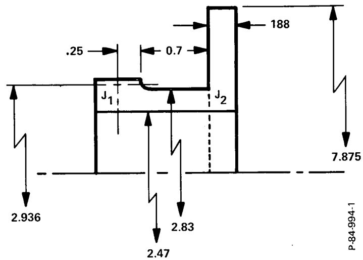
Figure B-11 - Inboard Ground Gear (Breadboard)
