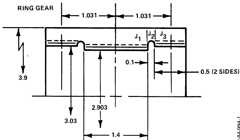
Figure B-8 - Ring Gear (Breadboard)
