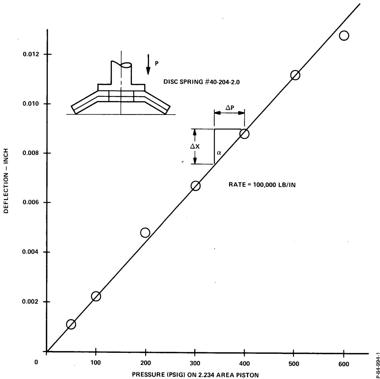
Figure A-3 - Schnorr Disc Spring Deflection Curve
