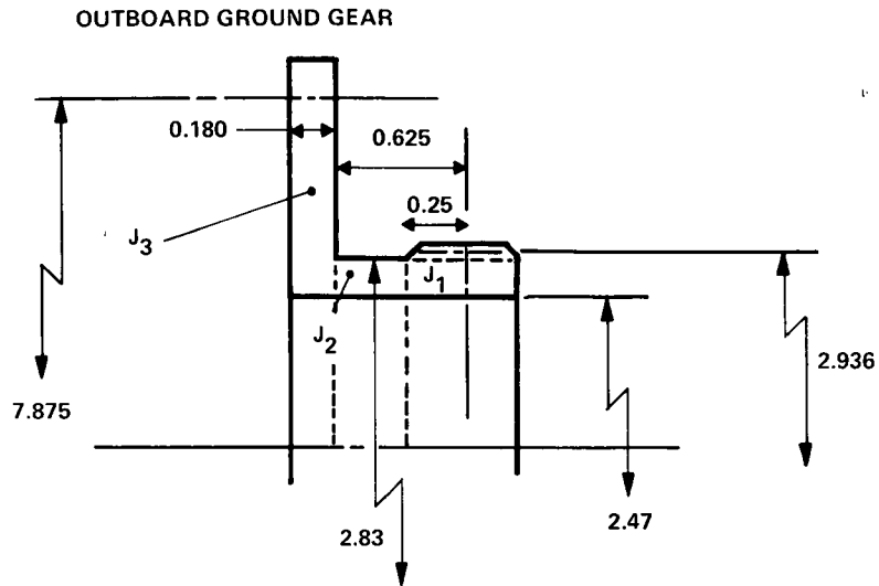
Figure B-9 - Outboard Ground Gear (Breadboard)
