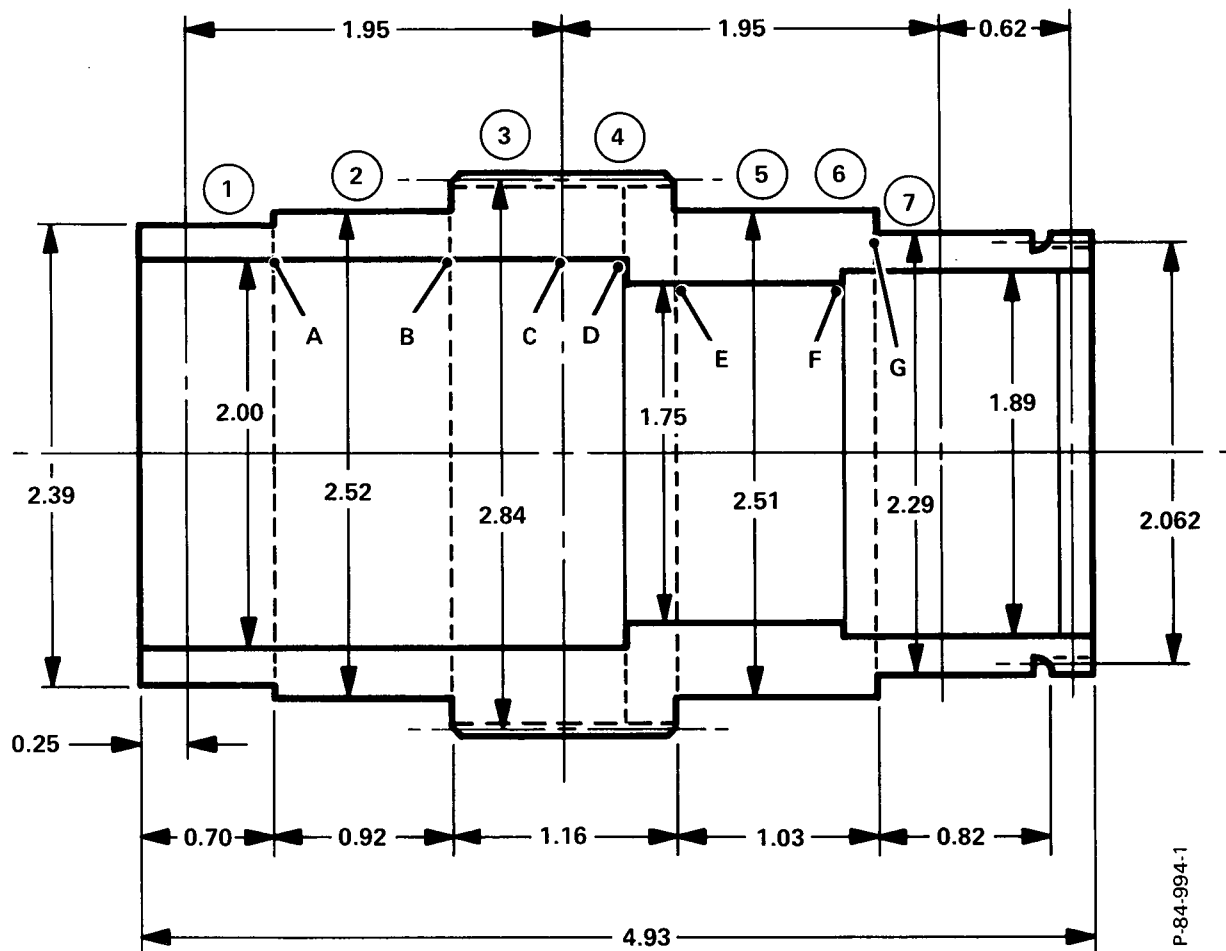
Figure B-1 - Actuator Output Gear (Flightweight)
