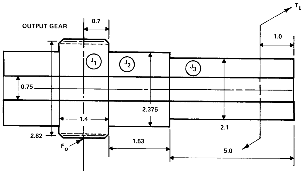
Figure B-7 - Output Gear (Breadboard)
