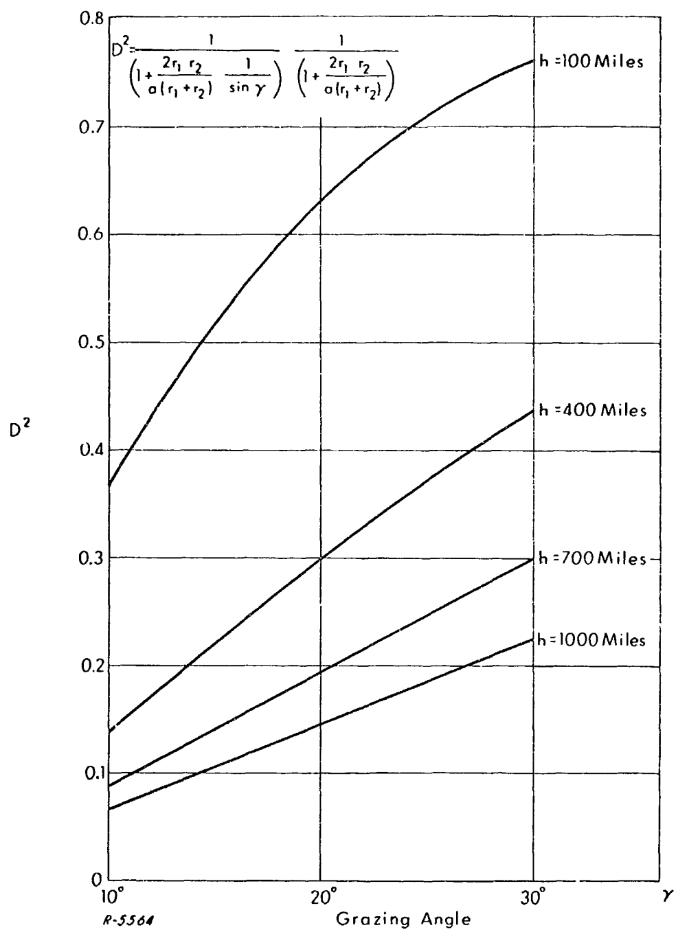
Fig. 2 Divergence Factor
