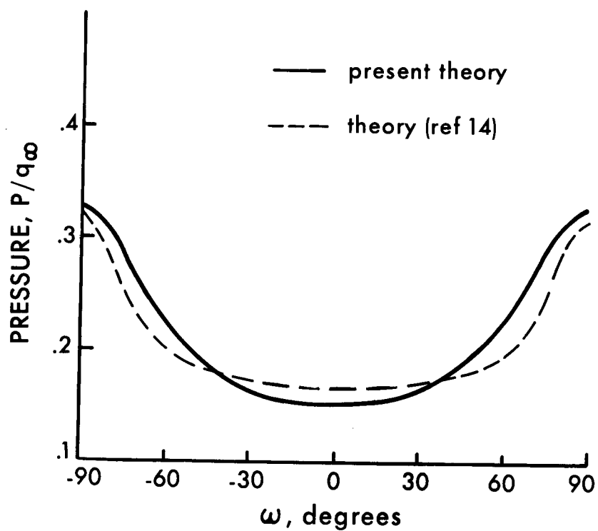
Fig. 4 - Surface pressure, shock shape and streamlines for 12.9° x 21.3° elliptic cone at M = 6.0 , \alpha = 0^\circ
