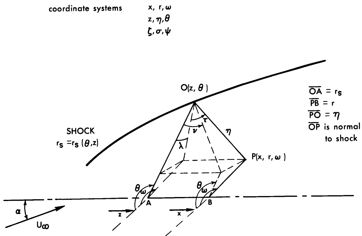
Fig. 1 - Coordinate systems
