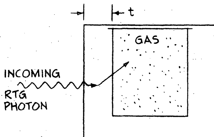
FIG. 10 CROSS SECTION OF PROPORTIONAL CENTER
