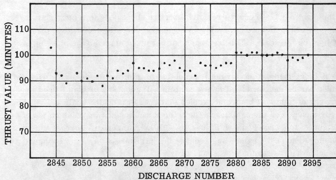
Figure 15. Sample Record of Data for a Test Series (Second Sheet) Showing Impulse Reading as a Function of Discharge Number
