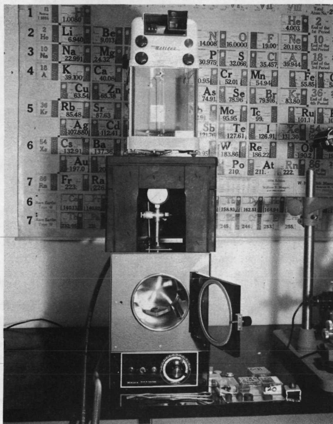
Figure 12. Setup of Vacuum Oven and Balance Used for Drying and Weighing Arc Chamber Parts
