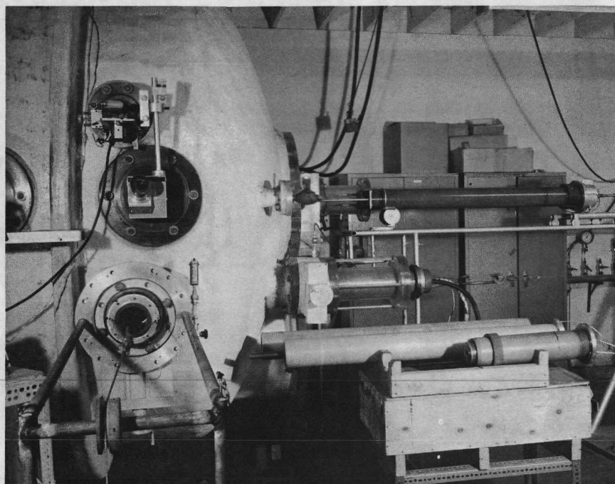
Figure 9. Side View of the Test Chamber
