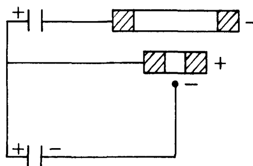
Front Cathode Trigger - on Anode
