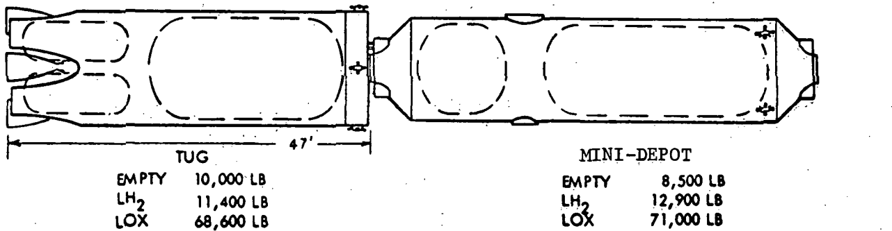
Figure 4-19. Permanent Tankage, Linear Mini-Depot
