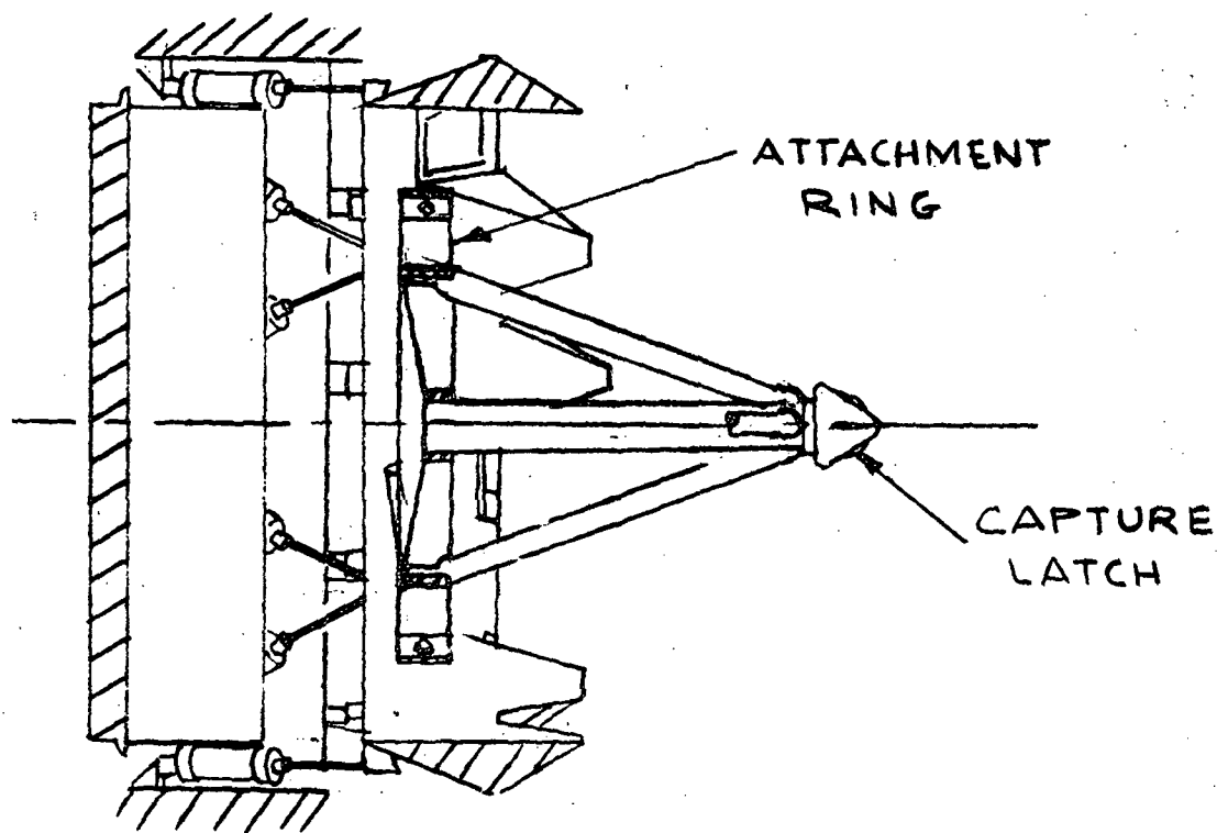
Figure 2-3. Ring Design with Apollo Probe Attached
