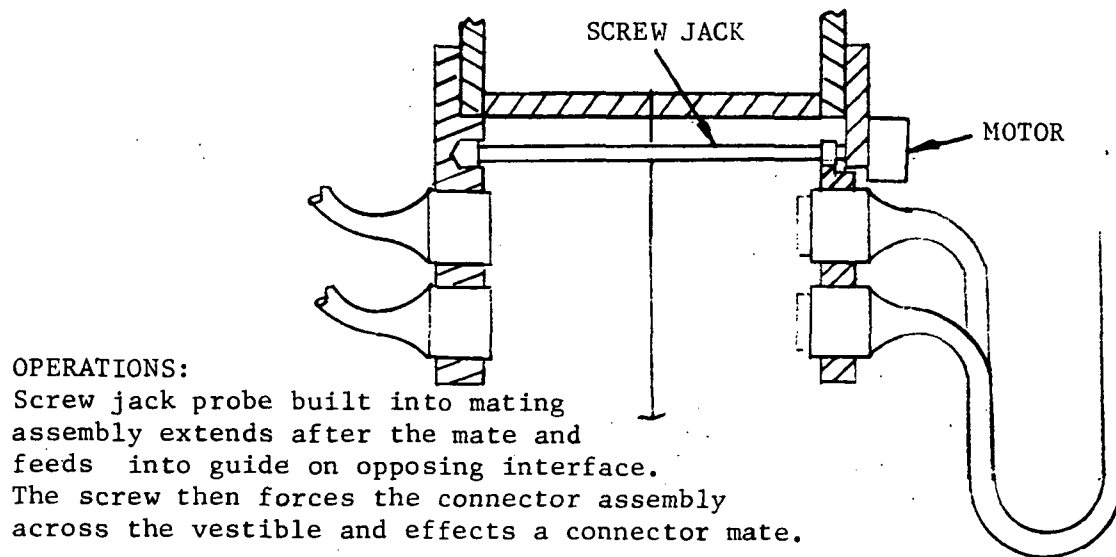
Figure 2-16. Automatic Multiple Connector Concept
