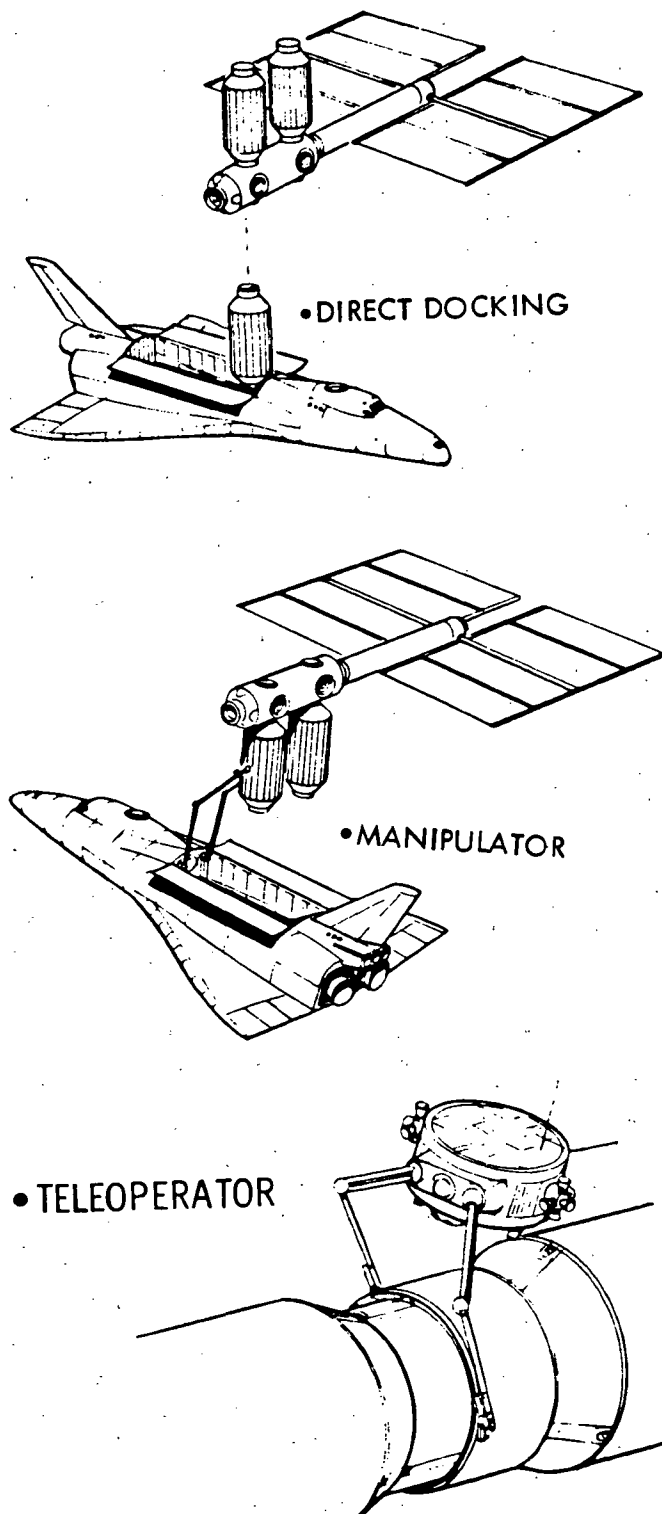
Figure 2-3. Orbital Assembly Alternate Approaches through Hard Dock
