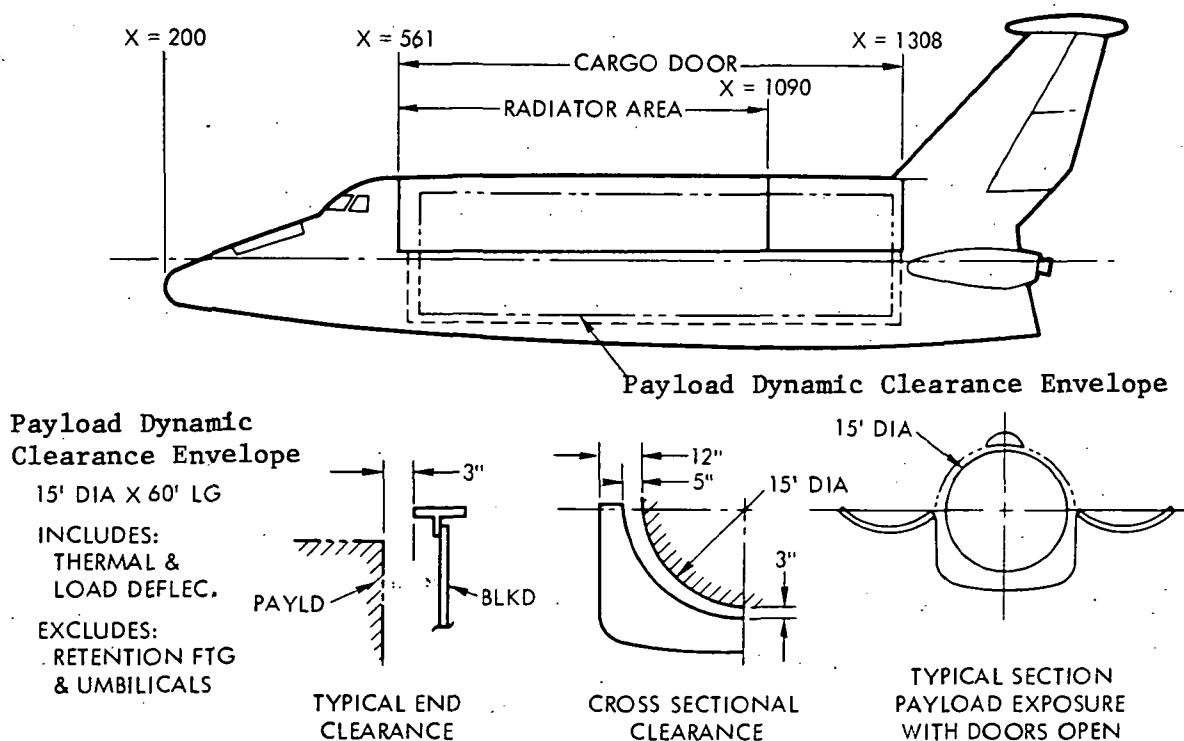
Figure 5-4. Orbiter/Payload Envelope
