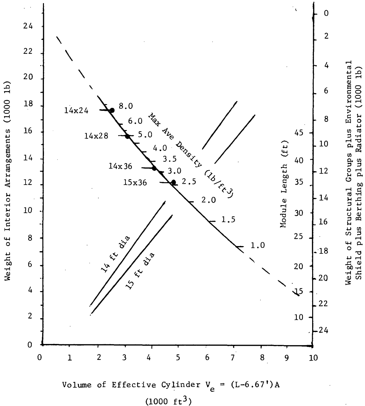
Figure 2-21. Weight-Length-Density Correlation for Modular Space Station
