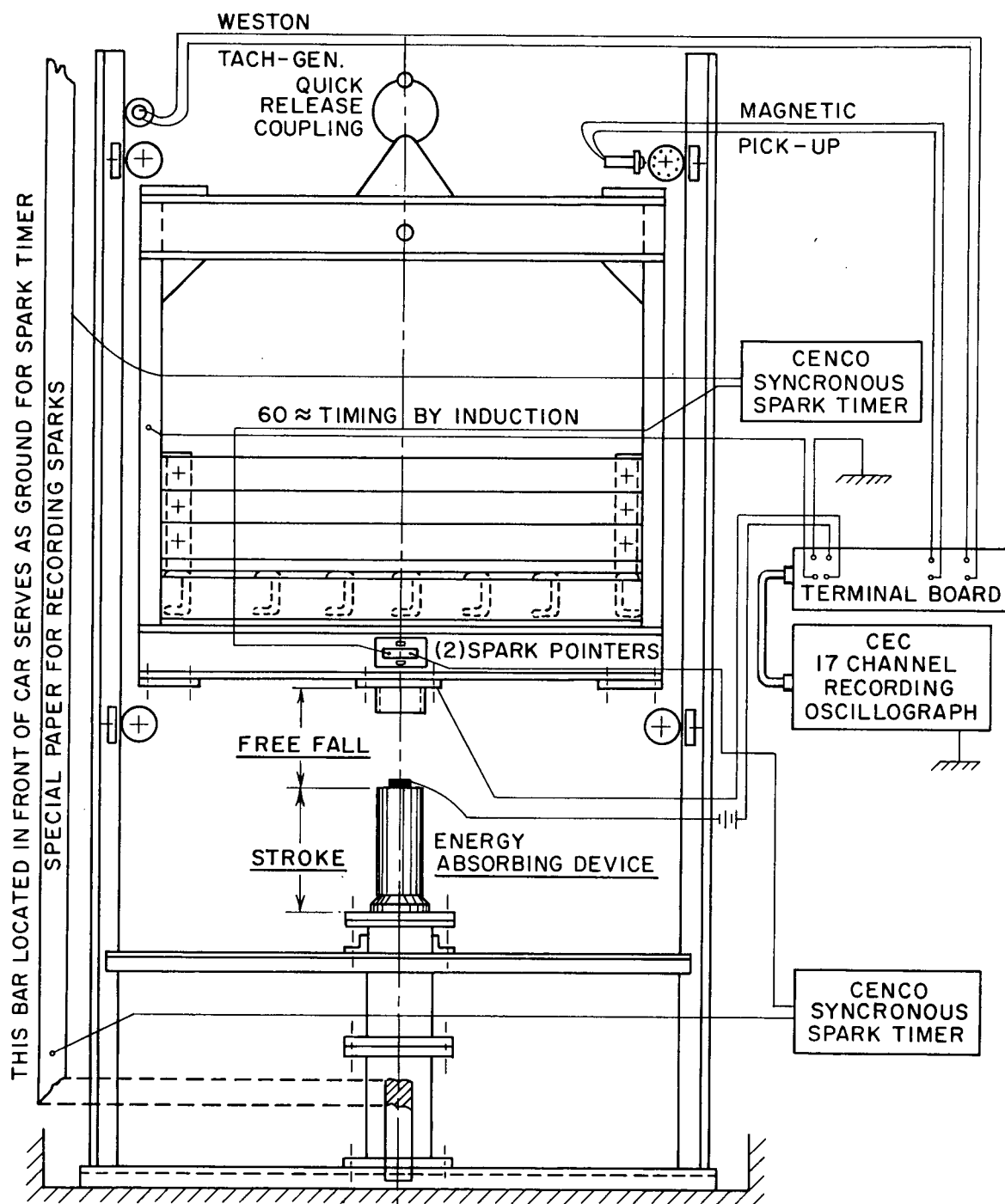
Figure 4.5. Otis Test Set Up
