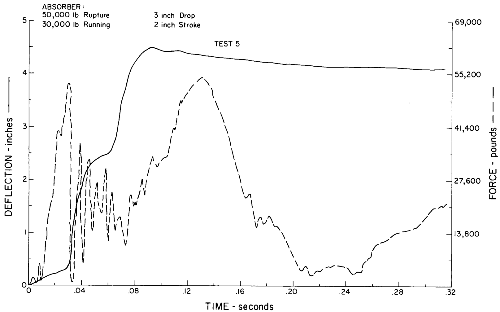
Figure 5.11. Force-Time and Deflection-Time Record for Test 5, Series No. 1
