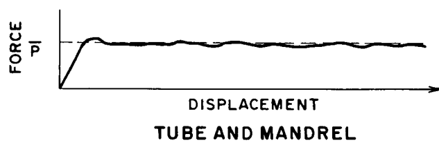
Figure 3.5. Force-Deflection Curve for Tube and Mandrel Energy Absorber
