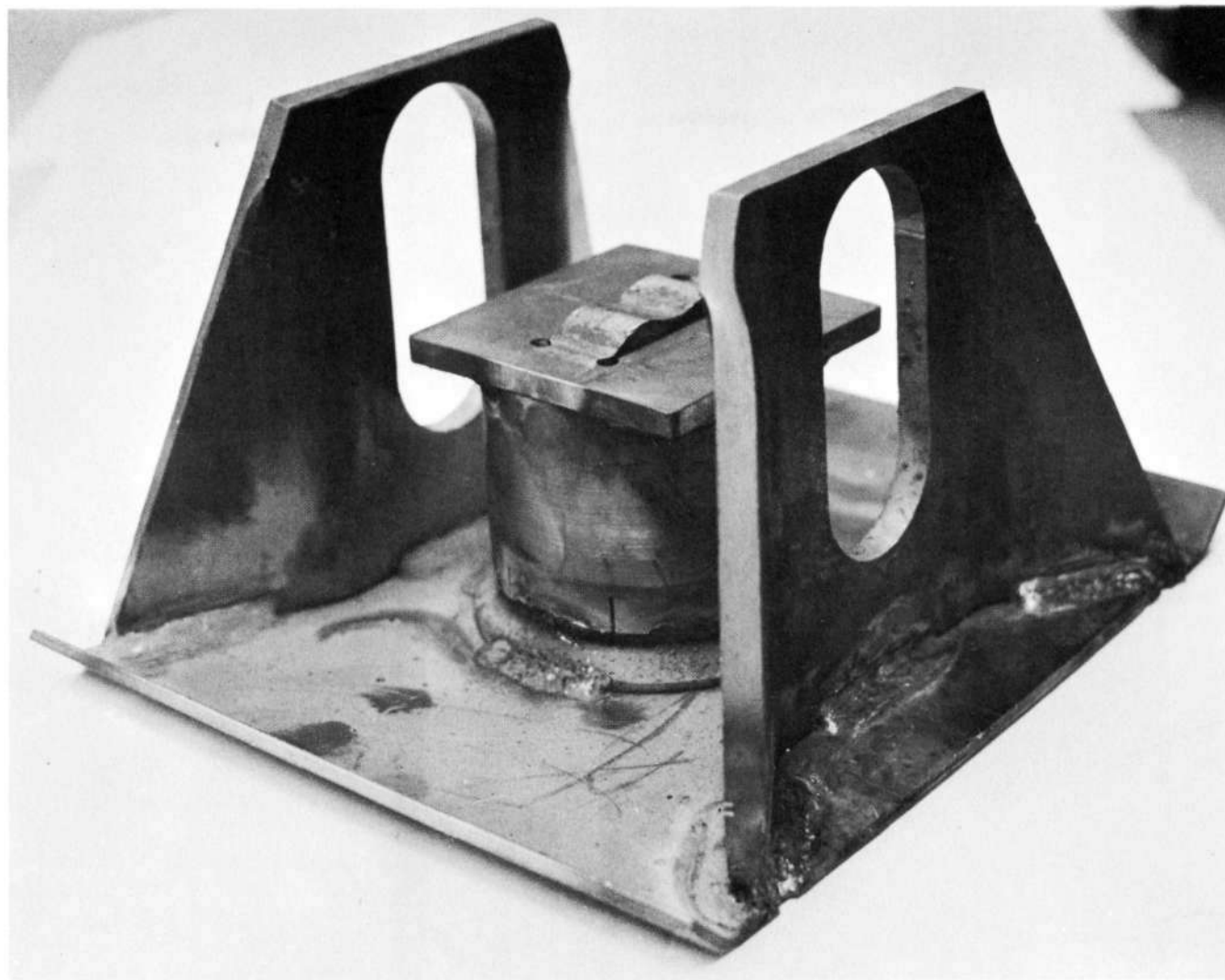
Figure 5.19. Photo of Homan Prototype Energy Absorbing Sand Shoe
