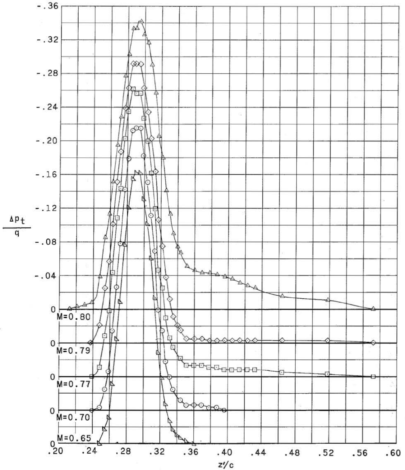
Figure 10.- Wake profiles for supercritical airfoil. \alpha = 0^\circ .
