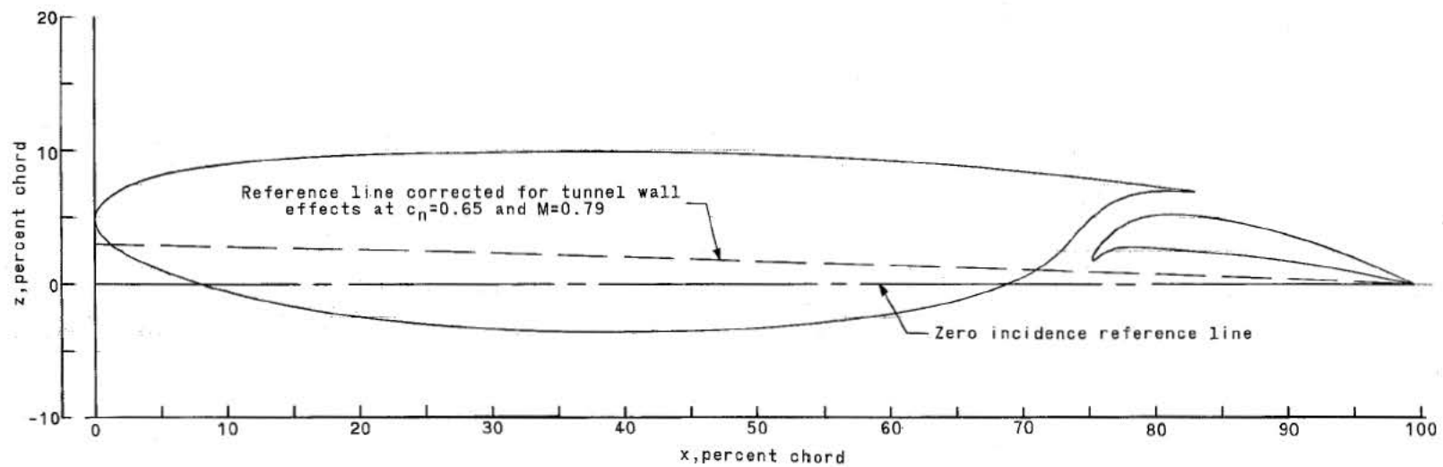
(a) Supercritical airfoil.
