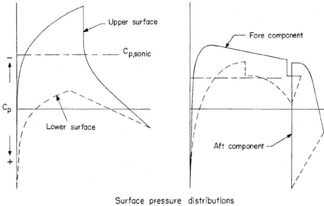
NACA 64A-series airfoil, M=0.69
