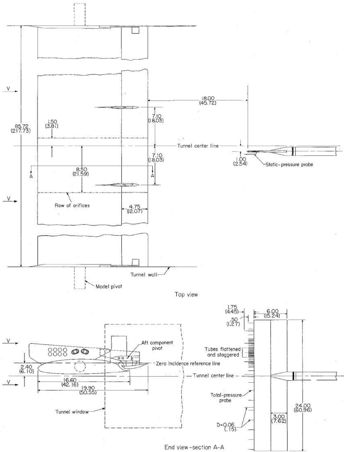
Figure 3.- Two-view drawing of apparatus. (All dimensions are inches (centimeters in parentheses).)
