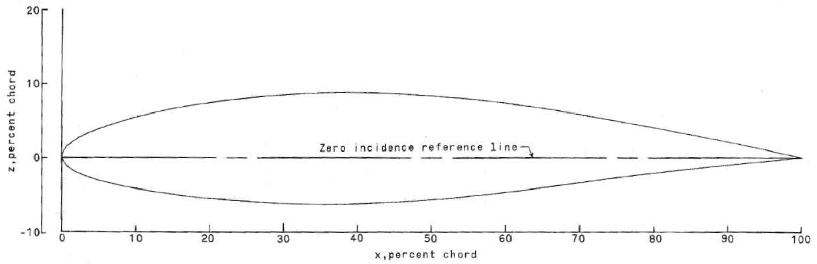
(b) NACA 64 2 A215 airfoil.
