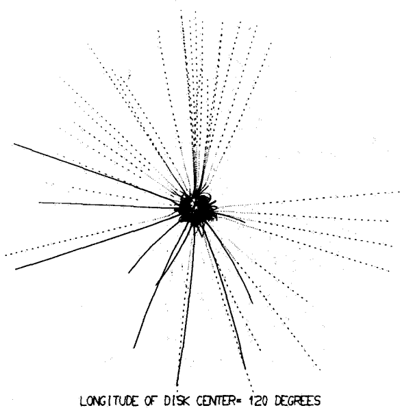
Figure 3. Coronal magnetic fields calculated out to a distance of 17 r_{\odot} . The calculations are based on the same material as figure 1. (a) View from the direction of the heliographic north pole. Zero longitude is towards the right. (b) View from the equatorial plane. North is upward, east to the left. Longitude 120^{\circ} of the central meridian corresponds to the time of the March 7, 1970, total solar eclipse.
