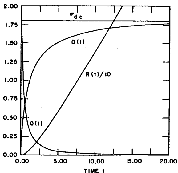
Fig. II-2. Numerical solution of Eq. (87), from Montgomery and Tappert. 45 Dimensionless units are: k/K_D , R/2K_D^2 , t[8\pi n_0 e c \epsilon^{1/2}]/\ell B . Notice that R increases linearly with t almost from the beginning.
