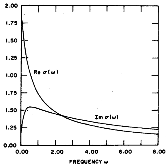
Fig. II-3. Real and imaginary parts of the conductivity from Eq. (113). The units of \sigma are n_0 e c \epsilon^{1/2}/\ell B .
