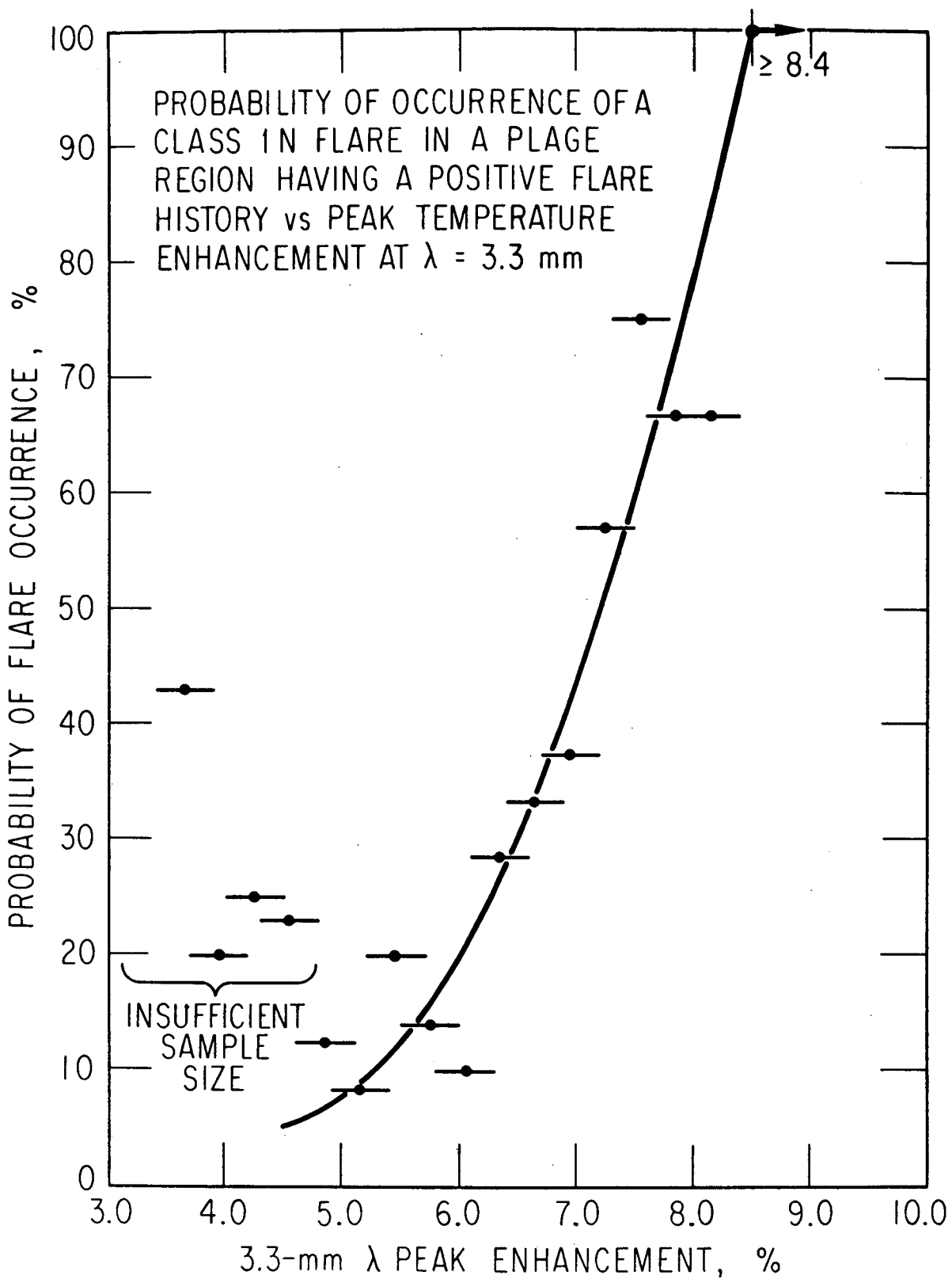
Fig. 8. Same as 7), but data applicable to class 1N flares in flare-prone plage regions.
