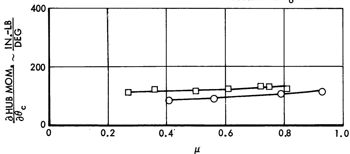
Figure 12. Rotor Hub and Shaft Moment Derivatives with Respect to \theta_c , Configuration 5
