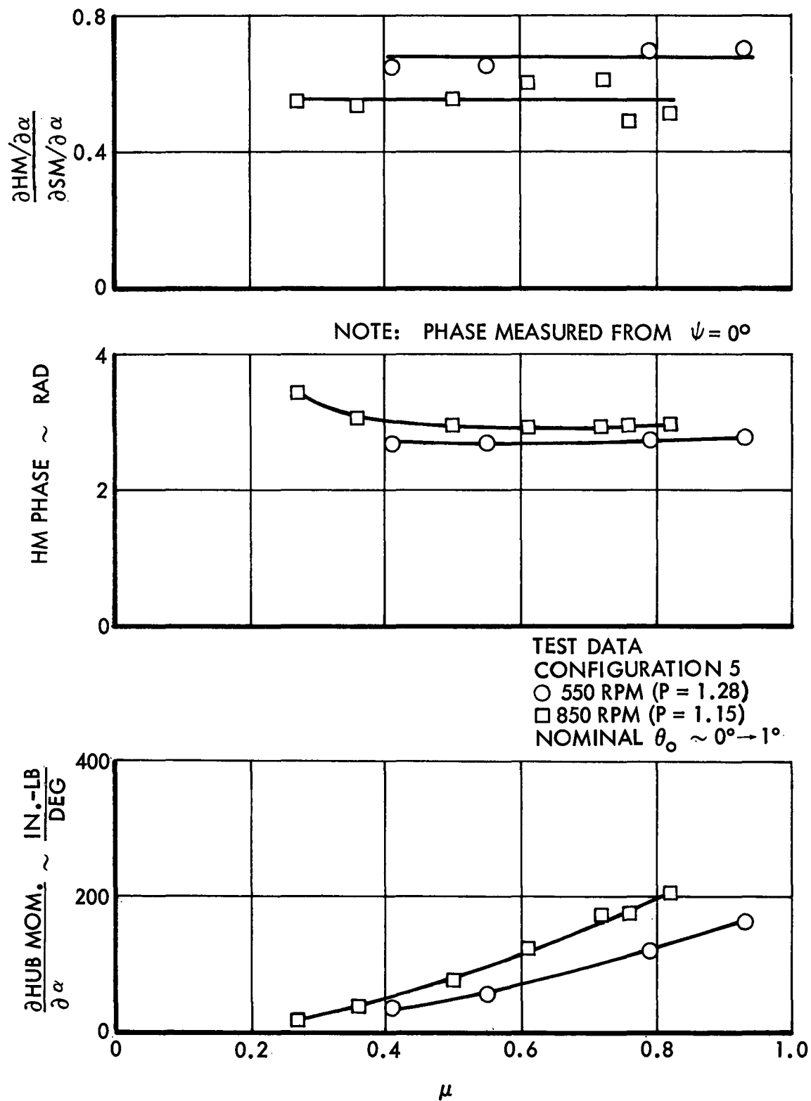
Figure 14. Rotor Hub and Shaft Moment Response Derivatives with Respect to \alpha , Configuration 5
