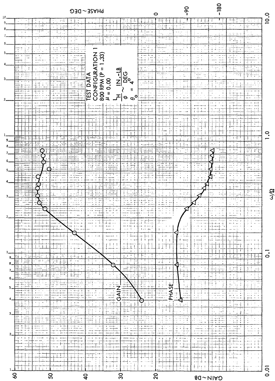
Figure C34. Rotor Hub Roll Moment Frequency Response to Shaft Roll, Configuration 1, \mu = 0.00 , 800 RPM ( \mu = 1.33 )
