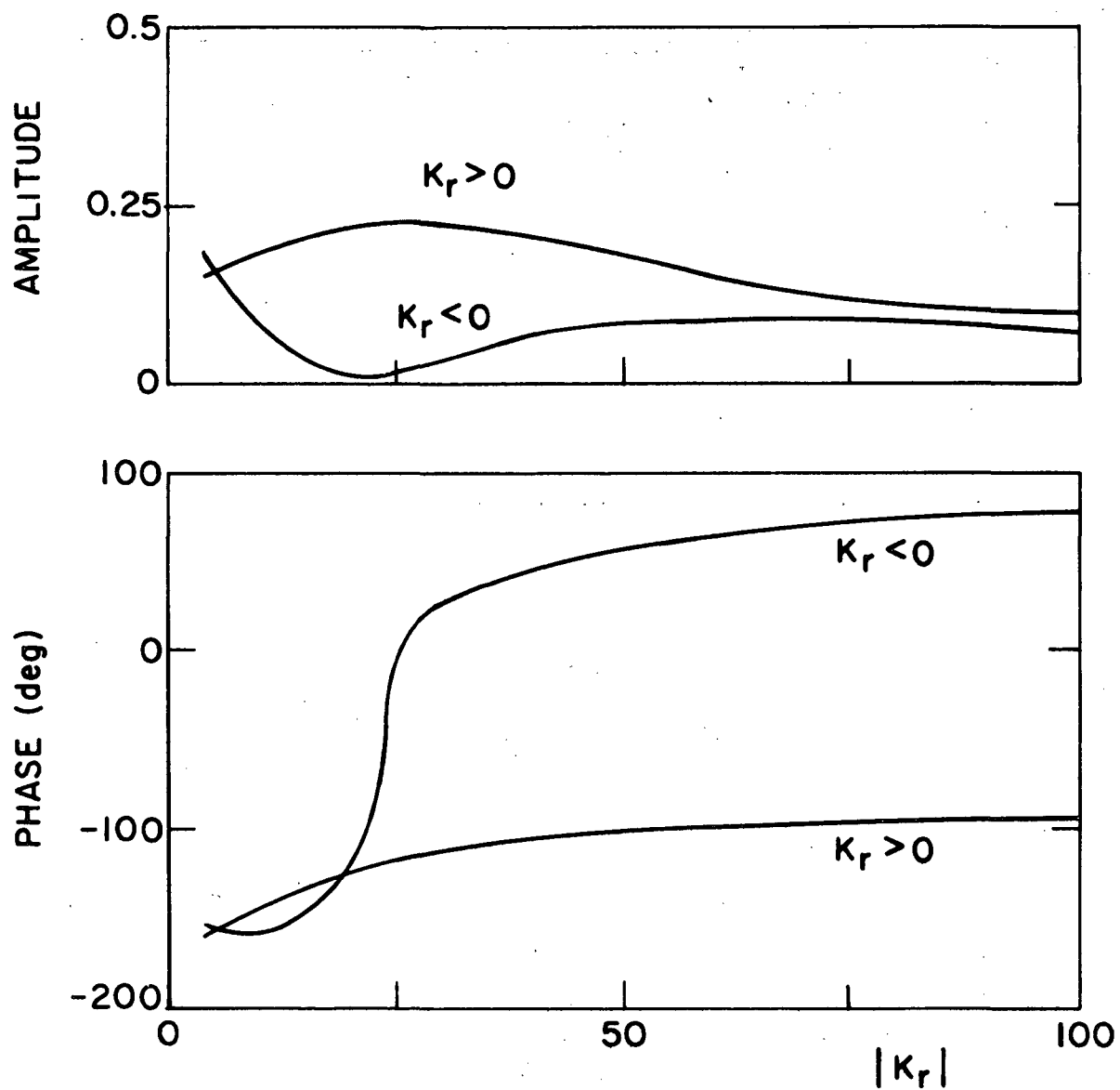
Fig. 4.10(b) Amplitude and phase of T_e \ln for the drift wave branch in Fig. 4.9 with v_{ez0} = 5(T_0/m_i)^{1/2} e \ln
