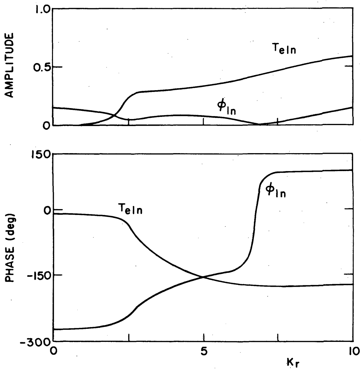
Fig. 4.8 Amplitude and phase of \phi_{\ln} and T_{e \ln} for the entropy wave branch in Fig. 4.6.
