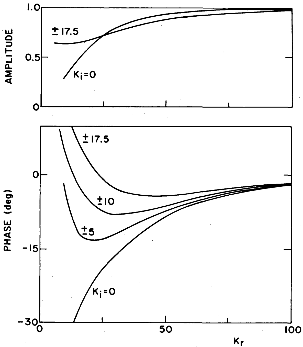
Fig. 4.7(a) Amplitude and phase of \phi_{ln} for the drift wave branch in Fig. 4.6.
