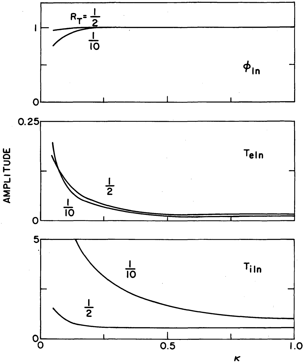
Fig. 5.3(a) Values of amplitude of the normalized variables \phi_{ln} , T_{eln} , and T_{ilm} for the conditions in Fig. 5.2 with R_T = 1/2, 1/10 .
