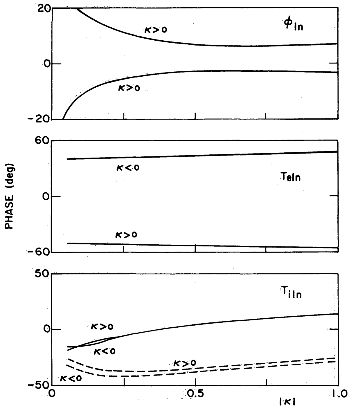
Fig. 5.5(b) Values of phase of the normalized variables \phi_{ln} , T_{eln} , and T_{iln} for the conditions in Fig. 5.5(a).
