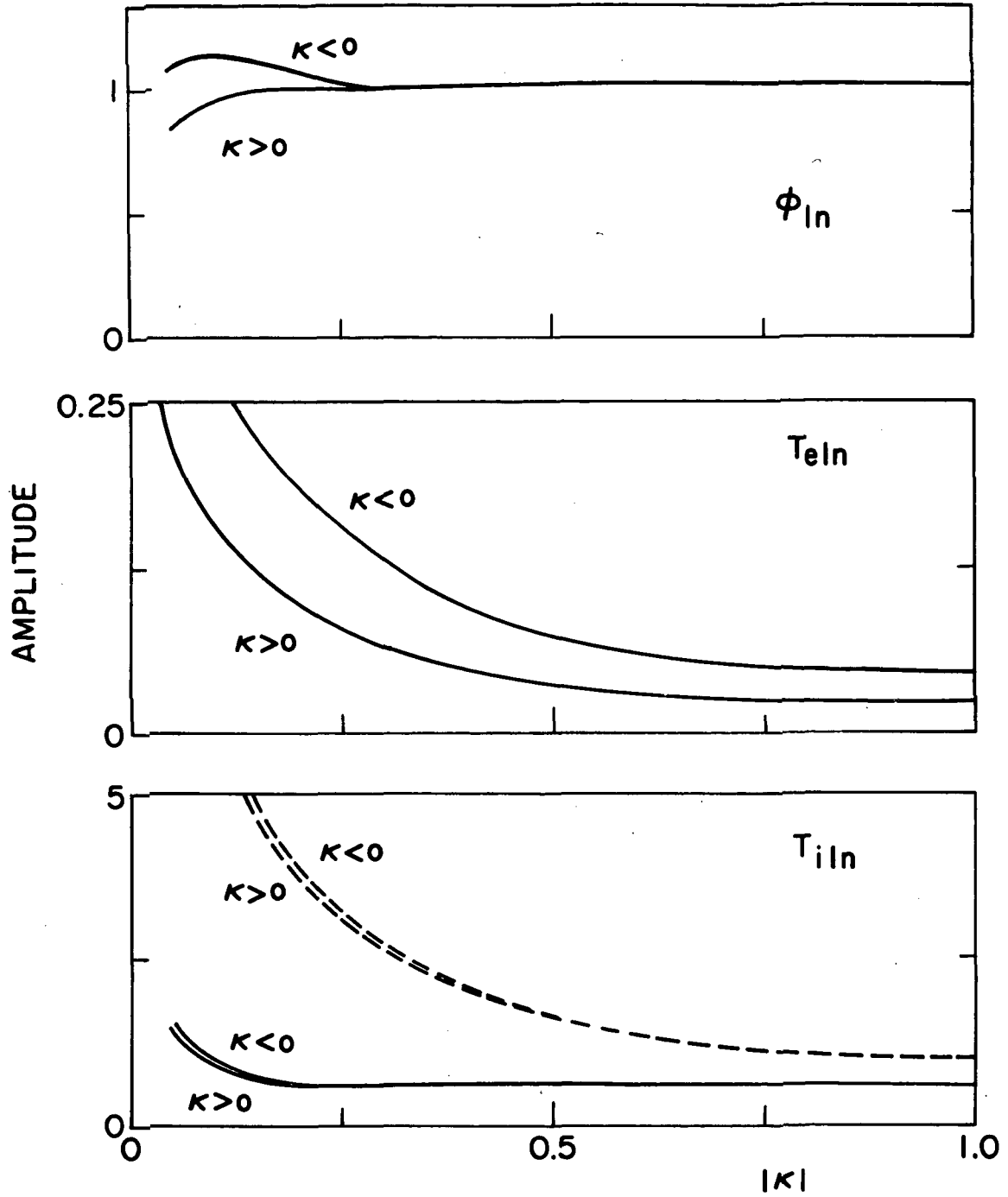
Fig. 5.5(a) Values of amplitude of the normalized variables \phi_{in} , T_{ein} , and T_{iin} for the ion-acoustic wave in Fig. 4.5 with v_{e0} = 4(T_{e0}/m_i)^{1/2} . —, R_T = 1/2 ; ----, R_T = 1/10 . Curves for R_T = 1/10 are omitted if they essentially coincide with R_T = 1/2 curves.
