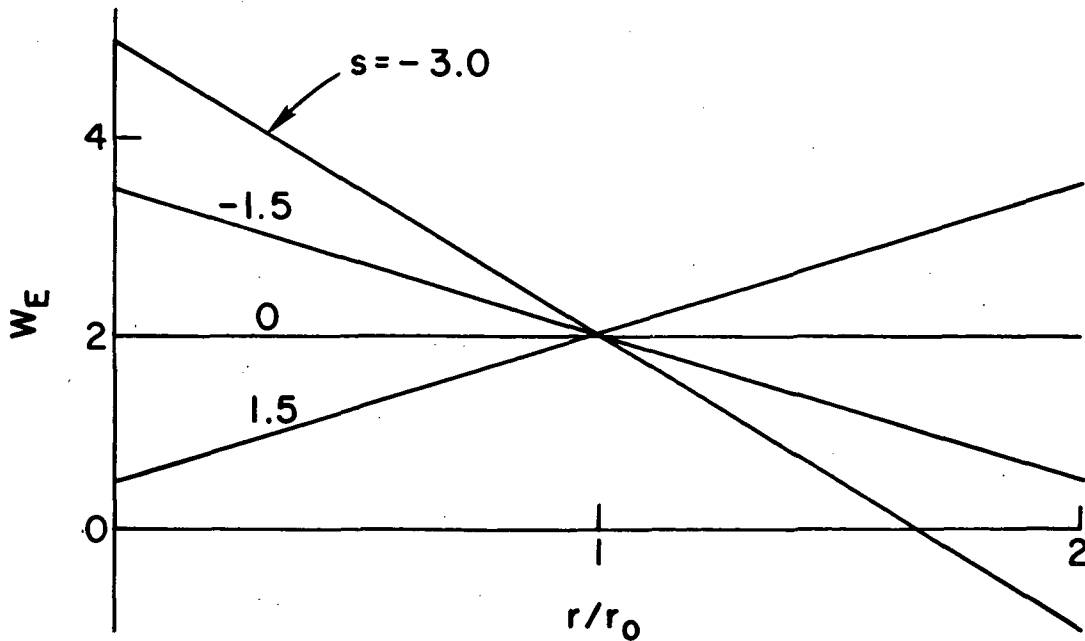
Fig. 3.5 Rotation frequency profile, W_E , due to the electric field, as given by Eq. (3.48).
