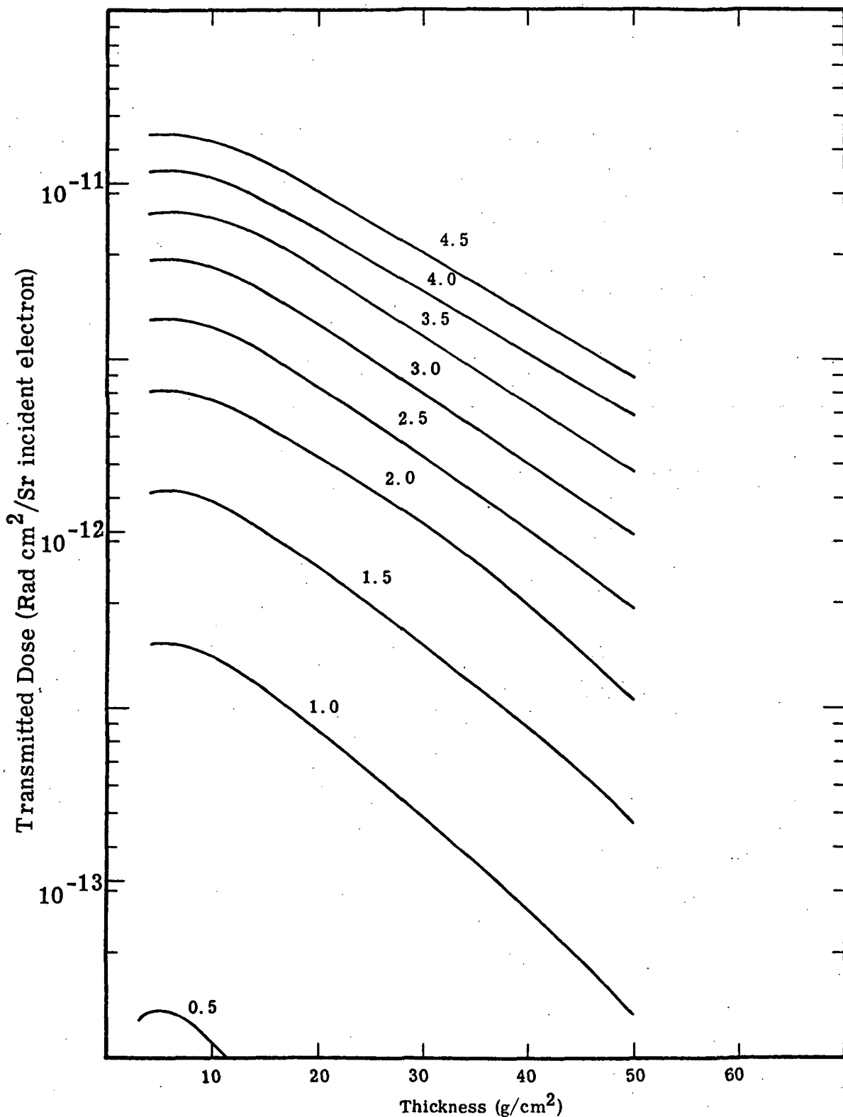
Figure 6.15. Bremsstrahlung tissue dose transmitted through Al shield caused by an isotropic flux of monoenergetic electrons incident on one side of the shield. Curves are normalized per incident electron. The incident electron kinetic energies are listed in MeV on the figure (Calculated from Eq. 6.47).
