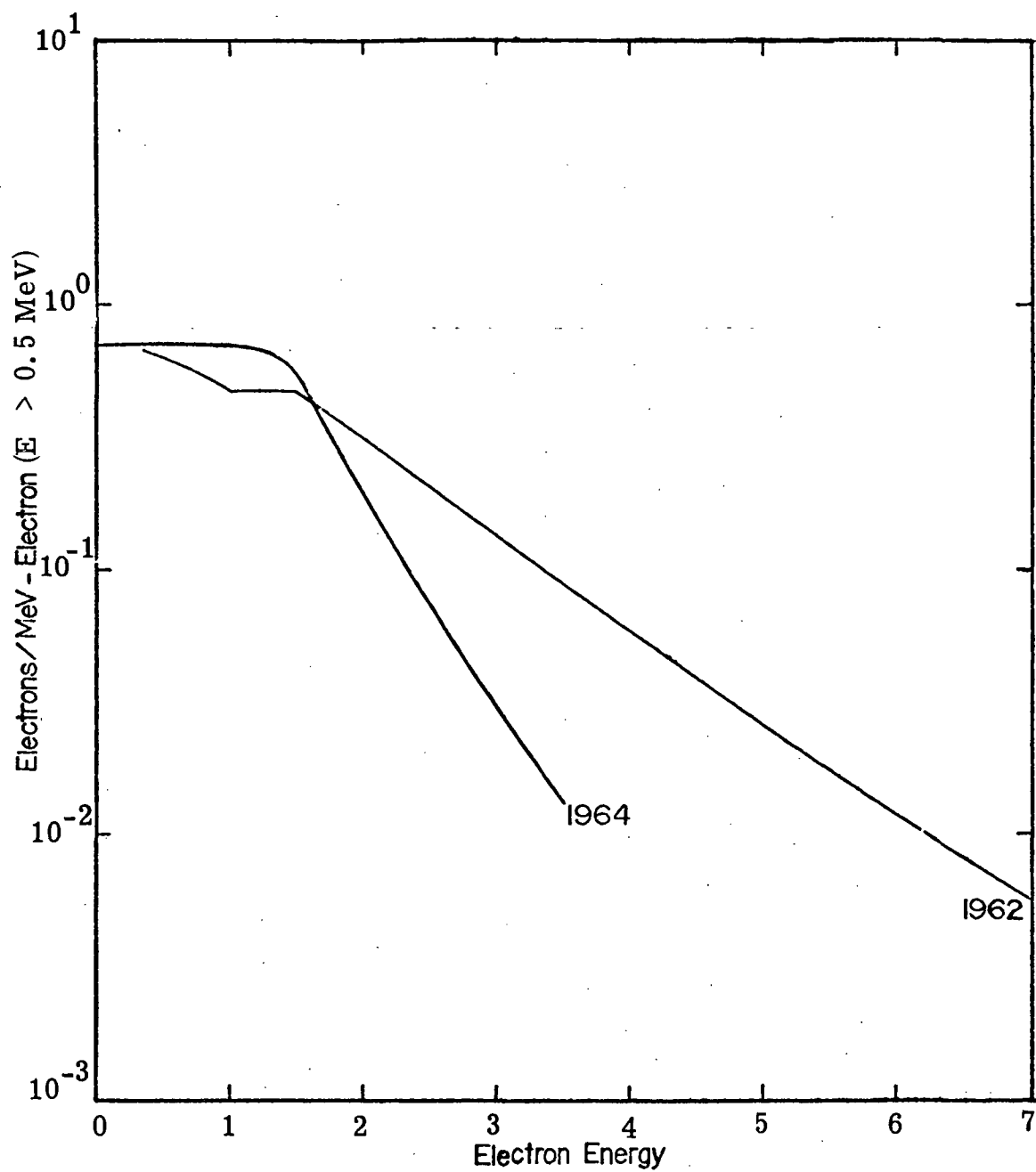
Figure 2.8. Electron energy spectrum at L = 1.2 measured two months after the Starfish event (1962) and two years later (1964)
