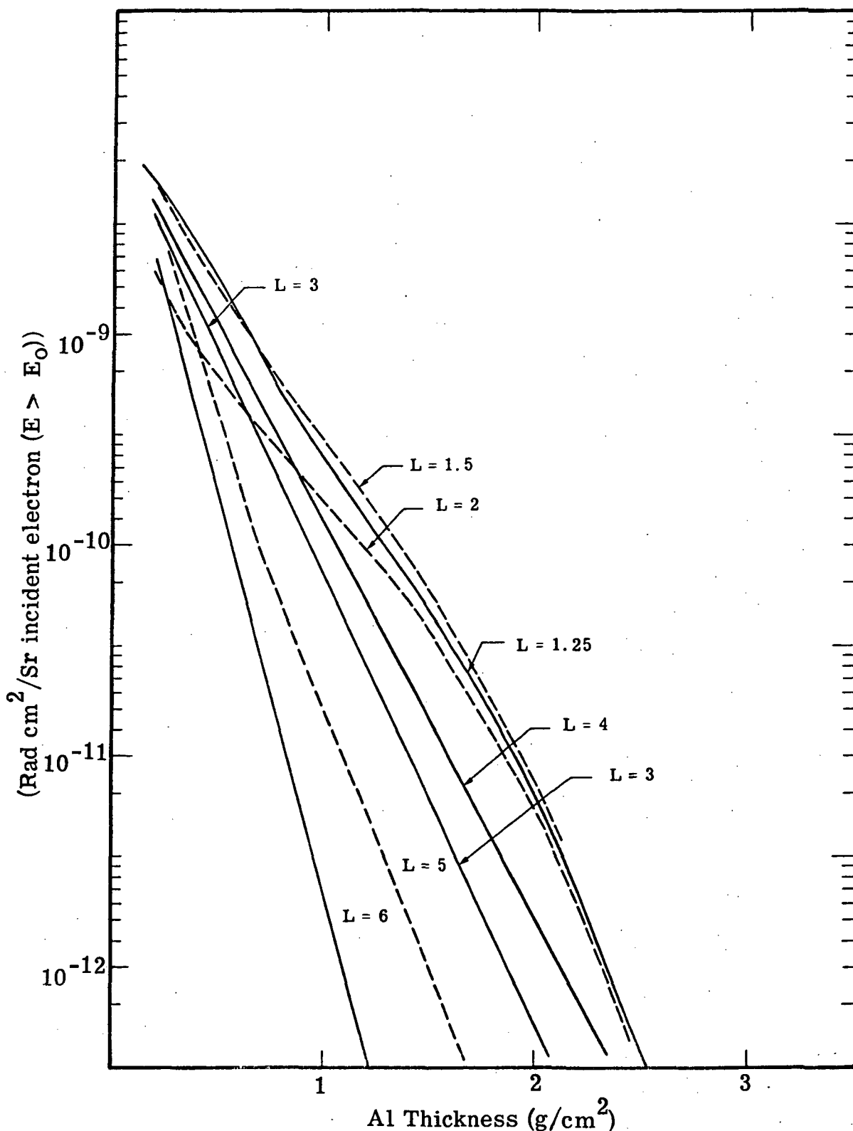
Figure 6.7. Transmitted tissue dose caused by isotropic flux of electrons incident on one side of a unit area of an Al shield. The electron energy spectra are given by Vette's AE2 electron environment. The L values associated with the various electron spectra are shown on the figure. The curves are normalized per unit incident electron. (N.B. The AE2 distribution is considered to be outdated by space scientists.)
