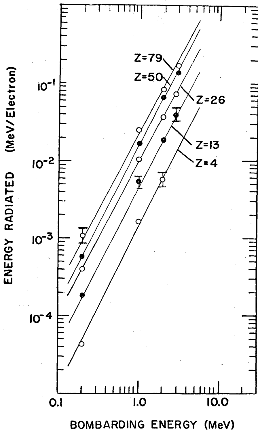
Figure 5.4. Energy radiated from thick targets of Be, Al, Fe, Sn, and Au as a function of bombarding energy, E . The respective lower cutoff photon energies for E = 0.2, 1.0, 2.0 , and 2.8 MeV. Experimental lower cutoffs are 36 keV, 50 keV, 133 keV, and 171 keV respectively. (From Ref. 28)
