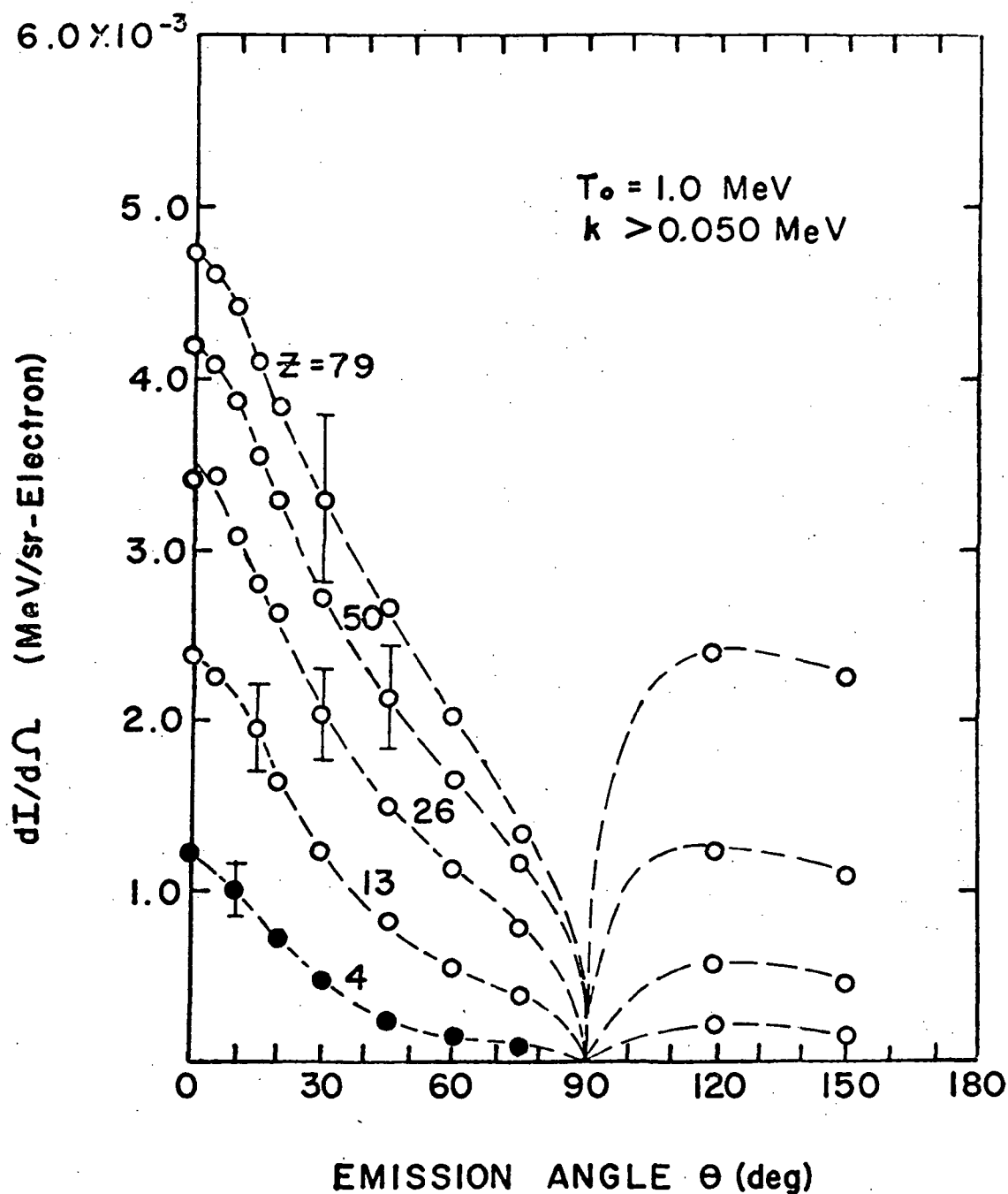
Figure 5.5. Angular distributions of bremsstrahlung intensities, integrated over photon energy, k > 0.050 MeV, for 1.0 MeV electrons on thick targets of Be, Al, Fe, Sn, and Au. (From Ref. 28)
