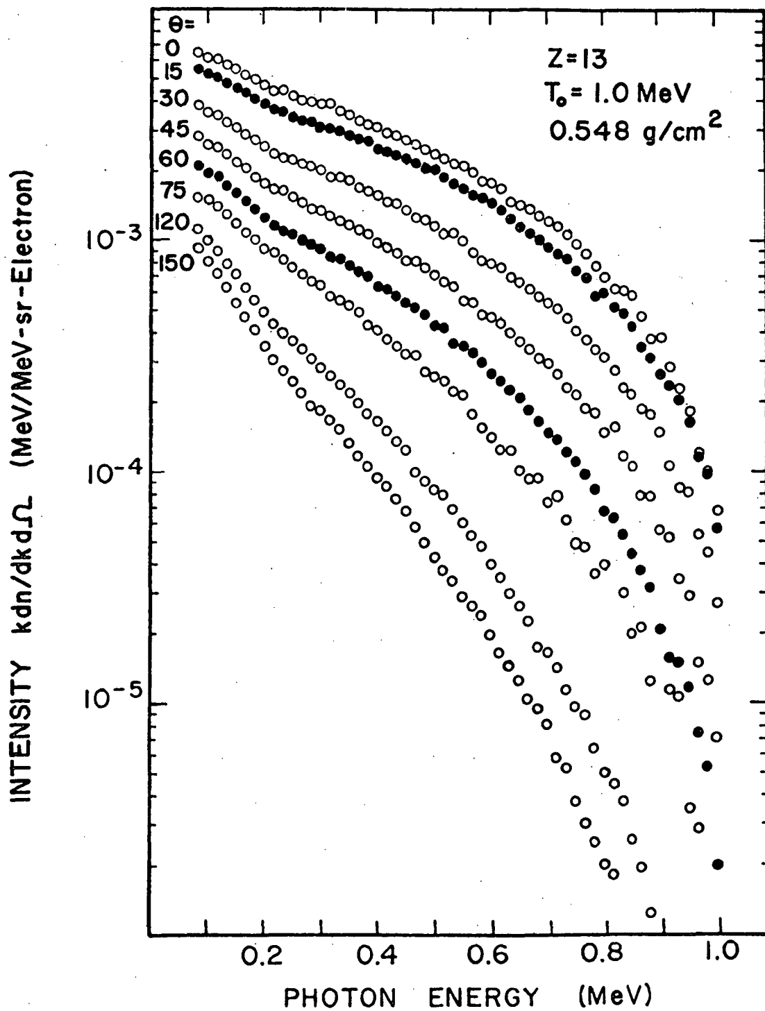
Figure 5.9. Bremsstrahlung differential intensity spectra for 1.0 MeV electrons on a thick Al target. (From Ref. 28)
