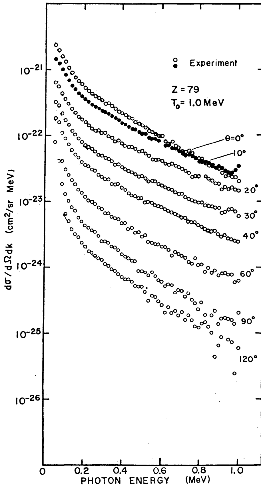
Figure 3.10. Bremsstrahlung differential cross sections for 1.0-MeV electrons on Au (From Ref. 22)
