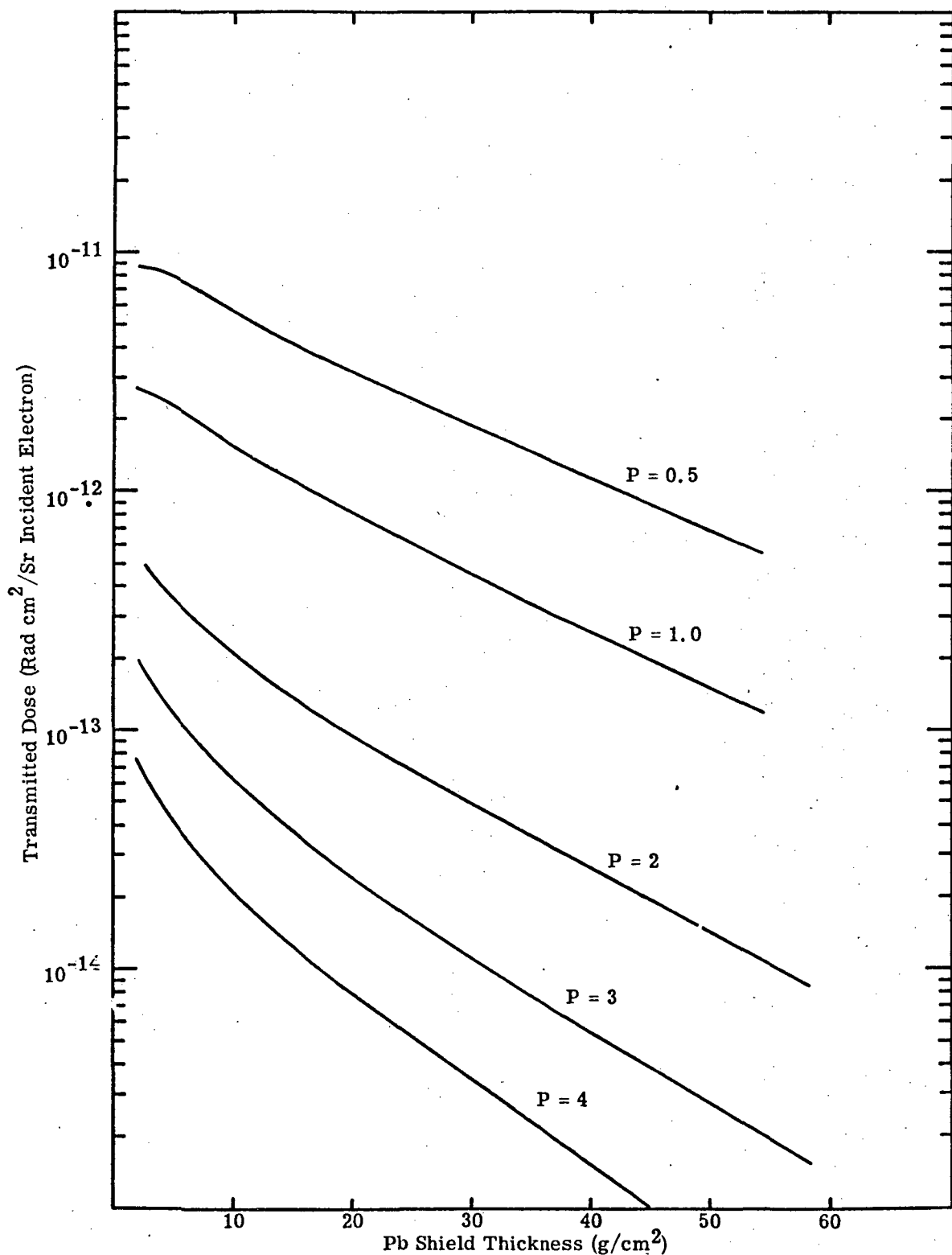
Figure 6.18. Bremsstrahlung tissue dose transmitted through a Pb shield caused by an isotropic flux of electrons incident on a unit area of one side of the shield. The electron energy spectra are given by N(E) = Pe^{-PE} . The values of P are listed in the figure.
