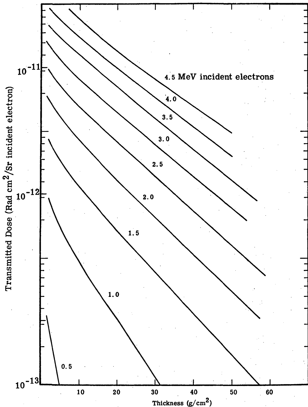
Figure 6.16. Bremsstrahlung tissue dose transmitted through a Pb shield caused by an isotropic flux of monoenergetic electrons incident on one side of a unit area of the shield. The curves are normalized per incident electron. The kinetic energies of the incident electron are listed on the figure.
