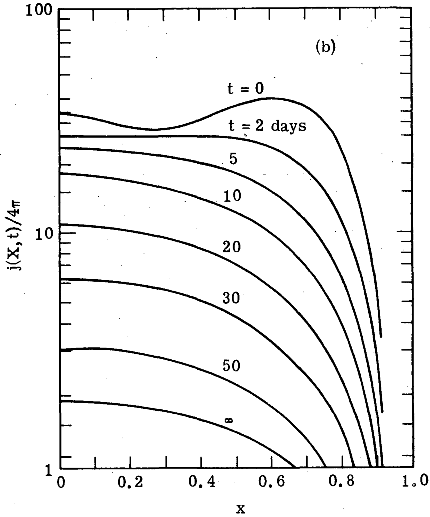
Figure 2.7. Decay of some initial particle fluxes to the steady state caused by pitch-angle diffusion. The flux is plotted as a function of the coordinate x = (1 - B_0/B)^{1/2} , where B_0 is the field intensity at the intersection of the L-surface in which the electron lies in the magnetic equatorial plane.
