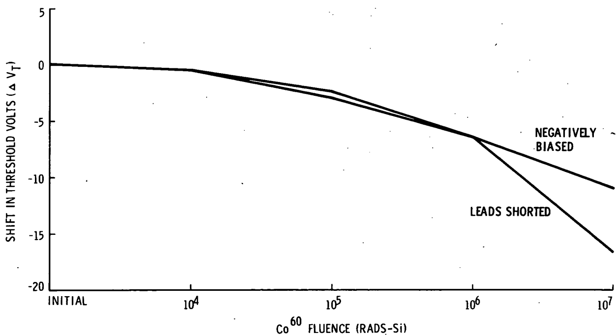
Fig. 4. The effect of \text{Co}^{60} gamma irradiation on unpassivated dual p-Channel MOSFETs.
