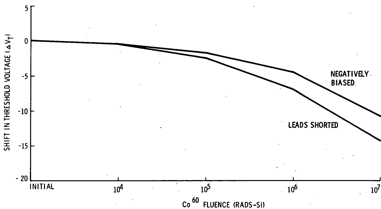
Fig. 3. The effect of \text{Co}^{60} gamma irradiation on passivated dual p-Channel MOSFETs.
