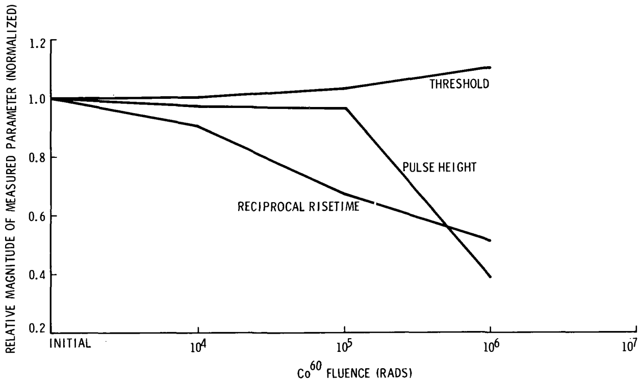
Fig. 1. The effect of \text{Co}^{60} gamma irradiation on micropower circuit, ICB-9002. Threshold, pulse height, and reciprocal rise time vs radiation fluence.
