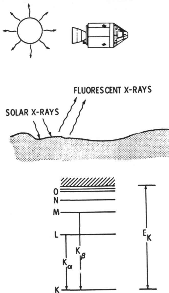
Figure 1—X-ray fluorescence at lunar surface. Lower diagram shows the electron transitions giving rise to characteristic K X-ray spectra.
