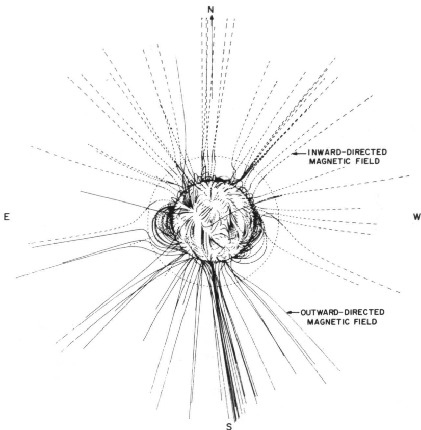
Figure 1—Model of the coronal magnetic field.
