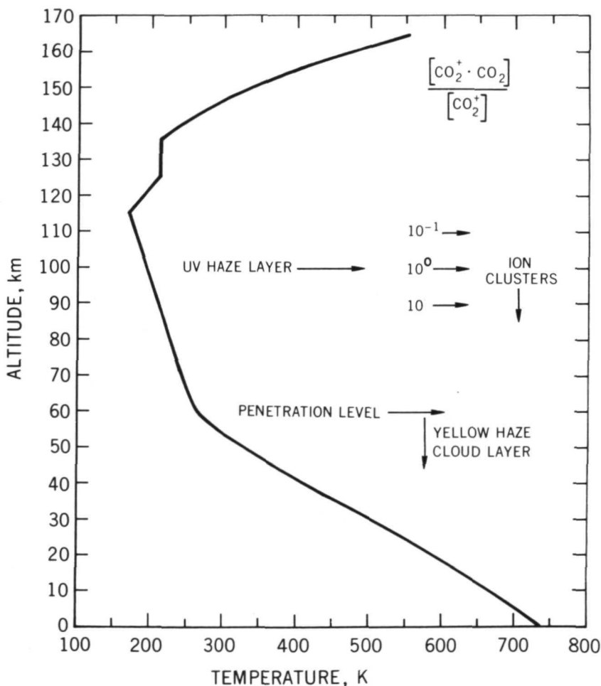
Figure 2—Altitude level of the Venus yellow cloud layer and ultraviolet haze layer in relation to the temperature distribution of the atmosphere and the ratio [\text{CO}_2^+ \cdot \text{CO}_2]/[\text{CO}_2^+] .
