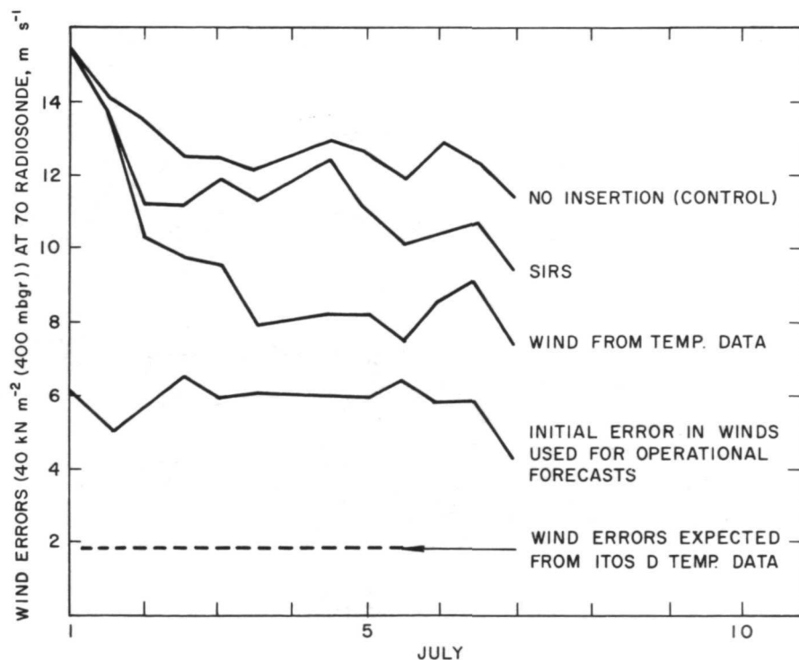
Figure 2—July 1970 experiment.
