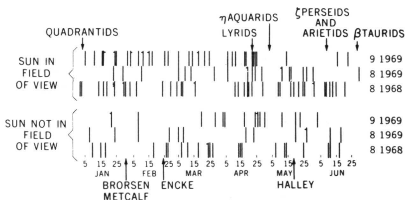
Figure 1—Pioneer 8 and 9 interplanetary dust detector counts.
