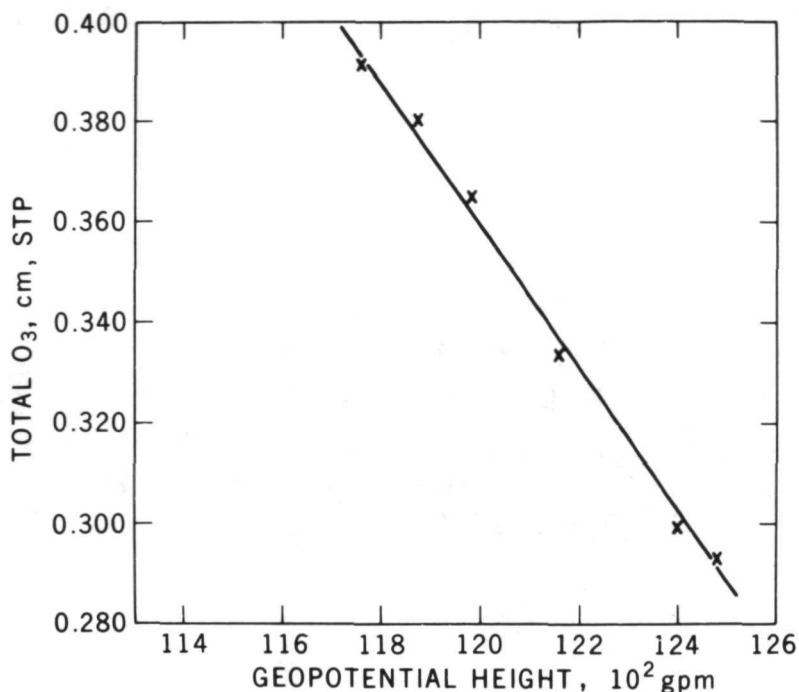
Figure 1—Total ozone versus 20\text{-kN-m}^{-2} (200-mbar) geopotential heights.
