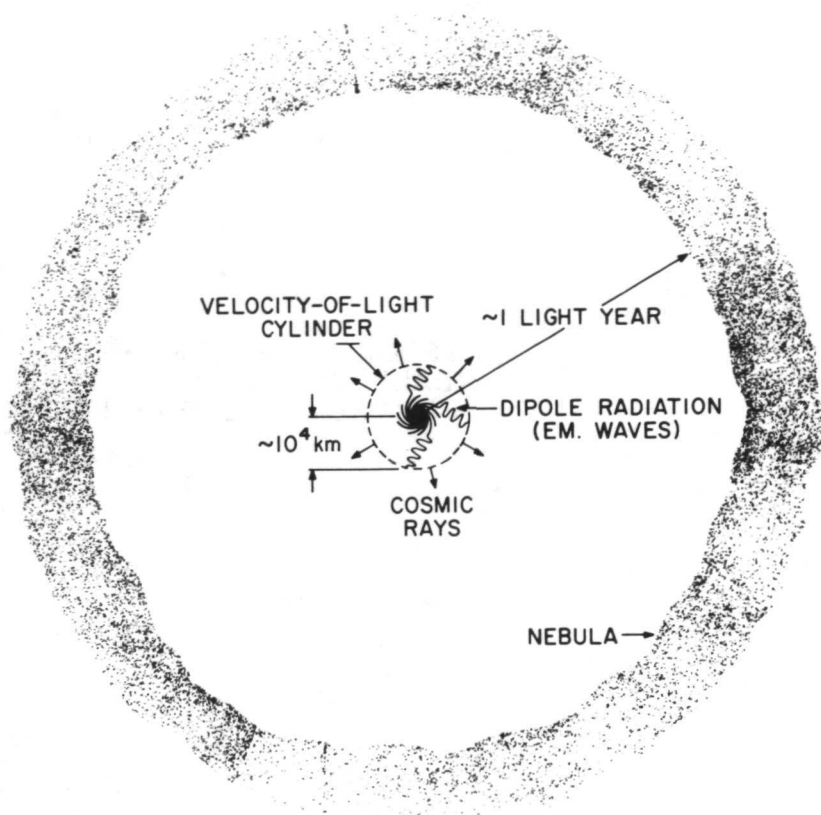
Figure 2—Pulsar environment.
