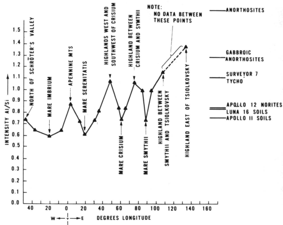
Figure 2—Plot of Al/Si intensity ratios along a northerly ground track.
