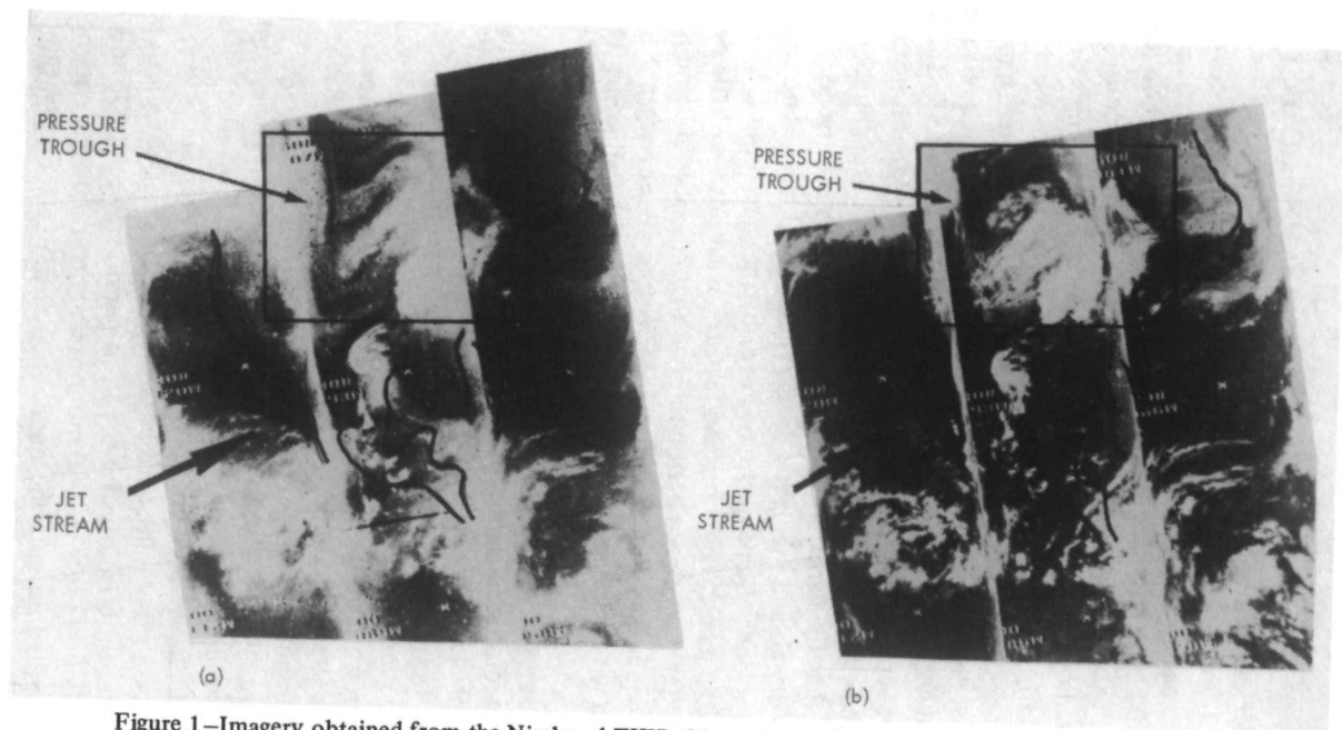
Figure 1—Imagery obtained from the Nimbus 4 THIR, May 14, 1970. (a) 6.7- \mu m wavelength observations. (b) 11.5- \mu m wavelength observations.
