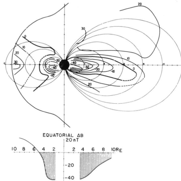
(a) Observed by OGO's 3 and 5, noon-midnight sectors, K_p = 0 to 1.
