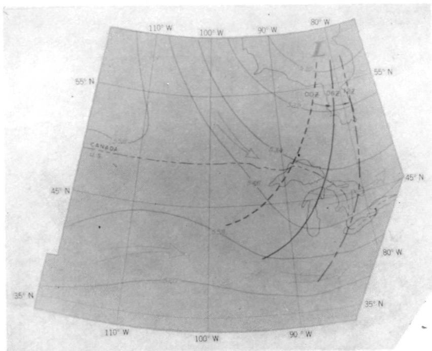
Figure 2—Motion of 50\text{-kN-m}^{-2} (500-mbar) flow at 0600 GMT, October 17, 1969.
