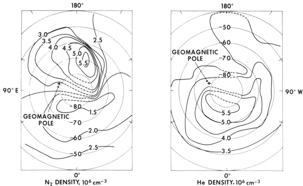
Figure 2—Contours of observed constant N 2 and helium densities plotted on a geographical latitude-longitude grid. Densities are extrapolated to 450 km.
