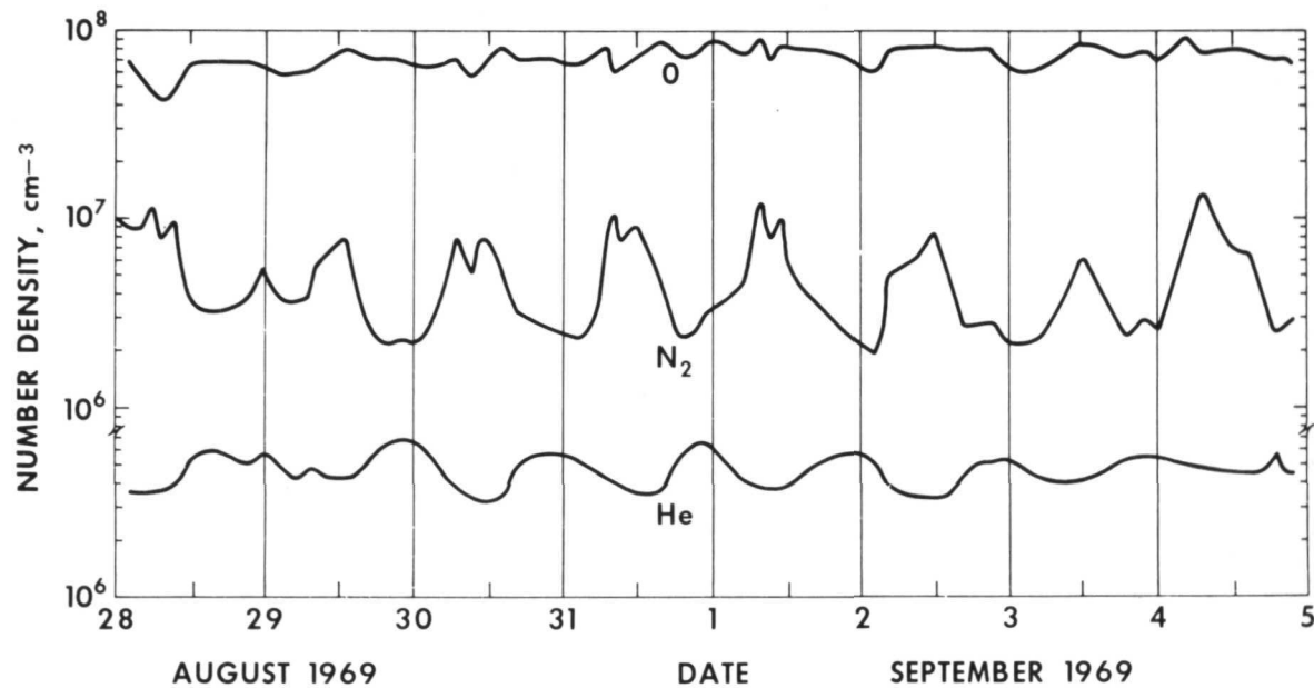
Figure 1—Gas densities at 430-km altitude as observed by the OGO 6 satellite near the South Pole.
