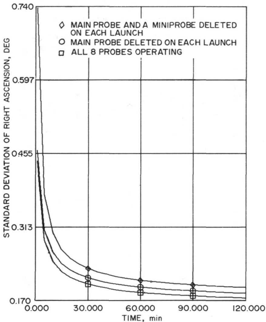
Figure 3—Standard deviation of right ascension as a function of time. A priori standard deviation is 10^\circ .
