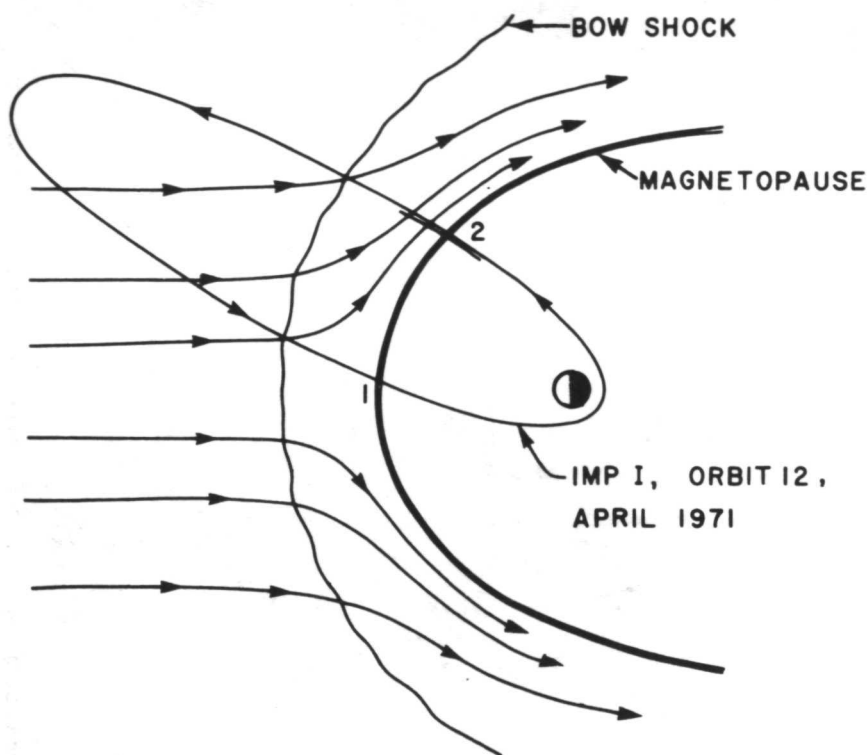
Figure 2—Satellite crossing of the magnetosphere.
