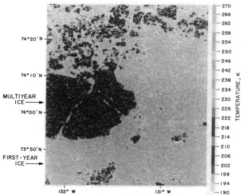
Figure 1—Passive microwave image of Arctic sea ice ( \lambda=1.55 cm) taken on a clear day from a NASA aircraft, March 15, 1971.
