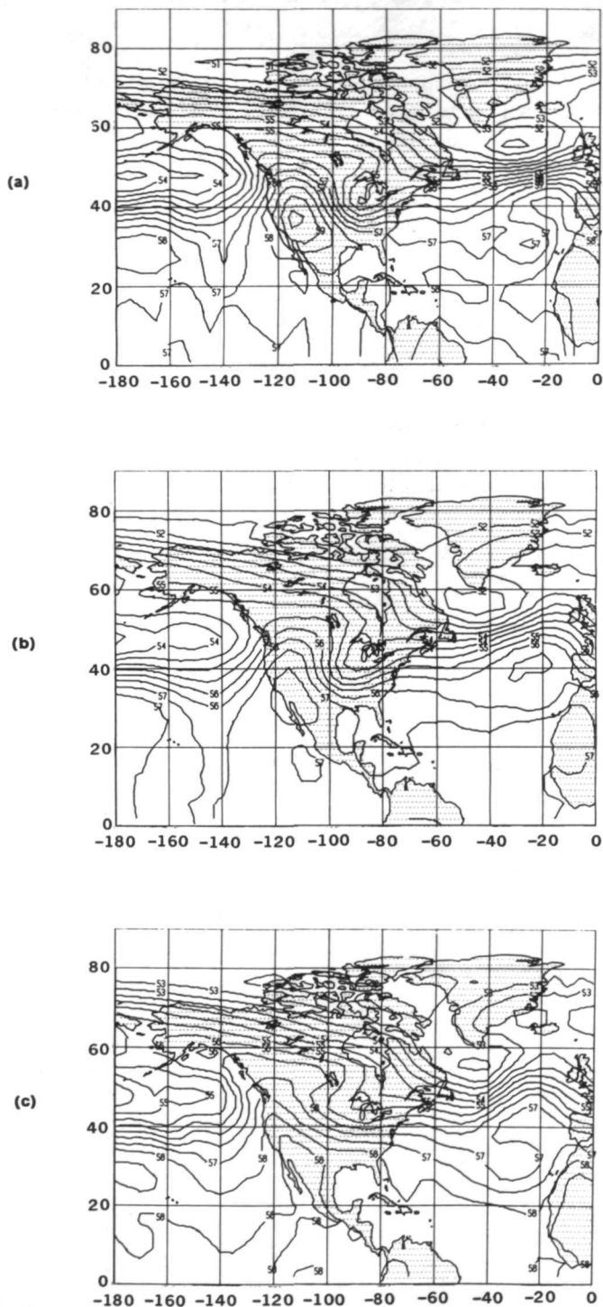
Figure 1—Comparison of 50-kN-m -2 (500-mbar) geopotential height analyses: (a) NMC observation; (b) Five-level GISS model; (c) Two-level UCLA model.
