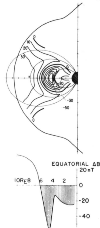
(b) Hoffman-Bracken (Ref. 1) quiettime ring current model.
