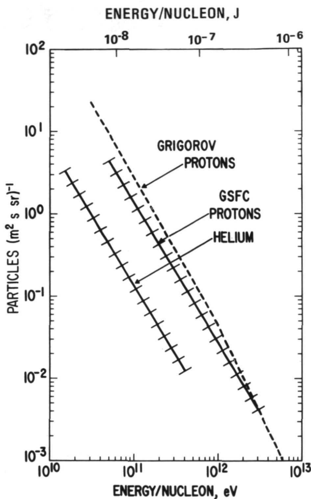
Figure 4—Integral spectra.
