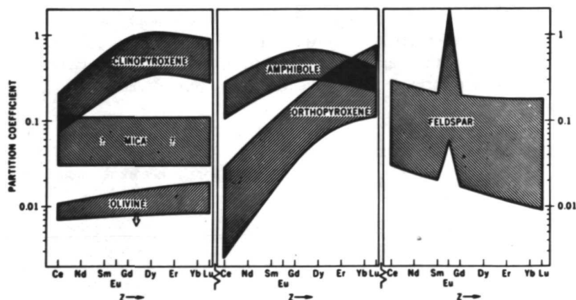
Figure 2—Mineral/liquid partition coefficients for rare Earth elements.
