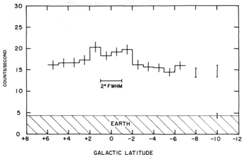
Figure 2—Counting rate as a function of galactic latitude.
