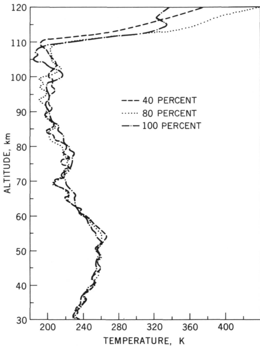
Figure 1—Temperature profiles of upper atmosphere obtained during the solar eclipse.
