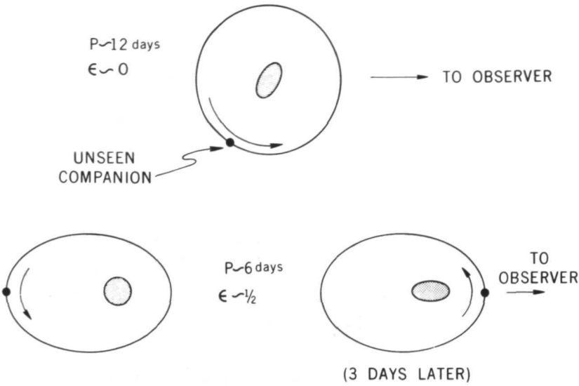
Figure 3—Two possible models of \beta Cephei.
