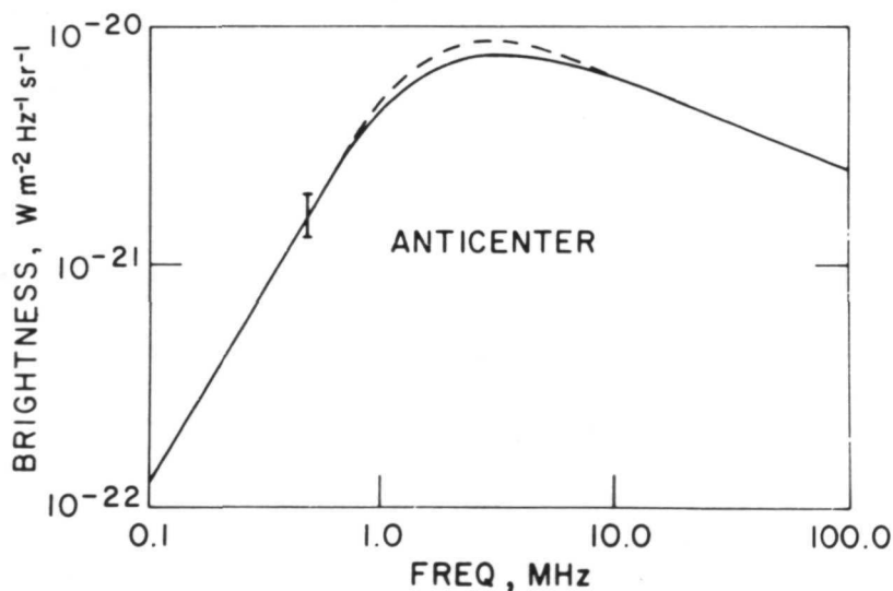
Figure 2—Brightness as a function of frequency for the model (solid line) and the RAE disk component (dashed line).
