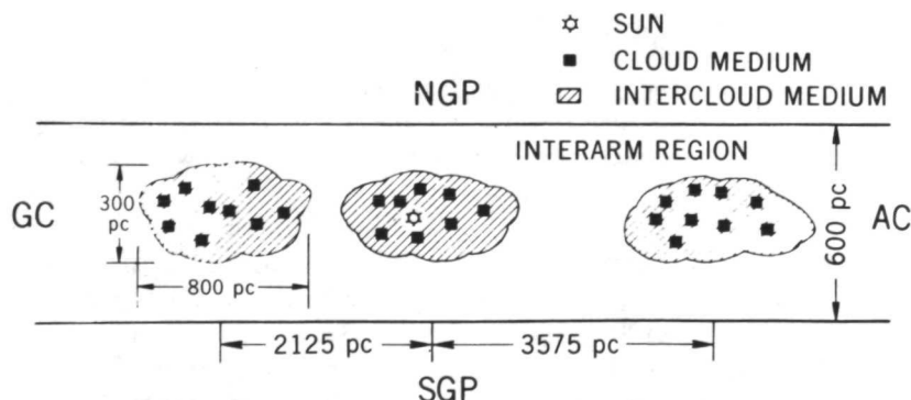
Figure 1—Geometry of the model of the interstellar medium.
