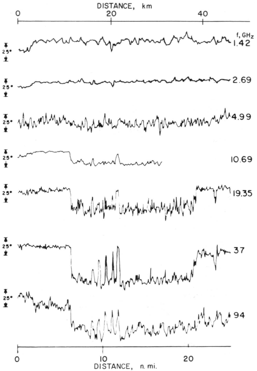
Figure 2—Multifrequency view of large multiyear ice floe.
