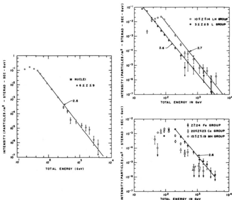
Figure 3—Energy spectra.
