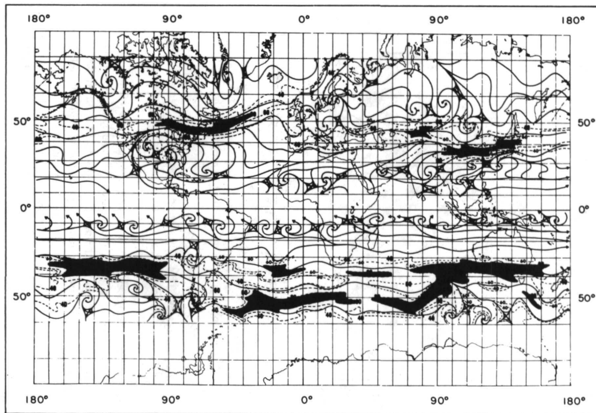
Figure 2—Geostrophic winds for 20\text{-kN-m}^{-2} (200-mbar), derived from total ozone data, IRIS, July 1969.
