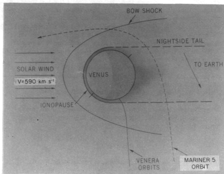
Figure 2—Solar-wind interaction model.
