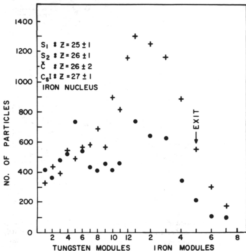
Figure 2—States of two iron nuclei as they pass through the modules. +: 0.5 \mu J (3000 GeV) nucleus; •: 69 \pm 11 nJ (430 \pm 70 GeV) nucleus.
