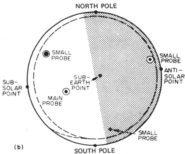
Figure 1—Position of probes on Venus surface.
