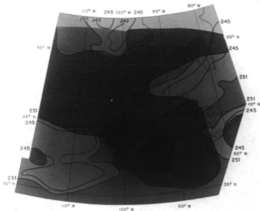
Figure 3—Vertical-motion results as interpolated to the satellite observation times of 0600 GMT.
