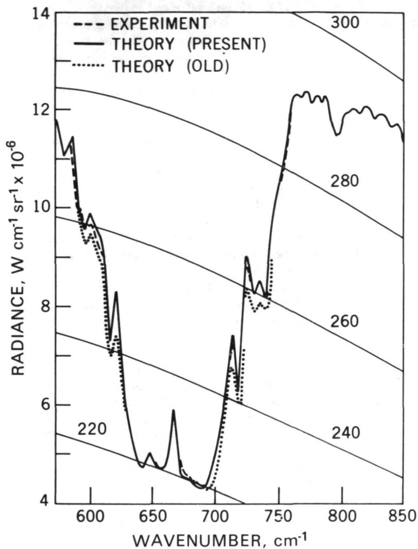
Figure 1—Earth radiance spectrum as determined by theory and as observed by the Nimbus 3 satellite over Brownsville, Tex.
