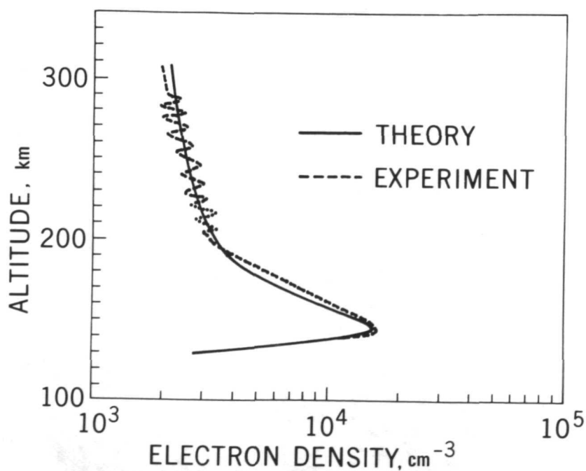
Figure 3—Nightside ionosphere model.
