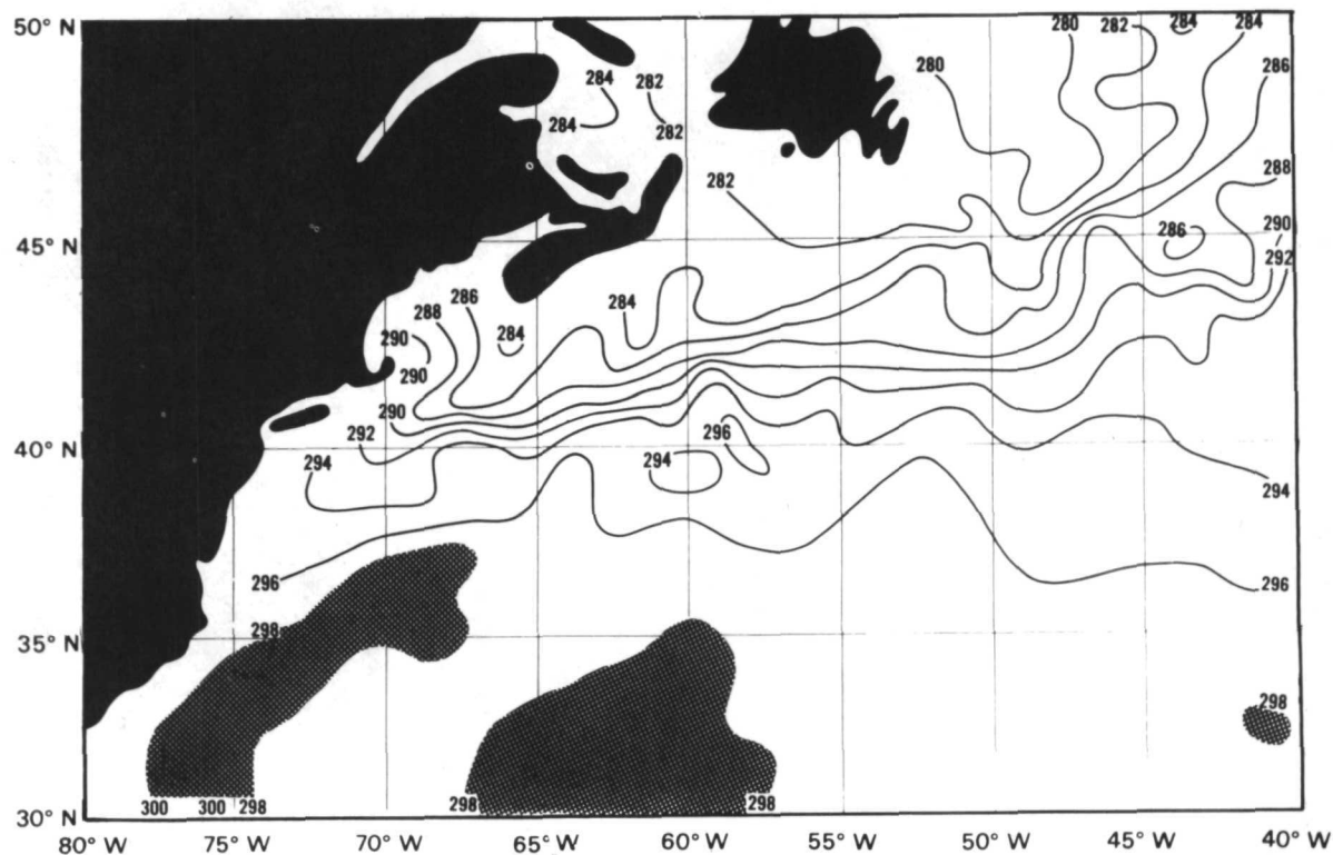
Figure 3—Sea surface temperature map.
