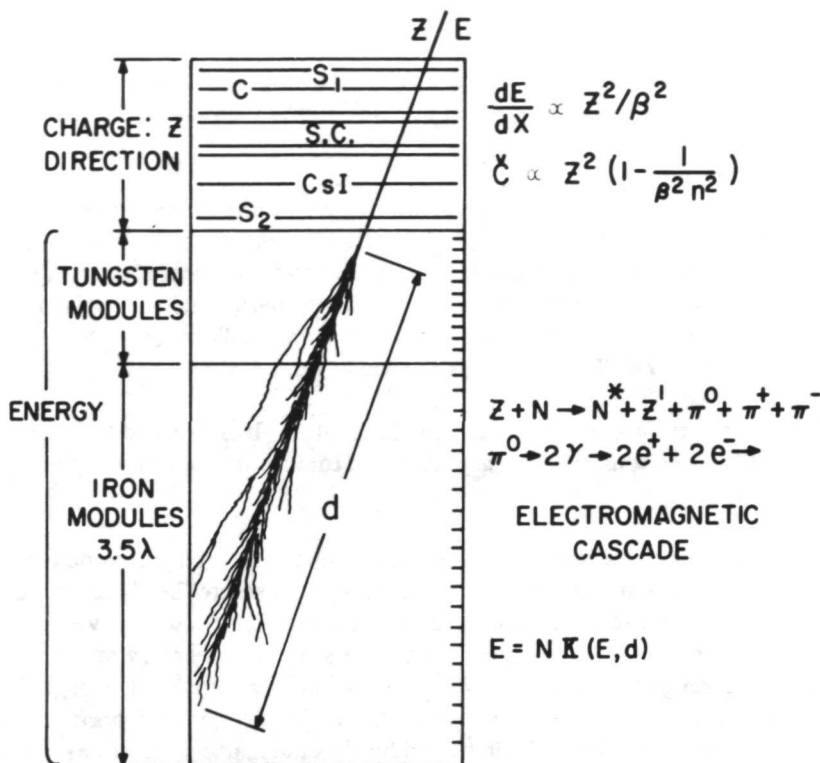
Figure 1—Diagram of instrument designed to identify particles and to measure their energies.
