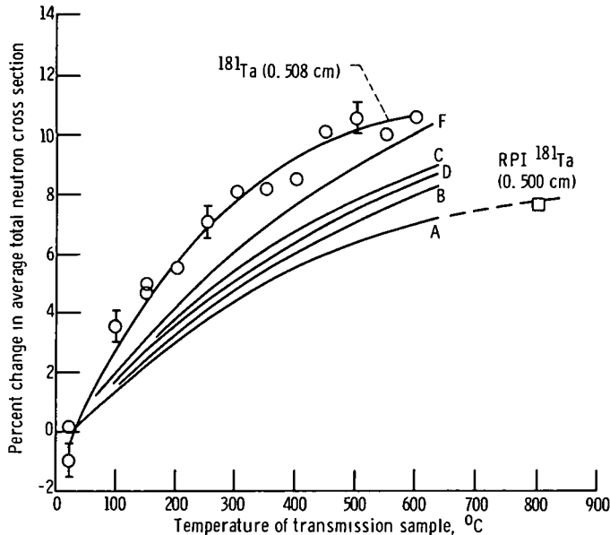
Figure 19. - Percentage change in average effective total cross section as function of temperature. Scandium-filtered beam of 2-keV neutrons; average level spacing, 4.3; ratio of average reduced scattering width to average level spacing, 1.8 \times 10^{-4} . Curves A, B, C, D, and F represent five different sets of mock data that have been Doppler broadened as a function of temperature. Point labeled RPI ^{181}\text{Ta} represents the RPI effective cross sections folded over the scandium-filtered spectrum. (Data from ref. 7.)
