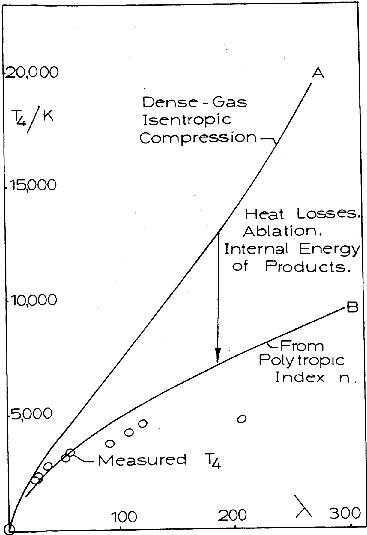
FIG. 13 Temperature Results at Peak Conditions
