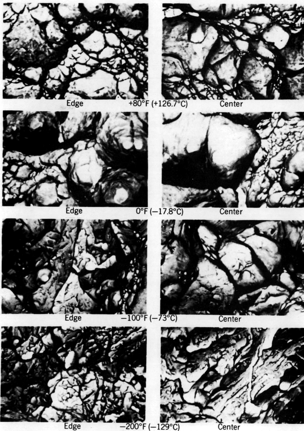
FIGURE 18 - SEM FRACTOGRAPHS OF 431 STAINLESS STEEL HARDENED AND TEMPERED V-NOTCH BAR TENSILE FRACTURES
