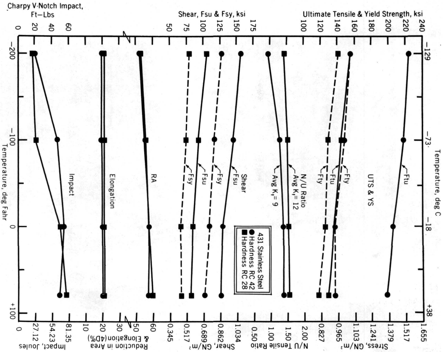
FIGURE 6 - LOW TEMPERATURE MECHANICAL PROPERTIES OF 431 STAINLESS STEEL BAR
