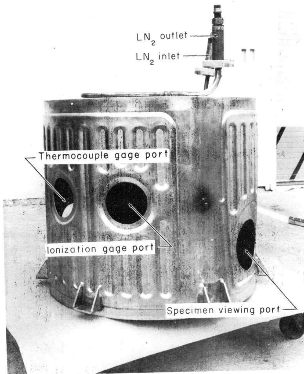
Figure 11.- Upper cryopanel.
