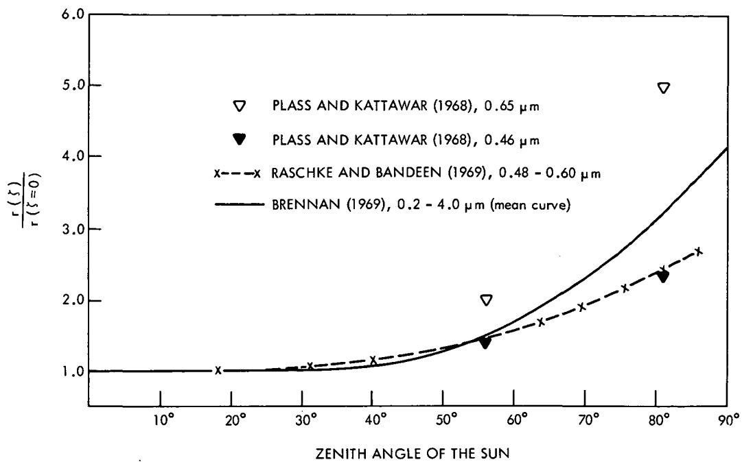
Figure B-8.—Ratio r(\xi)/r(\xi = 0) ; ocean model.
