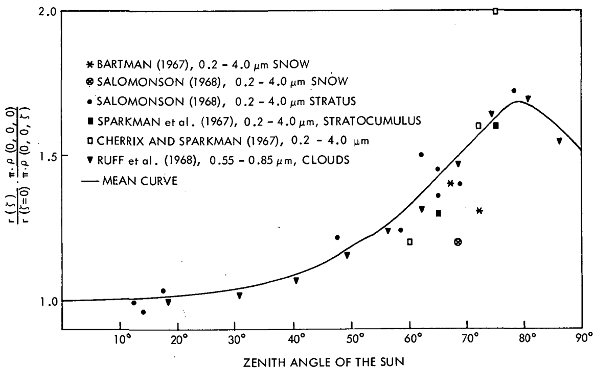
Figure B-2.—The function F_2(\xi) = [r(\xi)/r(\xi=0)] [\pi\rho(0, 0, 0)/\pi\rho(0, 0, \xi)] versus the Sun's zenith angle for cloud- and snow-covered areas.
