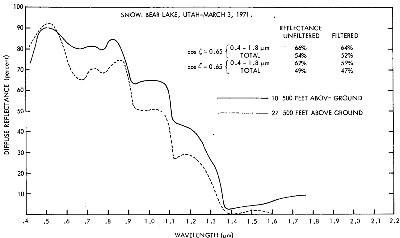
Figure 3.—Spectral reflectance of snow and cloudfree atmosphere obtained from airborne measurements at different altitudes above snow-covered Bear Lake, Utah (Hovis, 1971).
