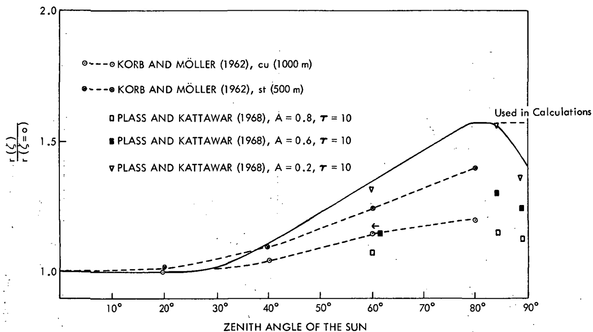
Figure B-6.—The ratio r(\xi)/r(\xi = 0) ; cloud-land model.
