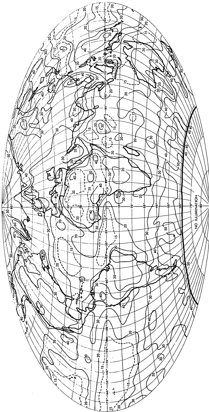
Figure 15.—Albedo (percent) of the Earth-atmosphere system during the period July 16 to 31, 1969. Values are daily averages.
