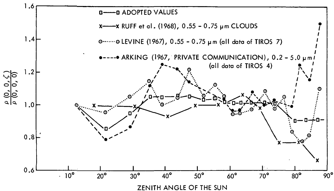
Figure B-1.—The function F_1(\xi) = \rho(0, 0, \xi)/\rho(0, 0, 0) versus the Sun's zenith angle.
