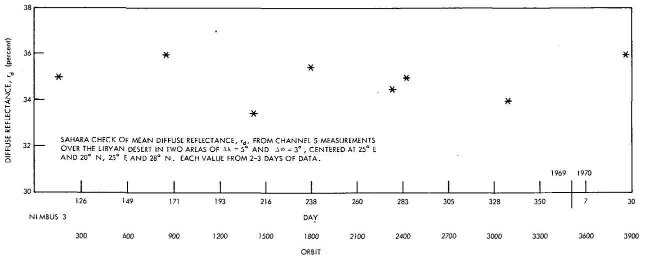
Figure 4.—Trend of reflectance over the Sahara Desert.
